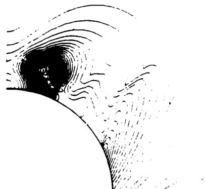
Fig. 4 Isobars on the 5 deg circular cone ( M_\infty = 4.25 , \alpha = 12.35 deg) separation forced at \theta = 115 deg.
