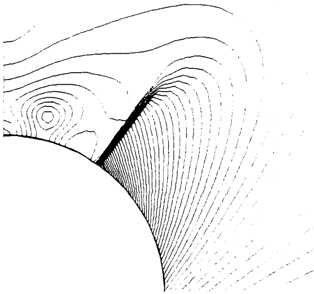
Fig. 6 Isobars on the 5° Circular Cone ( M_\infty = 4.25 , \alpha = 12.35^\circ ) Separation Due to Shock Vorticity Alone at \theta = 151.3^\circ
