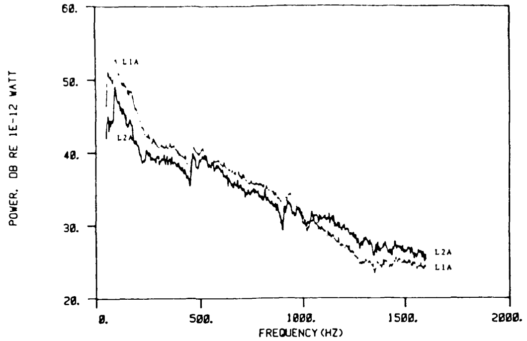
Figure 5.33: Louver geometry effect on sound power spectral level, L1A versus L2A at U = 30 m/s.
