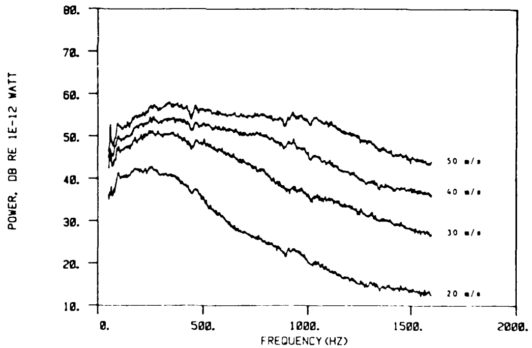
Figure 5.11(b): Orifice 03 sound power spectral levels versus freestream velocity
