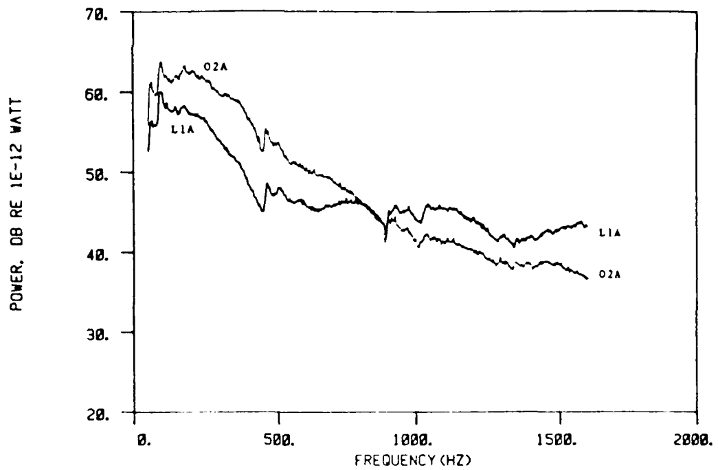
Figure 5.32: Effect of louvering on sound power spectral level, L1A versus O2A at U = 50 m/s.
