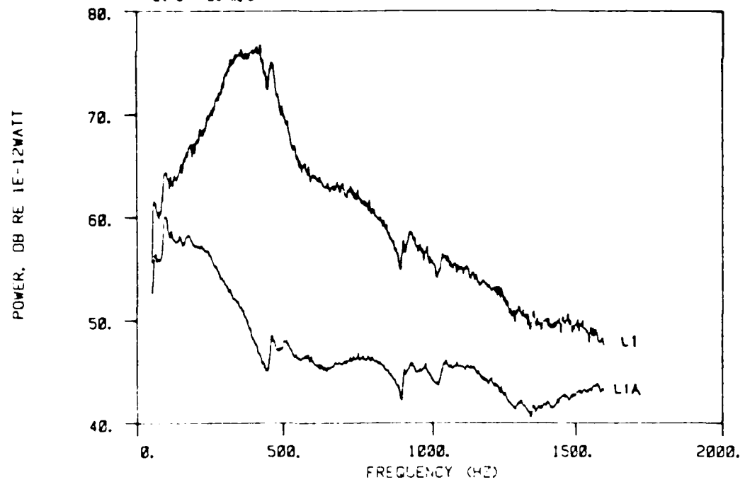
Figure 5.25: Edge angle effect on power spectral level, L1 versus L1A at U = 50 m/s
