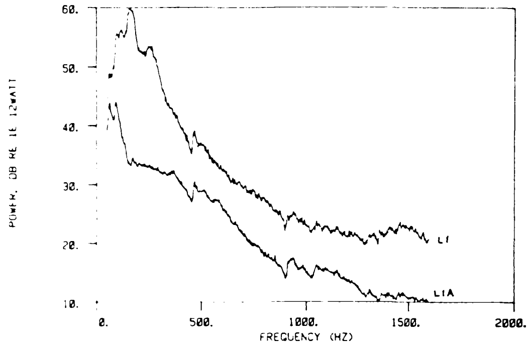
Figure 5.24: Edge angle effect on sound power spectral level, L1 versus L1A at U = 20 m/s
