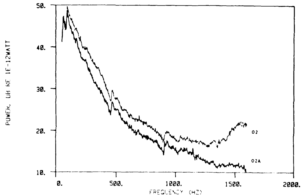
Figure 5.28: Edge angle effect on sound power spectral level, 02 versus 02A at U = 20 m/s.
