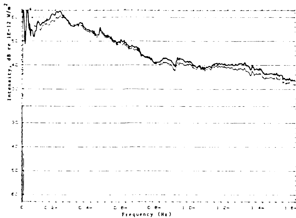
Figure 5.2: Sound field reactivity for orifice 02A. Shown are the sound intensity and sound pressure spectral levels. The difference between the two is defined as the sound field reactivity.
