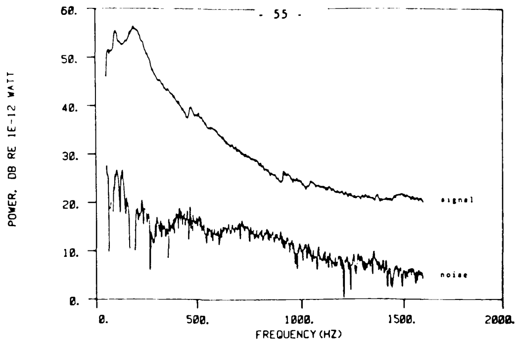
Figure 5.7 Signal to noise for orifice 01 at U = 30 m/s.
