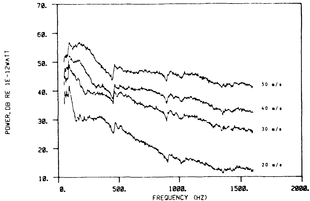
Figure 5.23: Lower L2A power spectral levels versus freestream velocity.
