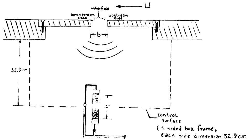
Figure 5.1: Schematic of orifice and probe geometry. Air flows at freestream velocity, U , over an aperture of streamwise dimension, b . Sound intensity is measured by probe (microphone spacing, \Delta r ) while continuously sweeping control surface.
