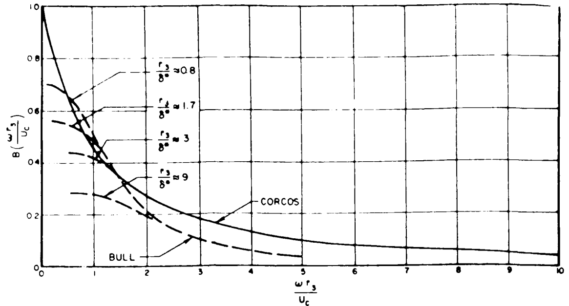
Figure 3.4: Amplitude function for lateral cross-spectral density of wall pressure From [16, BBN Report No. 4110366, 1966]
