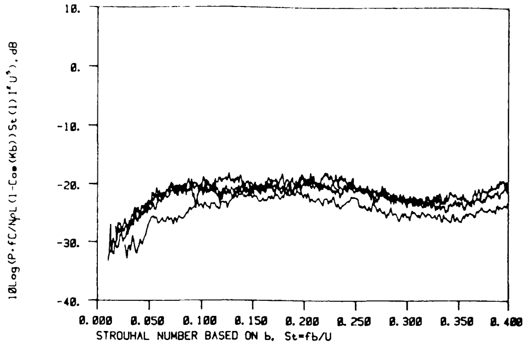
Figure 5.37: Scaling law verification for orifice 03
