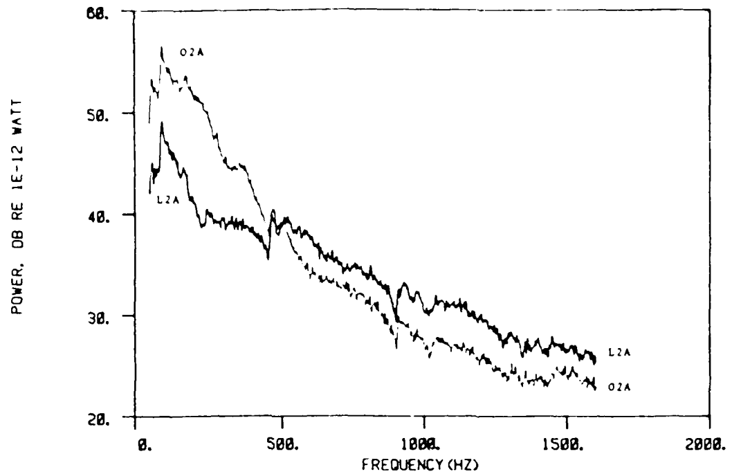
Figure 5.29: Effect of Louvering on sound power spectra level, L2A versus O2A at U = 30 m/s
