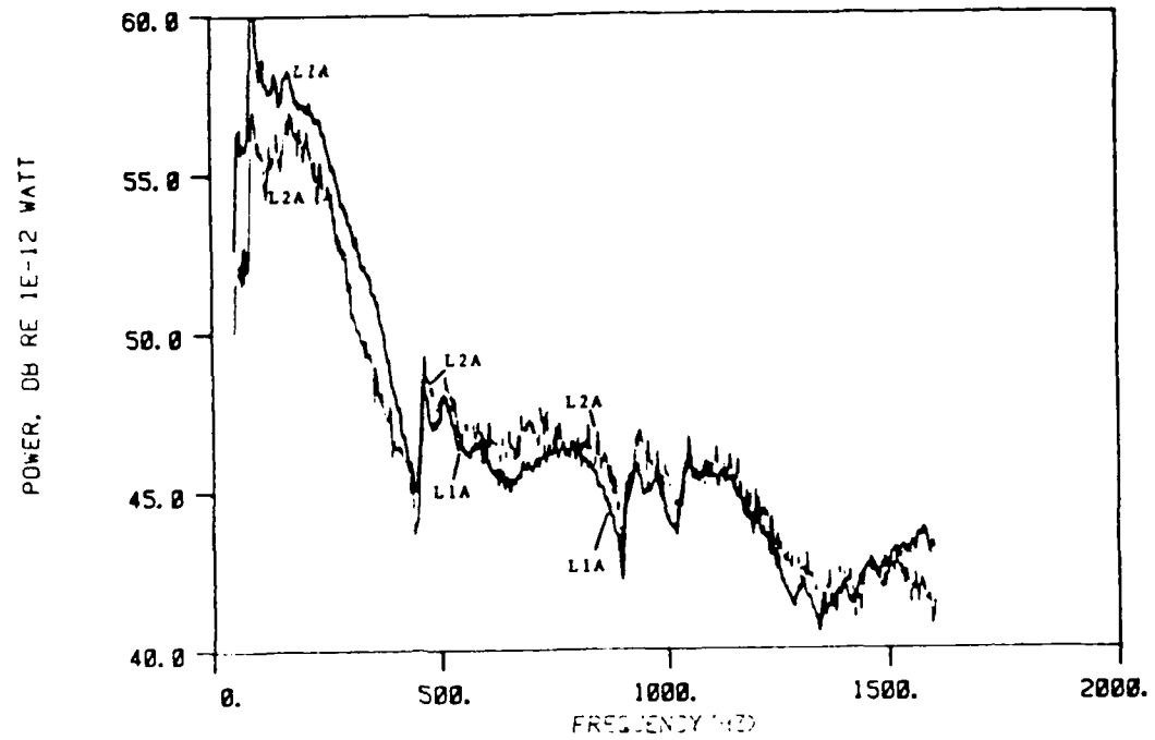
Figure 5.34: Louver geometry effect on sound power spectral level, L1A versus L2A at U = 50 m/s.
