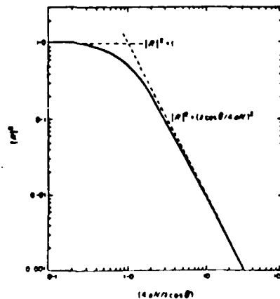
Figure 3.2: The infinite screen reflection coefficient as a function of the ratio (4aN/k\cos\theta) . From [9, Nelson, P.A., 1982].
