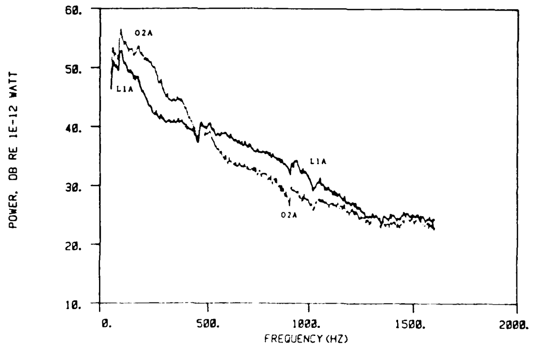
Figure 5.30: Effect of louvering on sound power spectral level, L1A versus O2A at U = 30 m/s
