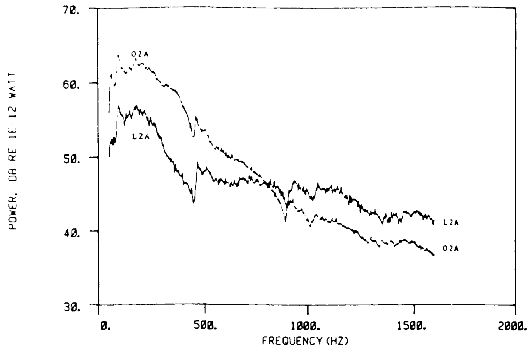
Figure 5.31: Effect of louvering on sound power spectral level, L2A versus O2A at U = 50 m/s
