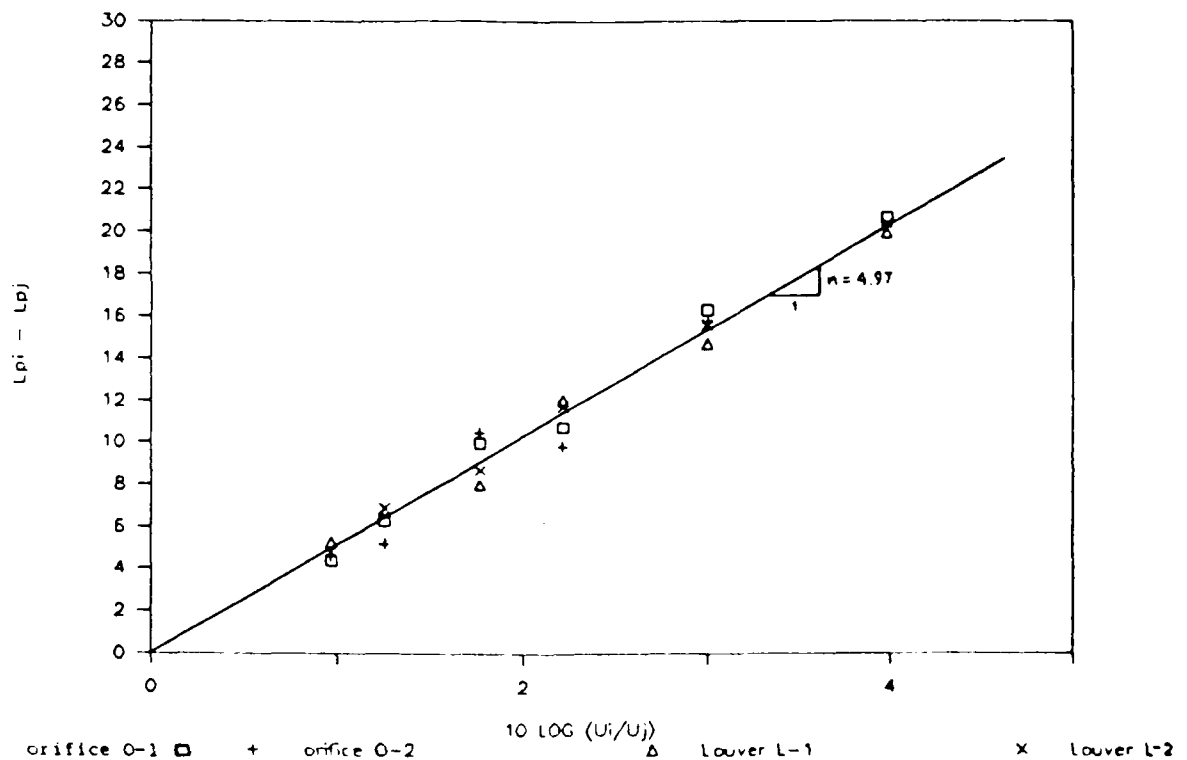
Figure 5.18: Speed/Power relationship for four samples ( P \propto CU^n ) with least squares fit
