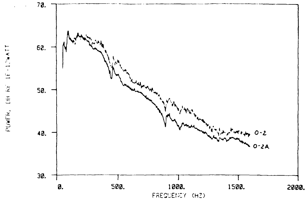
Figure 5.27: Edge angle effect on sound power spectral level, 02 versus 02A at U = 50 m/s.
