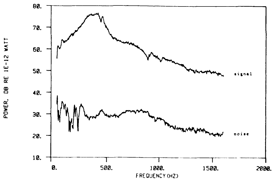
Figure 5.9: Signal to noise for orifice 03 at U = 20 m/s.
