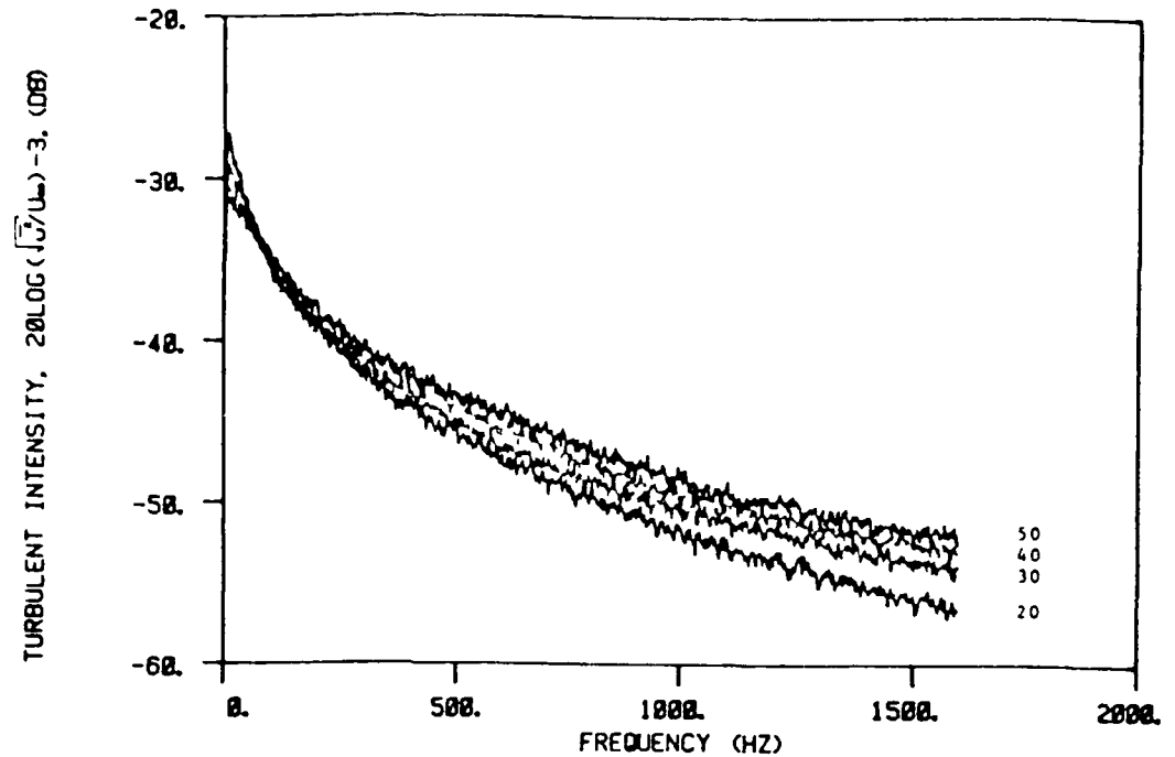
Figure 5.35: Turbulent intensity spectral levels for lower L1 versus freestream velocity.
