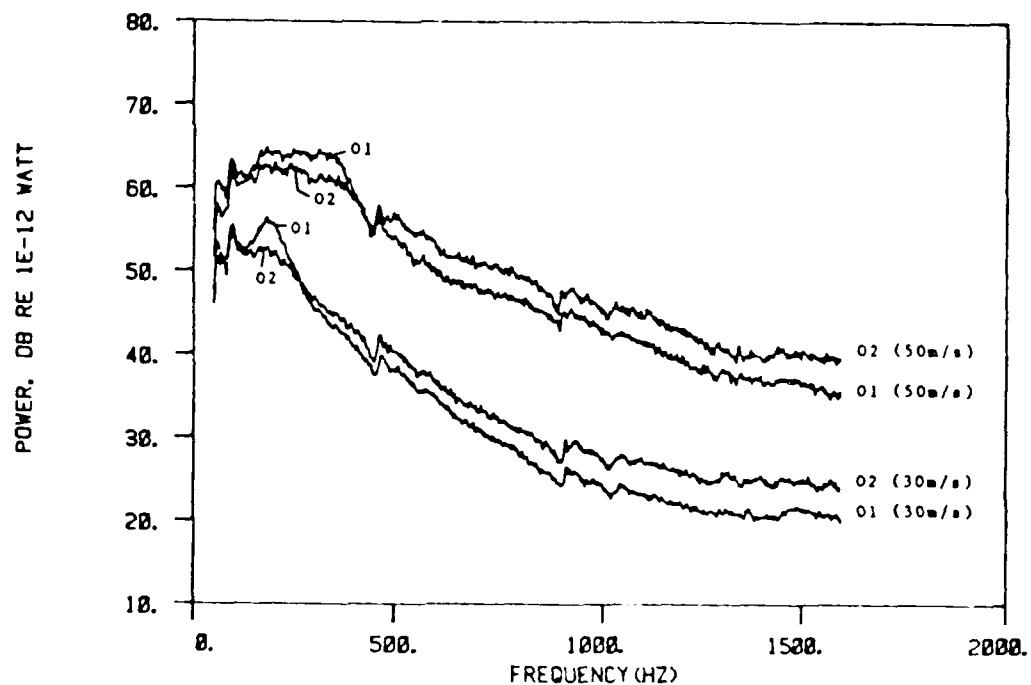
Figure 5.17: Orifice depth effect on sound power, 01 versus 02 at U = 30 and 50 m/s
