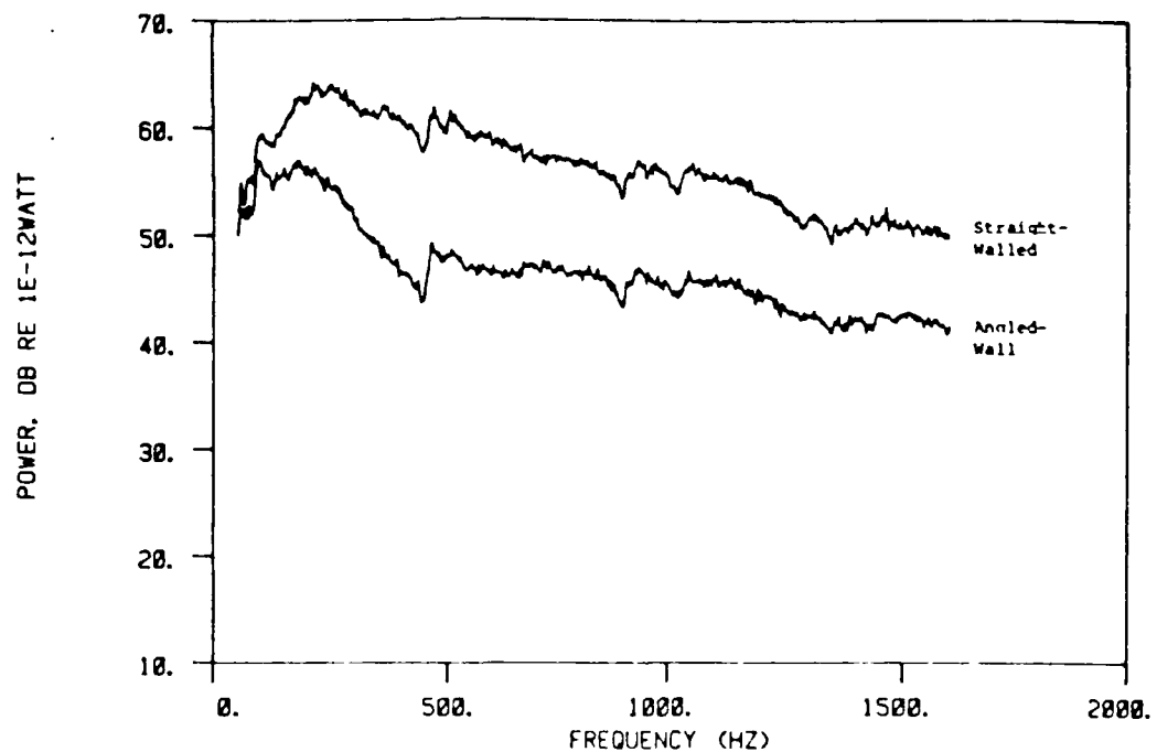
Figure 5.26: Edge angle effect on sound power spectral level, L2 versus L2A at U = 50 m/s.
