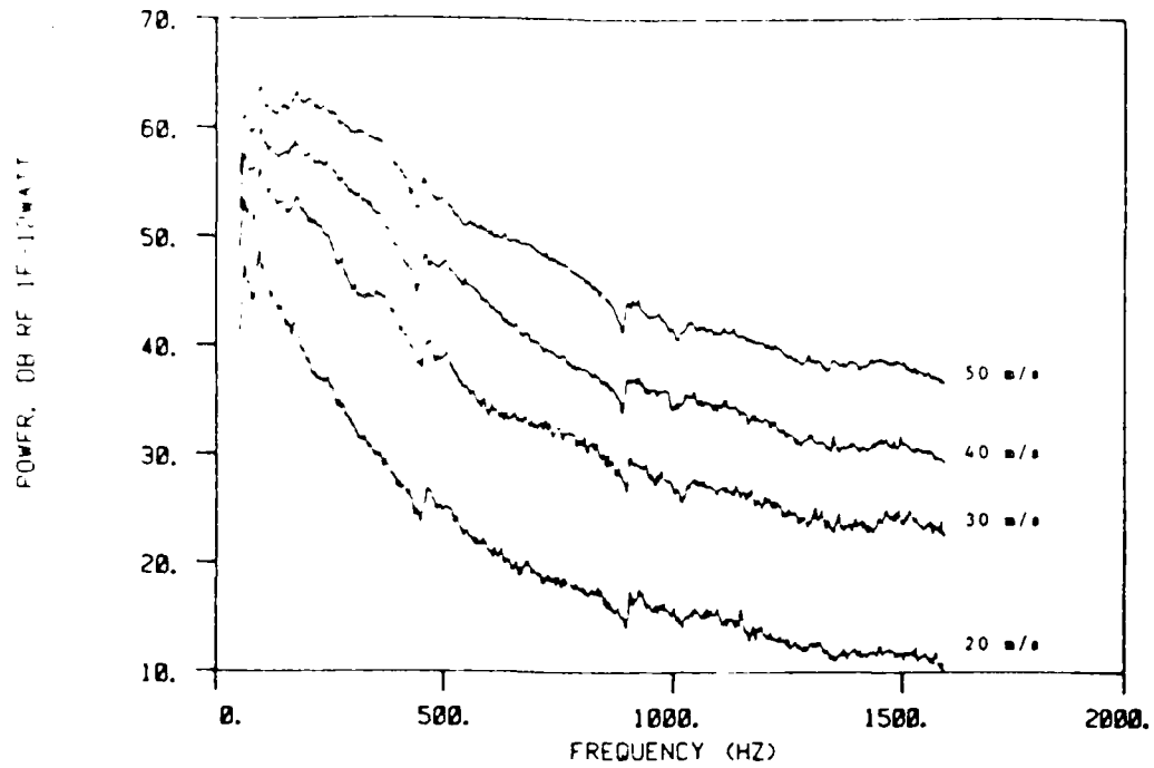
Figure 5.21: Orifice 02A power spectra level versus freestream velocity
