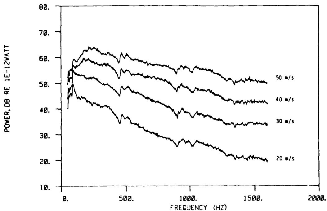
Figure 5.11(d): Louver L2 sound power spectral levels versus freestream velocity
