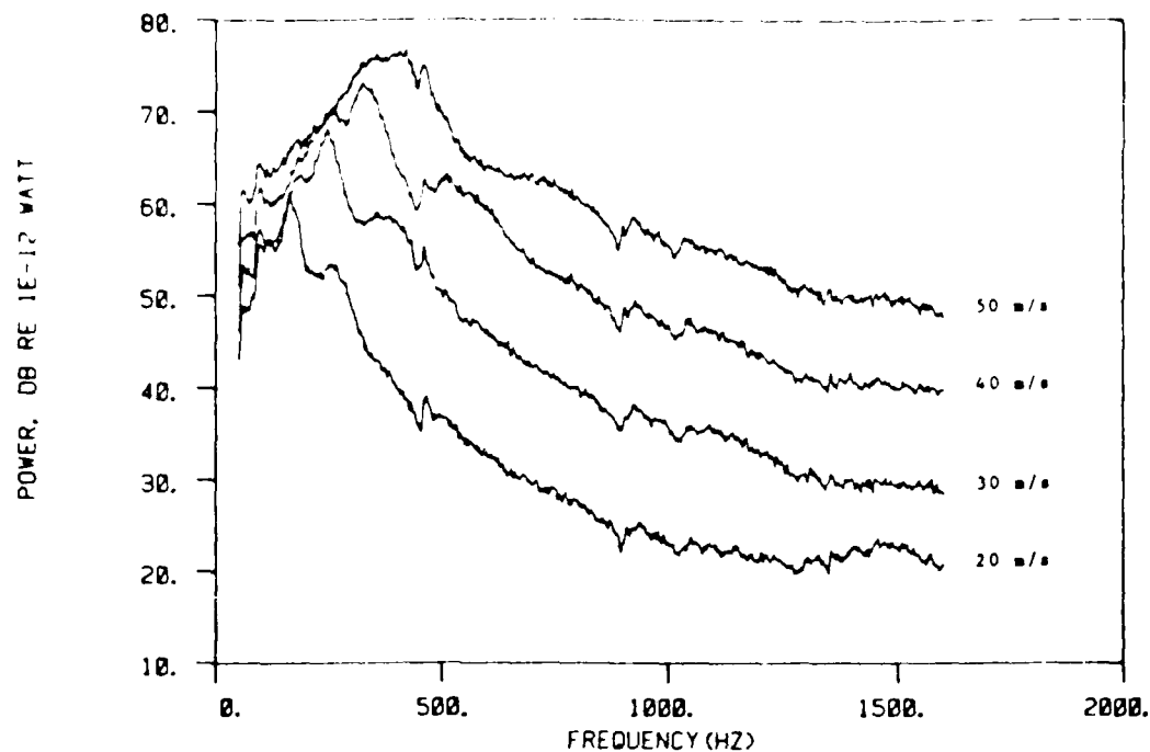
Figure 5.11(c): Louver L1 sound power spectra levels versus freestream velocity
