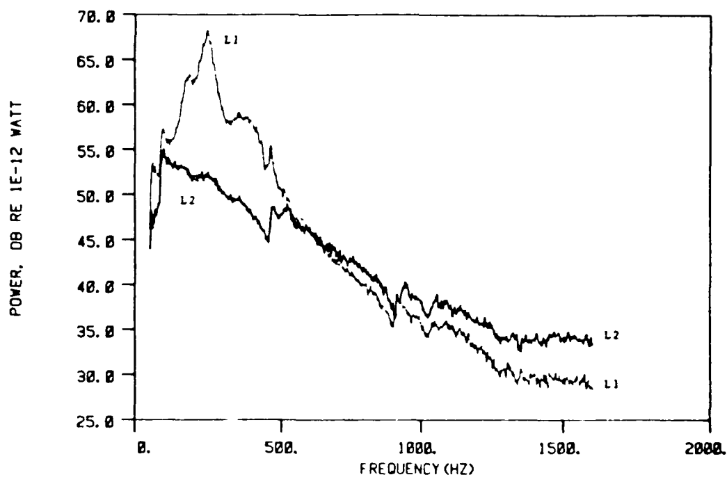
Figure 5.13: Louver geometry effect on sound power, L1 versus L2 at U = 30\text{m/s}
