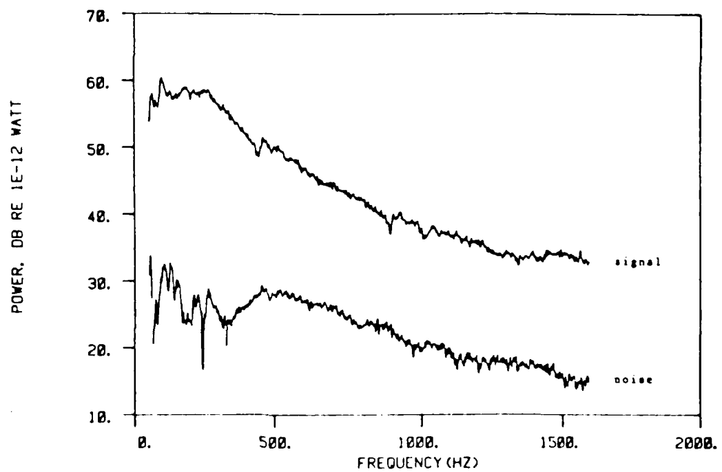
Figure 5.8: Signal to noise for orifice 02 at U = 40 m/s.
