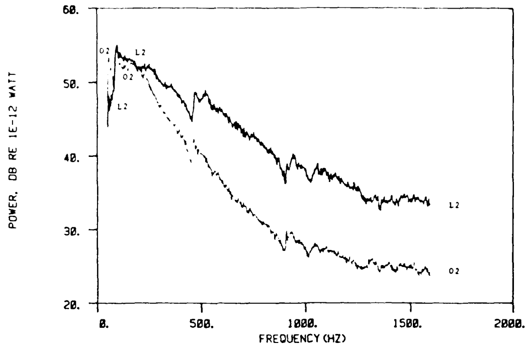
Figure 5.15: Effect of louvering on sound power, L2 versus O2 at U = 30 \text{ m/s}
