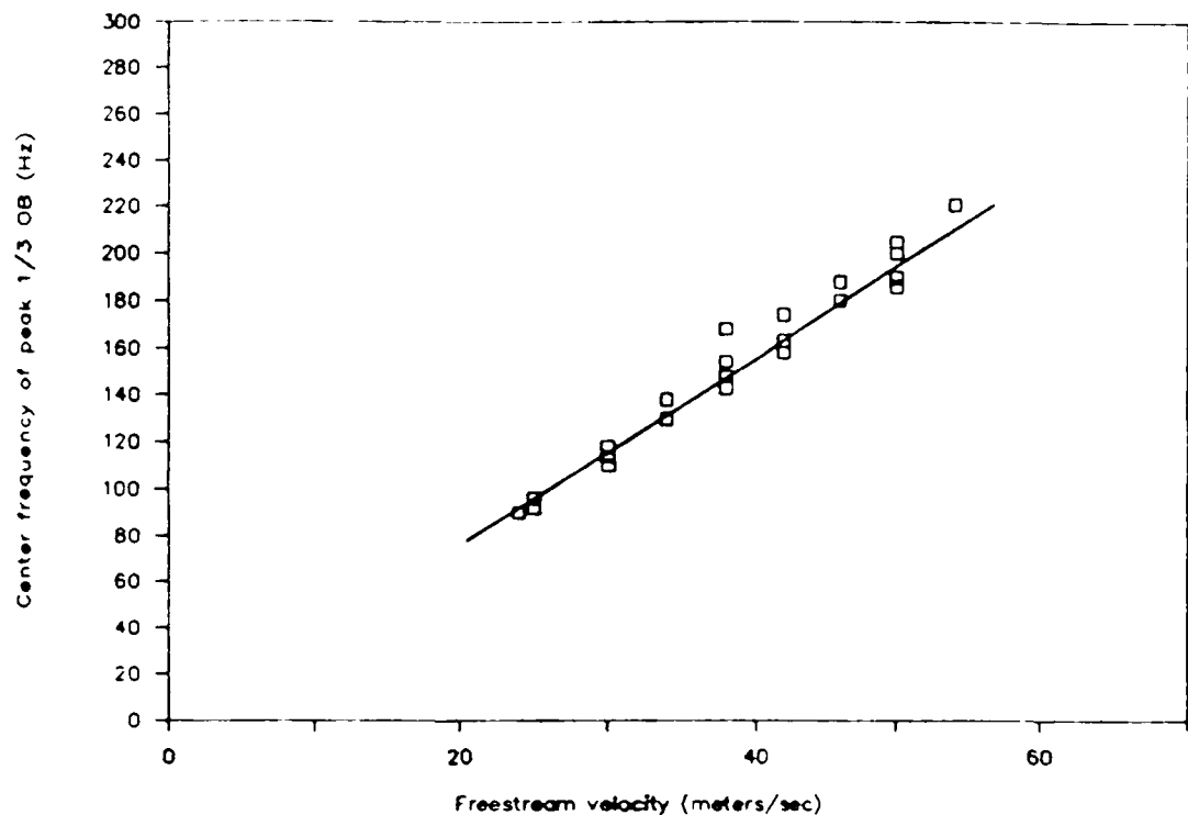
Figure 5.4: Frequency/velocity relationship for orifice 01. Shown are four separate experiments for various radial distances, r .
