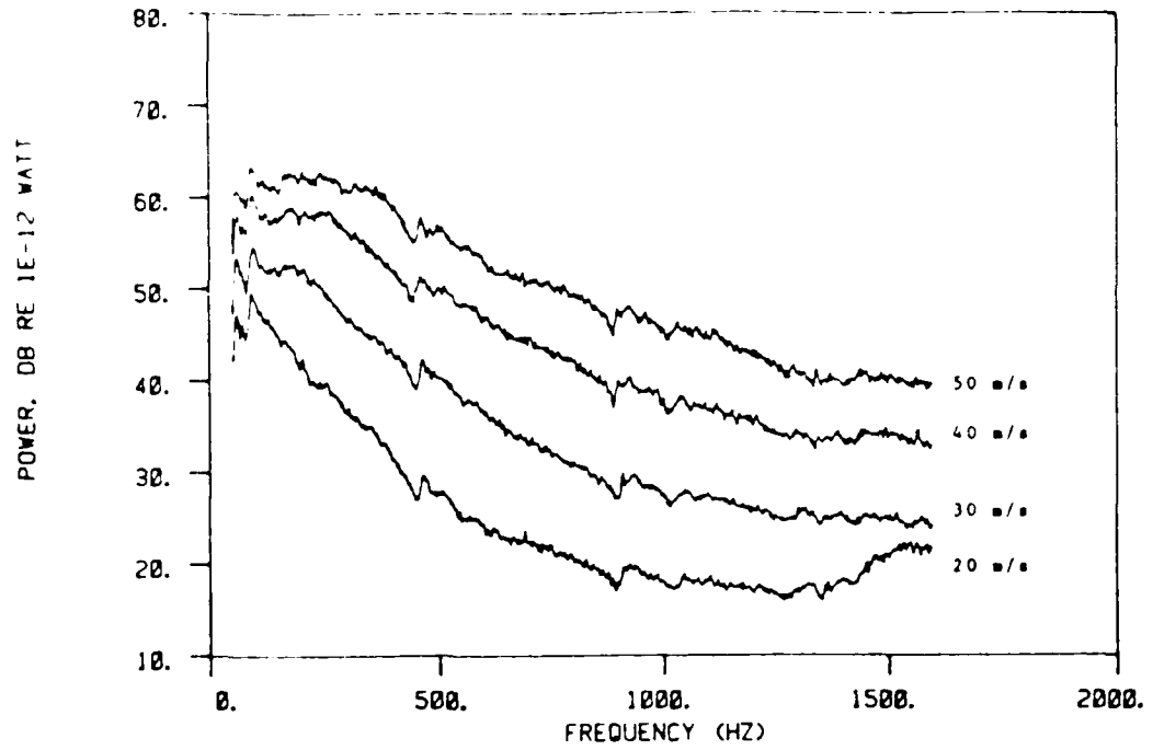
Figure 5.11(a): Orifice 02 sound power spectral levels versus freestream velocity
