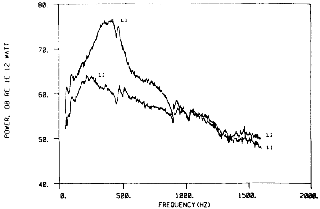
Figure 5.14: Louver geometry effect on sound power, L1 versus L2 at U = 50\text{m/s}
