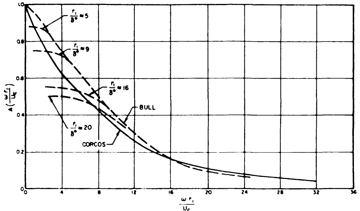
Figure 3.3: Amplitude function for longitudinal cross-spectral density of wall pressure. From [16, BBN report No. 4110366, 1966]
