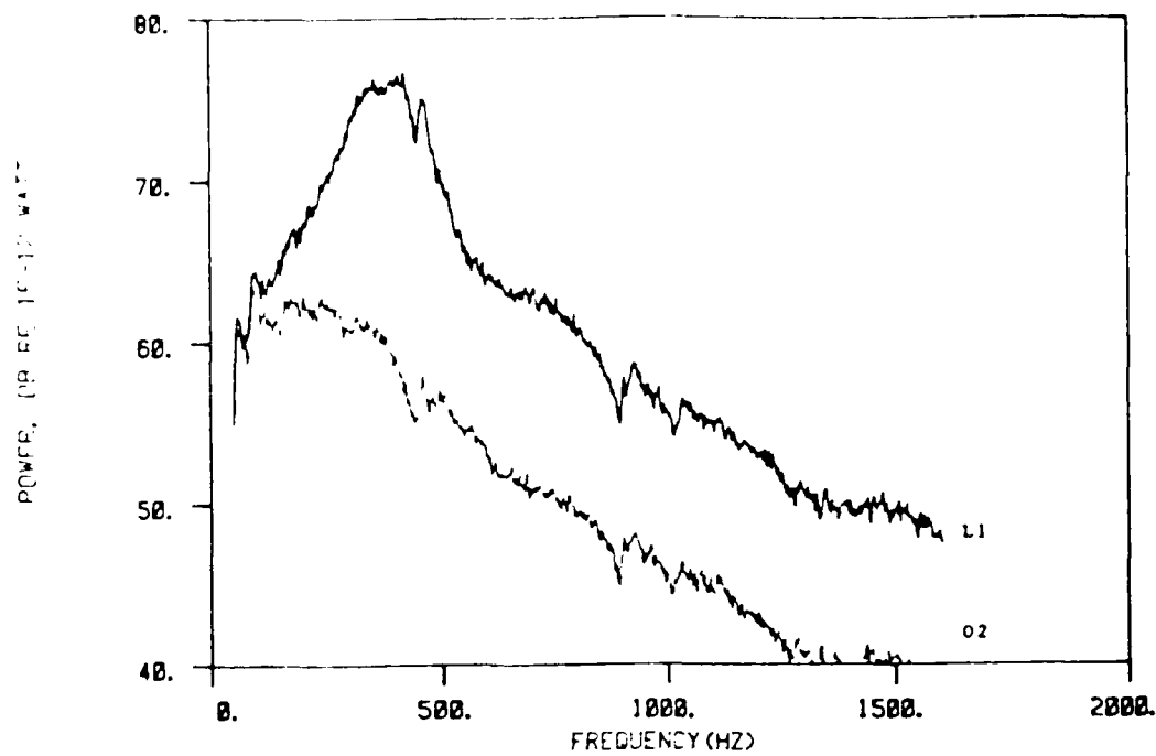
Figure 5.12a: The effect of louvering on sound power, L1 versus L2 at U=50\text{m/s}
