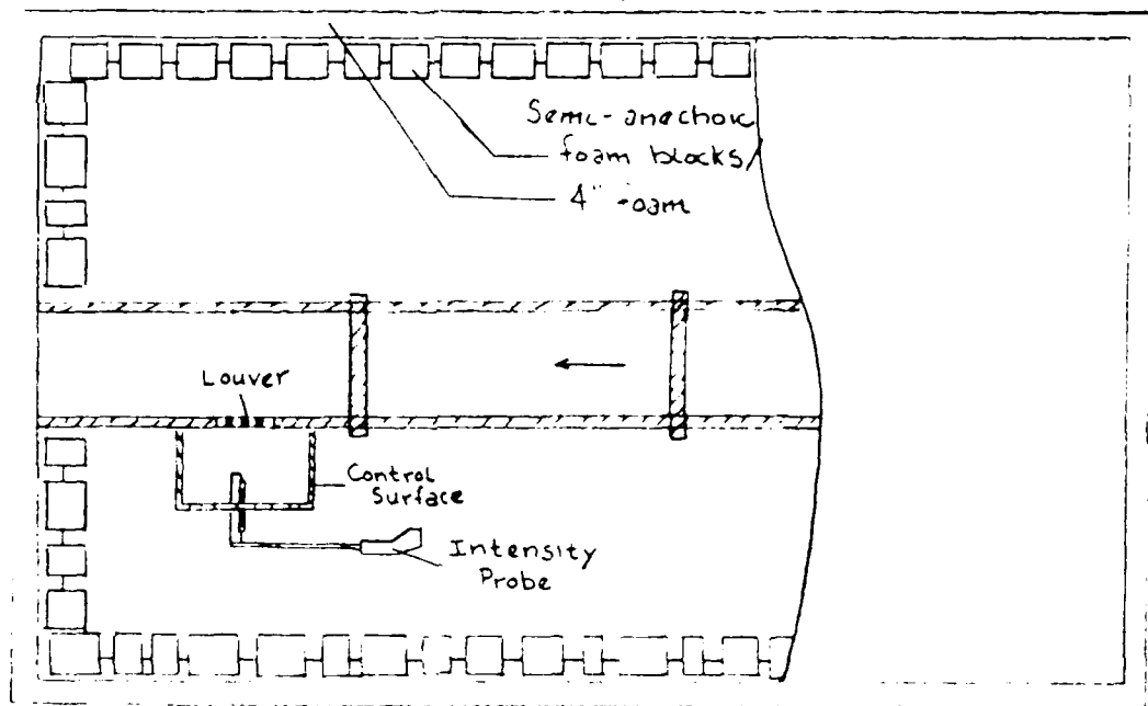
Figure 4.2: Experimental set-up within the wind tunnel, front and top views
