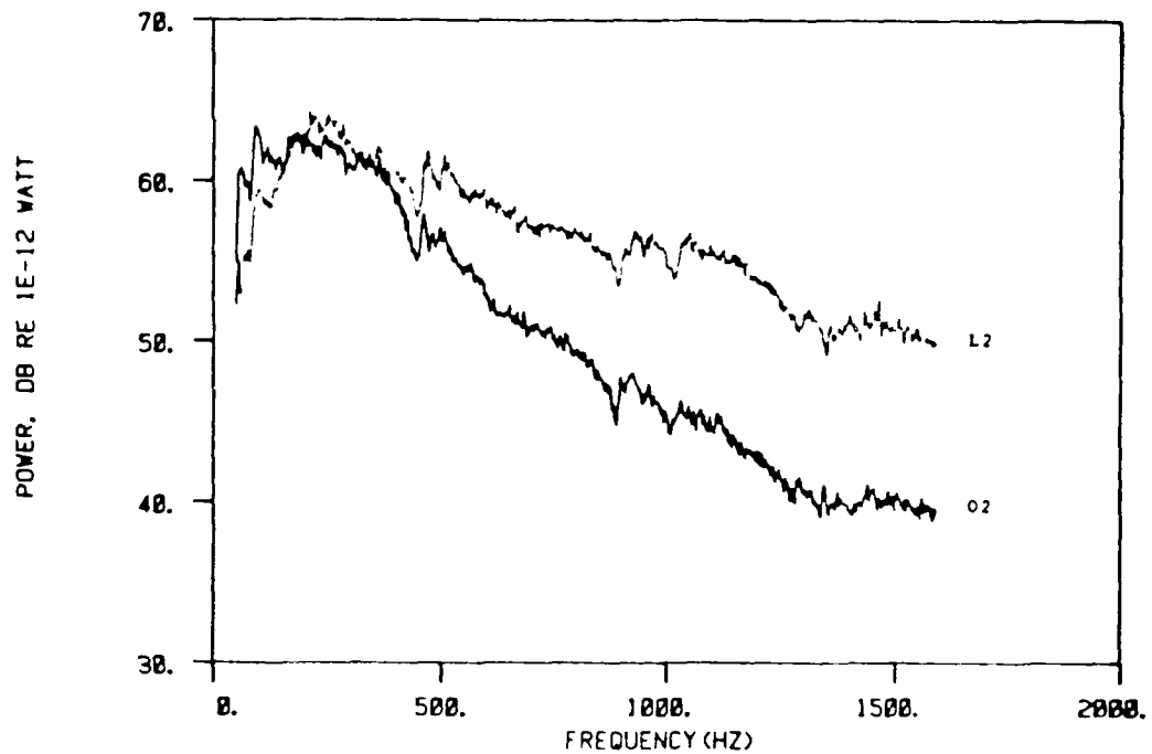
Figure 5.16: Effect of louvering on sound power, L2 versus O2 at U = 50 \text{ m/s}
