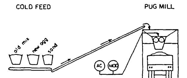
b. Standard Batch Plant Used To Produce Cold Recycled Mix
