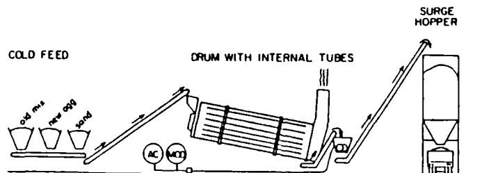
d. Indirect Heating Method
