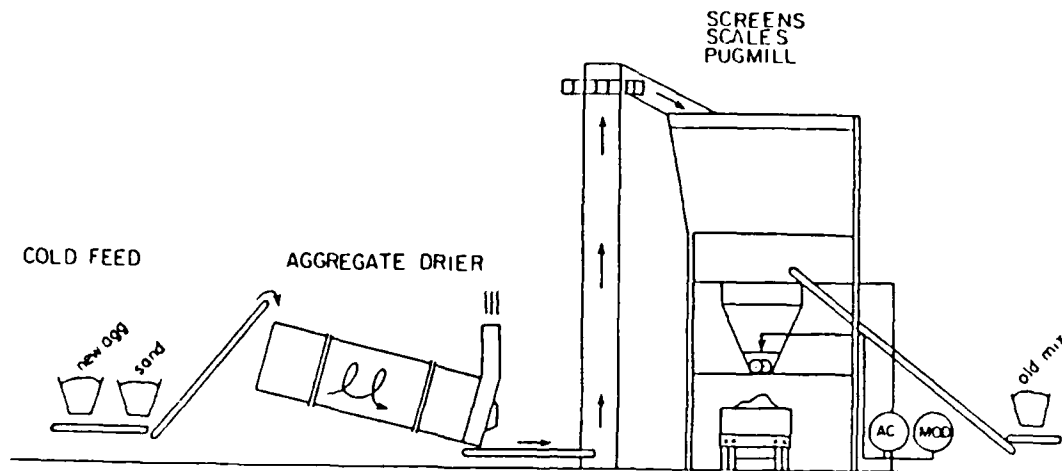
a. Old Mix Added At Pug Mill
