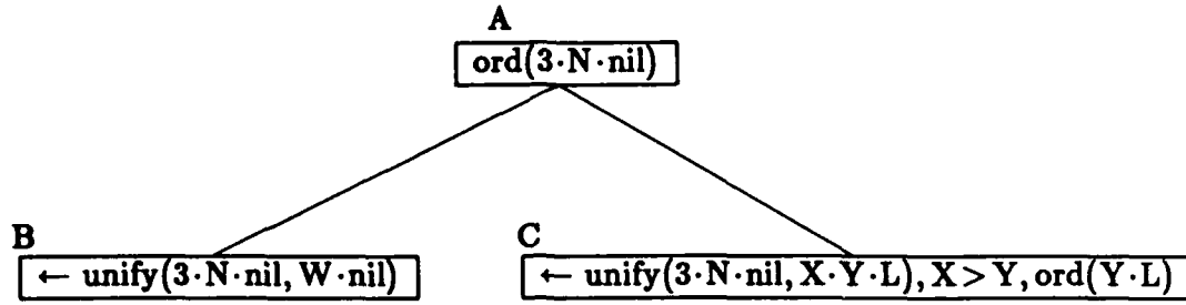
Figure 5.1: Overlap reduction
