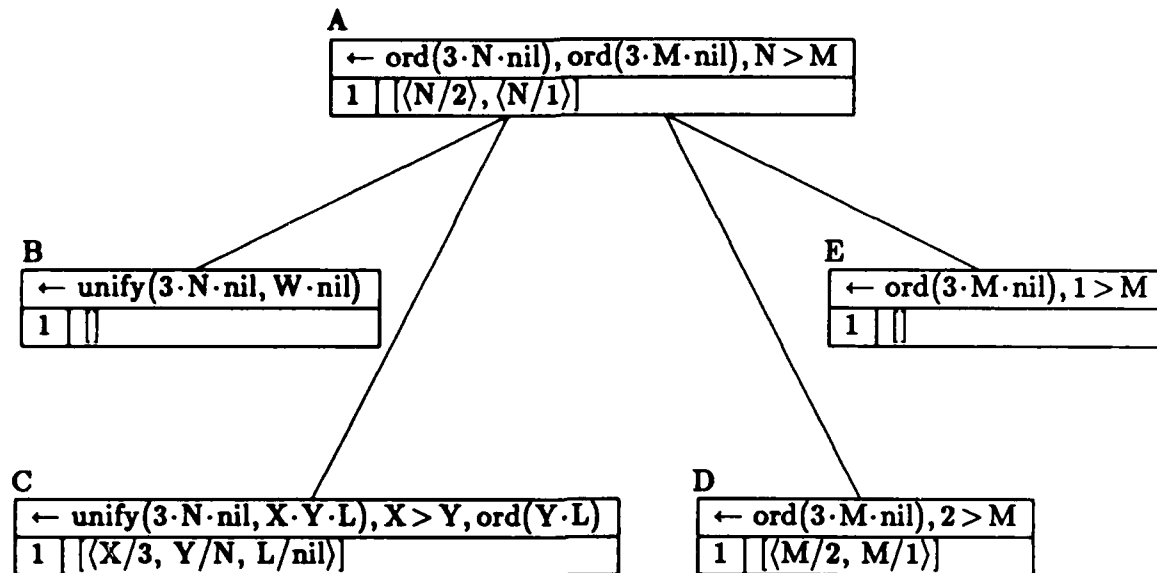
Figure 5.3: Upper two levels of an ESL tree
