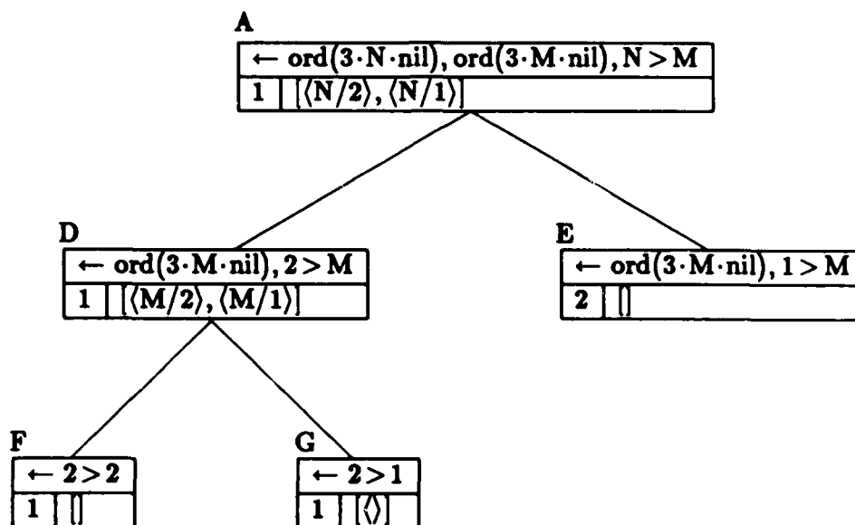
Figure 5.2: Selection reduction
