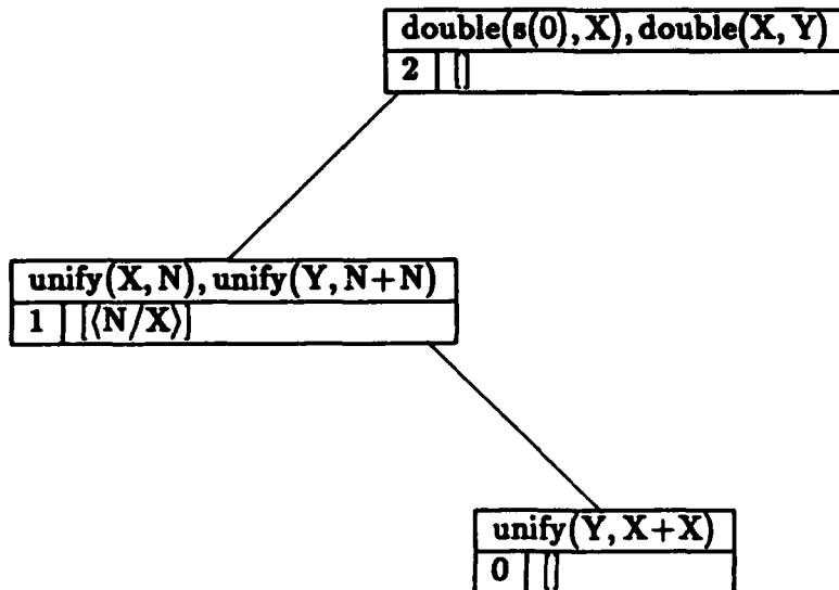
Figure 5.8: Blocked M-ESL tree
