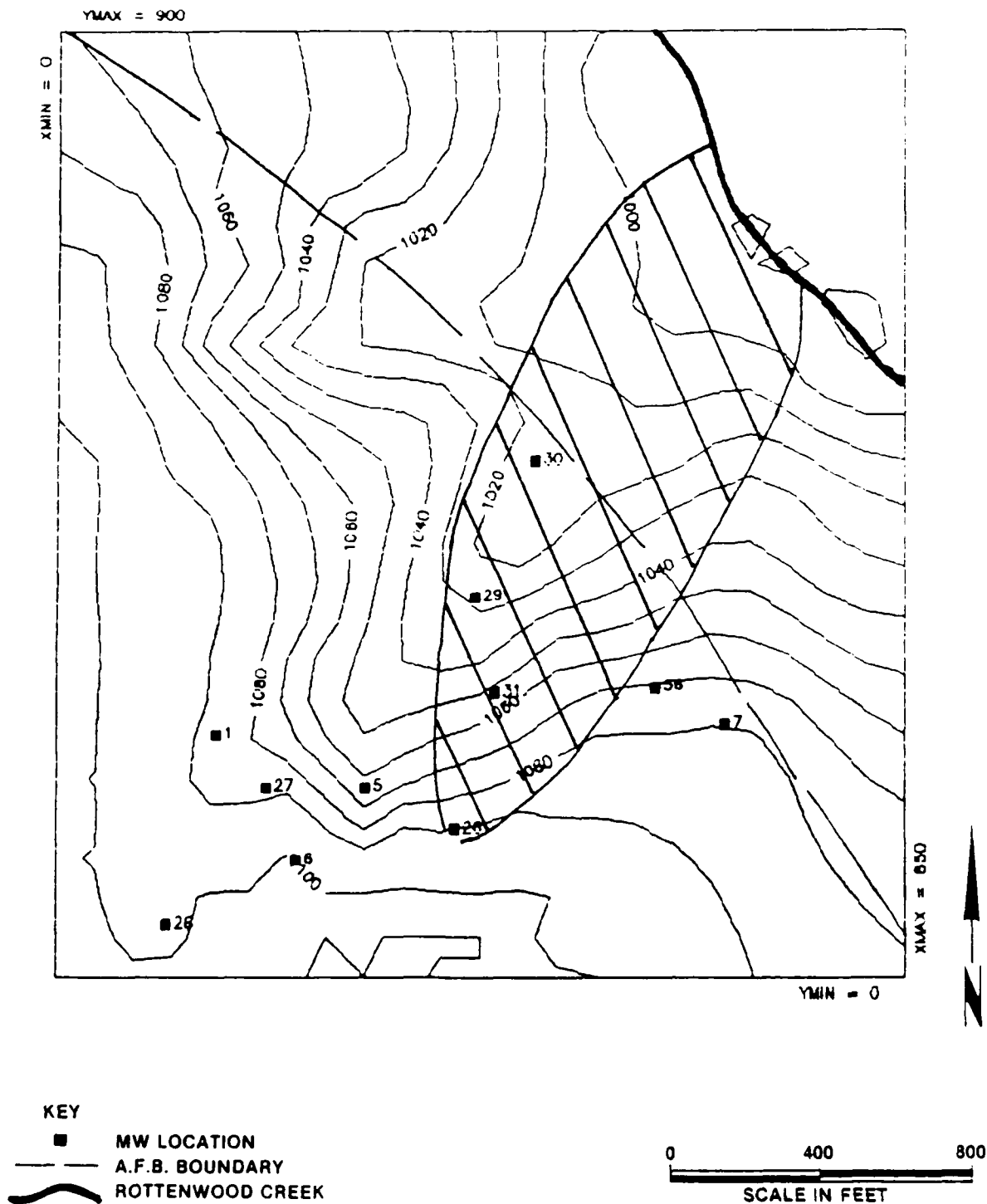
Figure 4.3-34 METHYLENE CHLORIDE PLUME—730-DAY RANDOM WALK PROJECTION FOR MAY 1986 IMPOSED ON SURFACE ELEVATIONS (FT), ZONE 2—INDUSTRIAL FACILITIES, ACTIVE LANDFILL, AND STORMWATER RETENTION BASIN NO. 2
