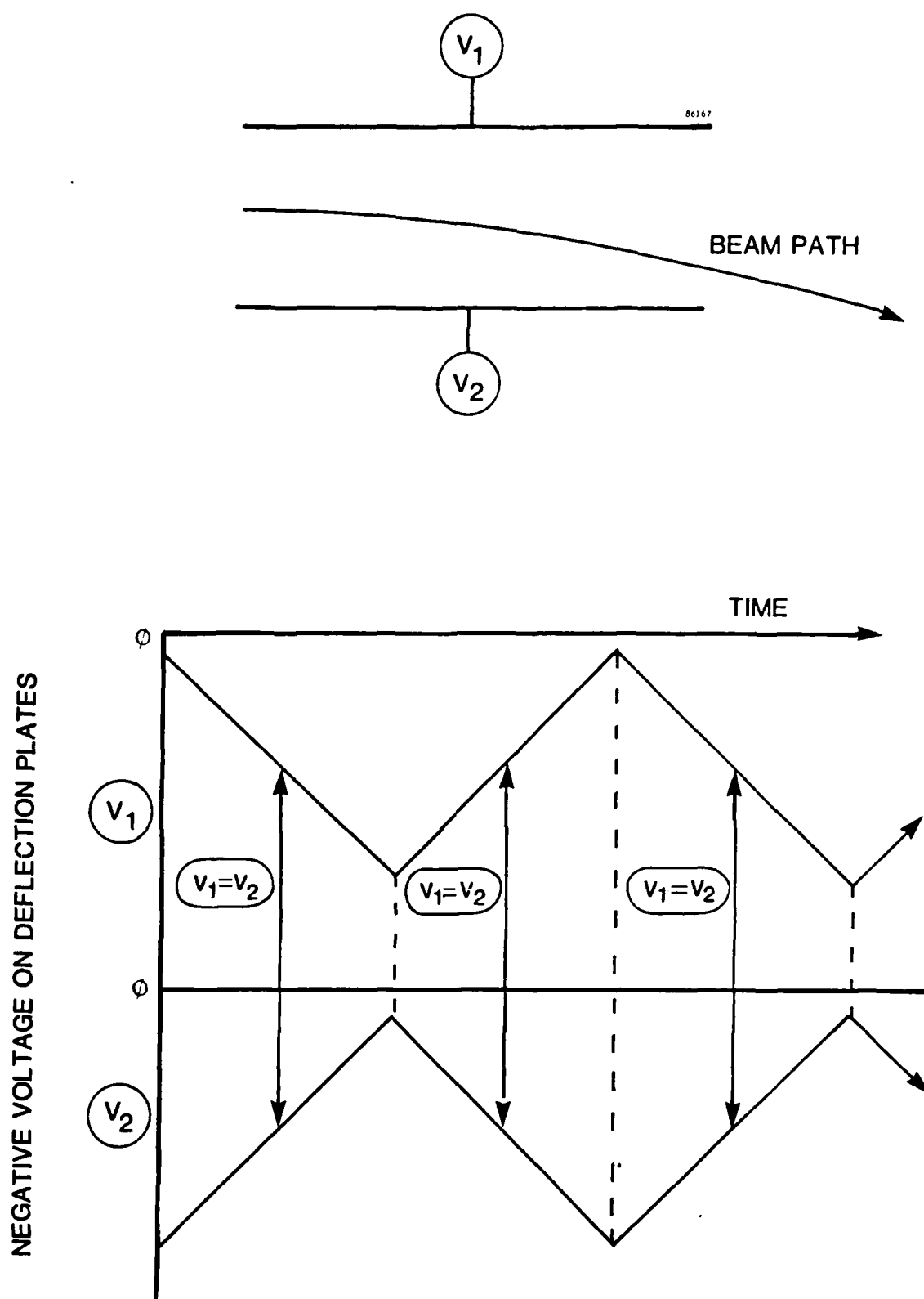
FIGURE 3-9. ORIGINAL DEFLECTION PLATE GEOMETRY.
