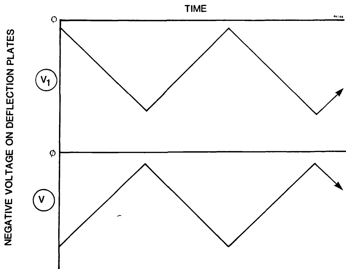
FIGURE 3-10. MODIFIED DEFLECTION PLATE GEOMETRY.
