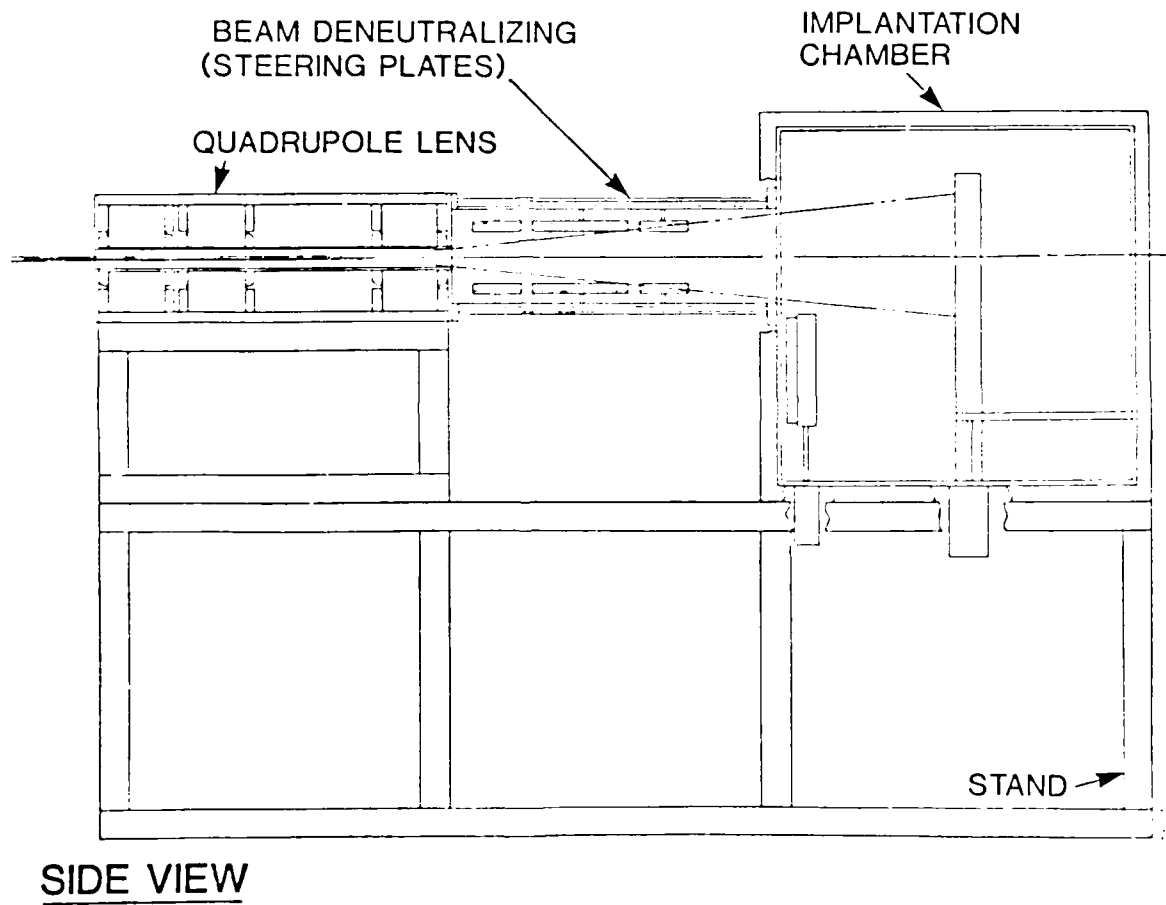
FIGURE 3-11. SUPPORT STRUCTURE FOR THE END STATION.
