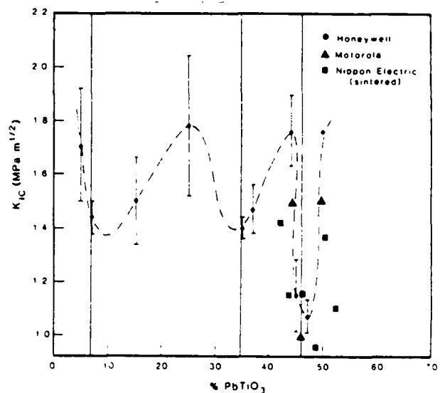
Figure 5. Critical fracture toughness, K_{IC} , of PZT as a function of the PbTiO_3 in the material. The vertical lines represent the positions of the phase boundaries (after Freiman et al [11]).
