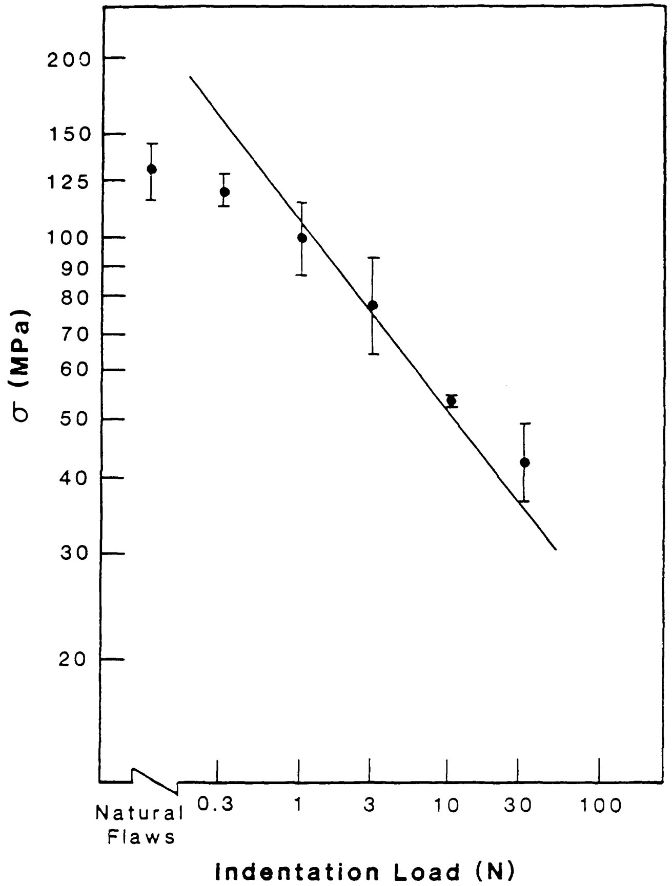
Figure 7 Fracture stress-indentation load plot for XLS02 (Dupont) ceramic.
