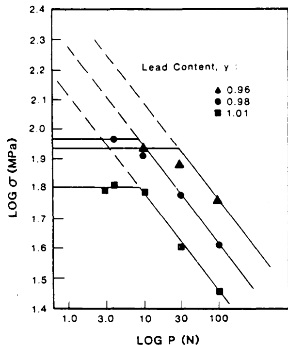
Figure 6. Indentation-fracture data for a 95/5 PZT ceramic [Pb_yNb_{0.02}(Zr_{0.95}Ti_{1.04})_{0.98}O_3] in which y varied from 0.96 to 1.01. Positions of the curves of slope, -1/3 , are indicative of the K_{IC} of each material. Strength plateaus are a measure of the effect of internal stresses (after Freiman et al [11]).
