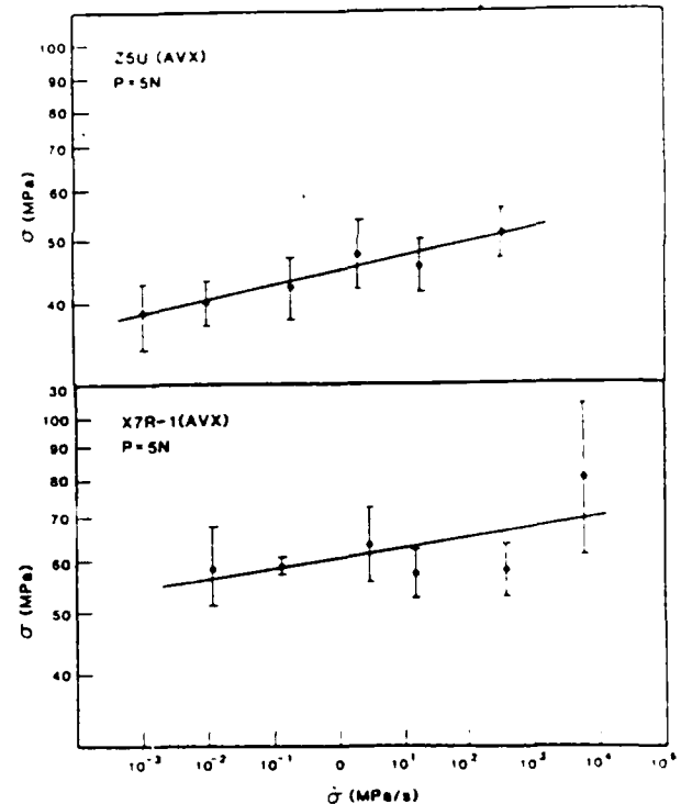
Figure 8. Stressing rate dependence of the strength of two capacitor ceramics ZSU and X7R. Data was obtained on indented squares of material in water ( \dot{\sigma} = 5 specimens/data point). Note the lack of change in strength for the lower 5 stressing rates in X7R material suggesting the existence of a crack growth limit (after Baker and Freeman [22]).
