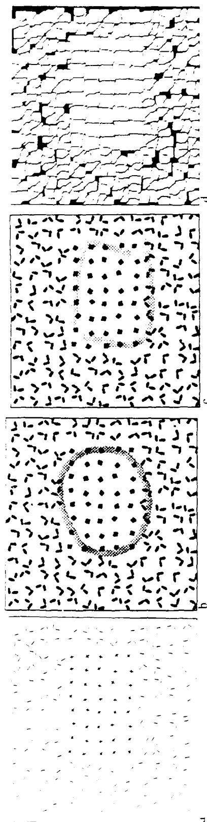
Figure 6.1 (a) A purported demonstration of crossings as textons [Julesz and Bergen 1983]. (b) However, the + 's yield wider blobs than the L segments after \nabla^2 G filtering, shown here with detected width boundaries. (c) Nearest-neighbor (center-to-center) spacing boundaries also account for perception. (d) The partial Voronoi tessellation (whose computation is described in Section 4.5.2) defines the neighbor relations.
