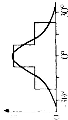
h(\theta)
