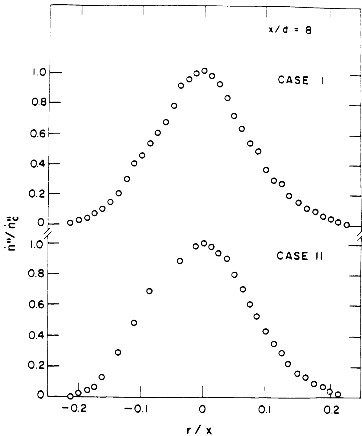
Figure 8. Mean particle number fluxes at x/d = 8 .
