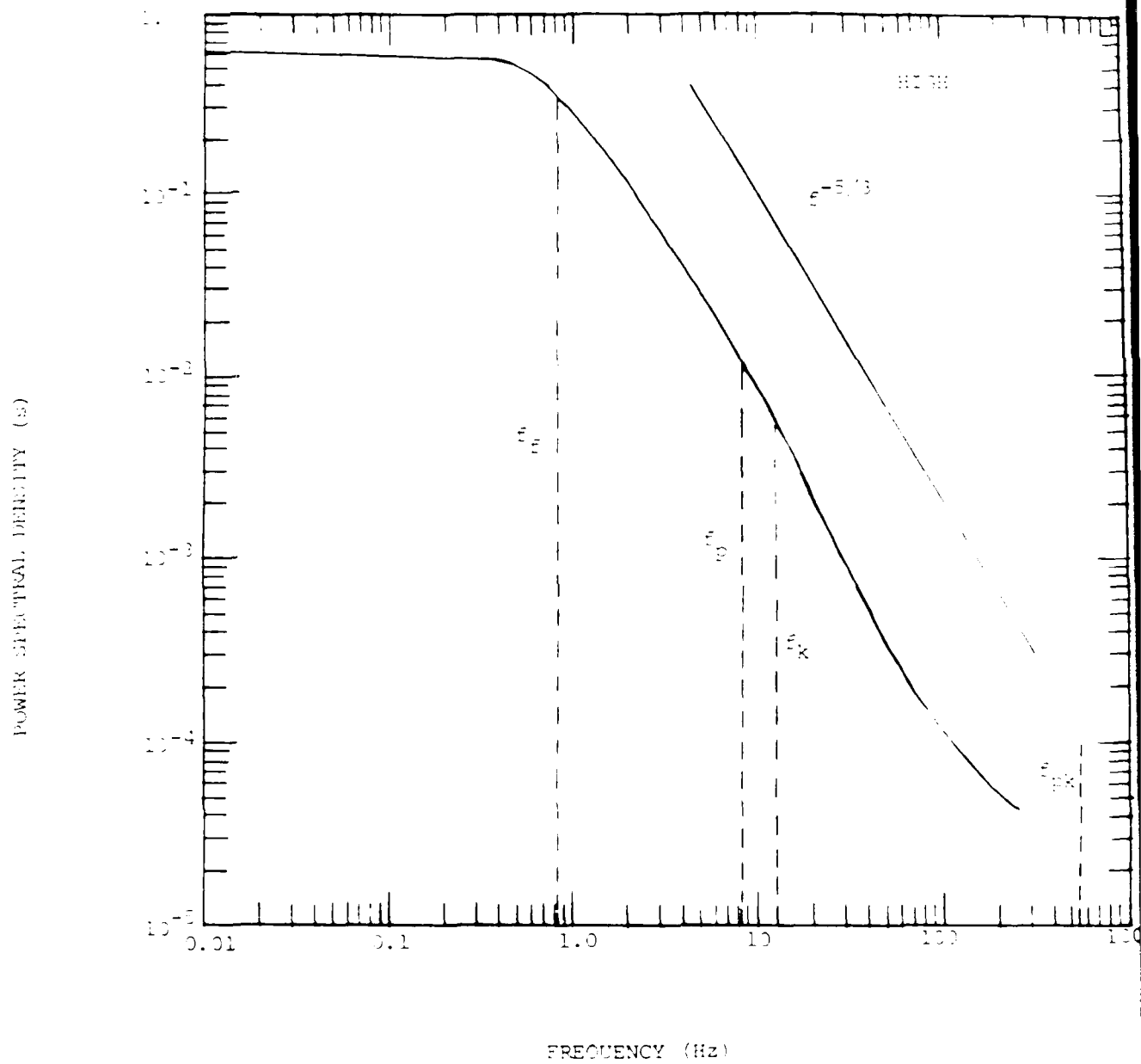
Figure 38. Power spectrum of streamwise velocities (high condition).
