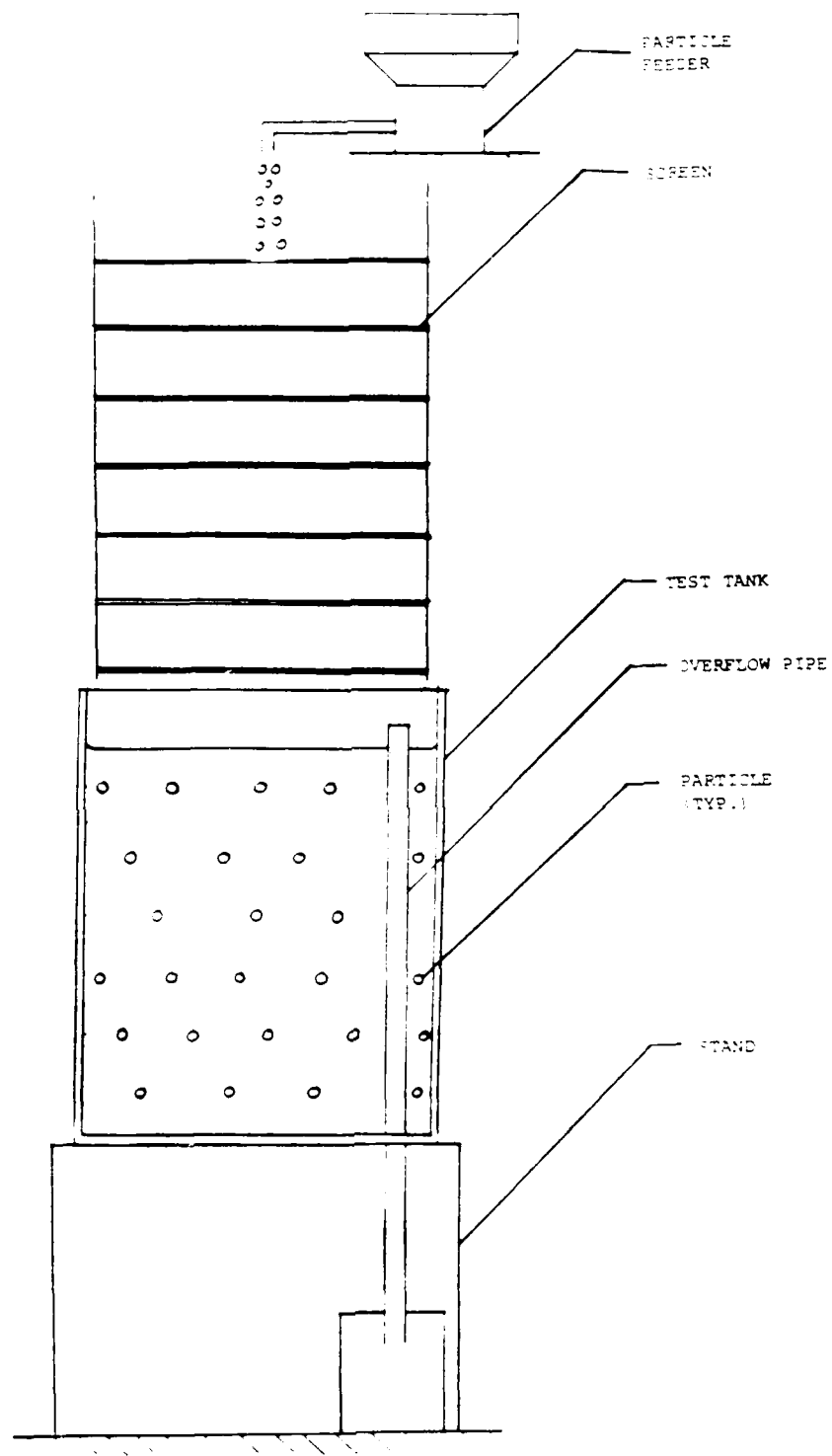
Figure 24. Sketch of the homogeneous particle flow apparatus.
