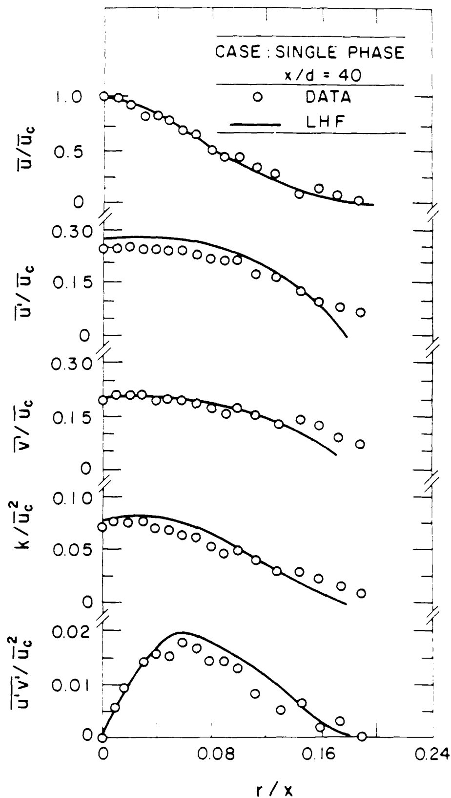
Figure 14. Mean and turbulent properties for the single-phase jet, x/d = 40 .
