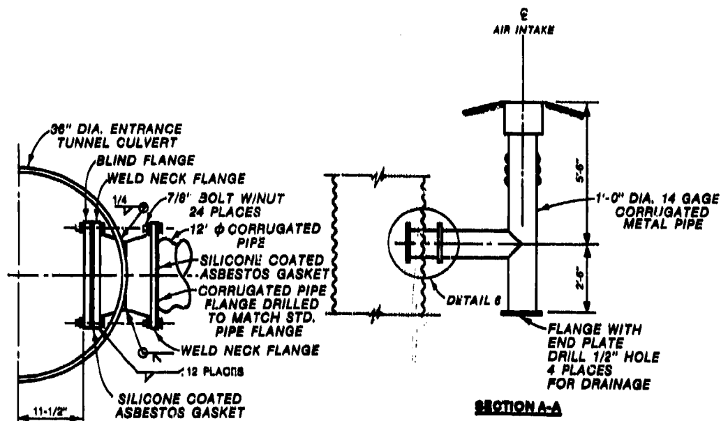
DETAIL-4
