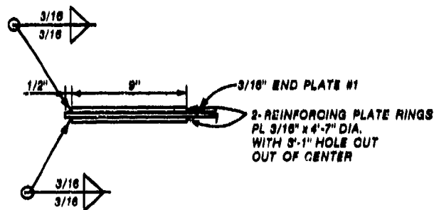
SECTION H-H
