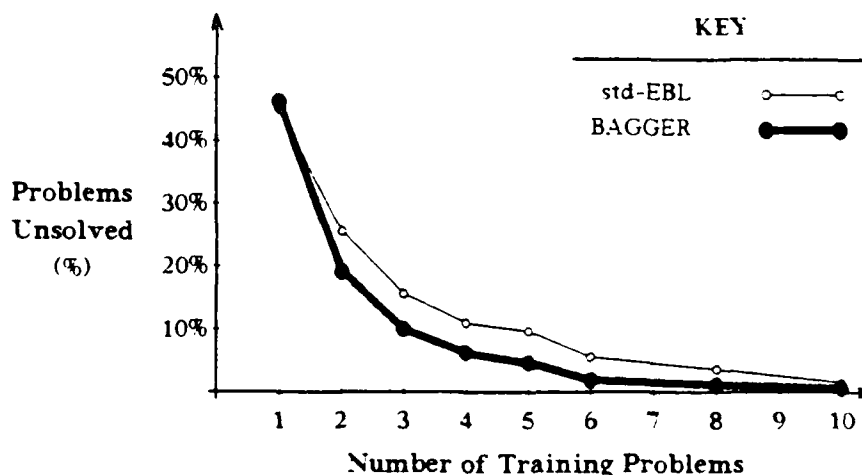
Figure 19. Failure Comparison of the Trained Problem Solvers
