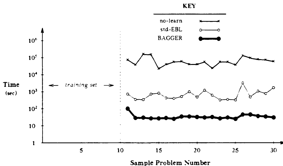
Figure 17. Performance Comparison of the Trained Problem Solvers
