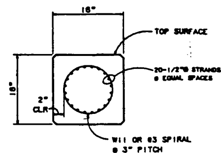
SECTION - 16" SQ PILE 1 1/2" = 1'-0" W/ 20 STRANDS CIRCULAR PATTERN
