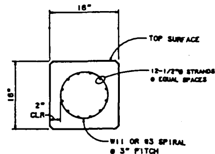
SECTION - 16" SQ PILE 1 1/2" = 1'-0" W/ 12 STRANDS CIRCULAR PATTERN
