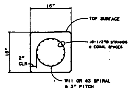
SECTION - 16" SQ PILE 1 1/2" = 1'-0" W/ 16 STRANDS CIRCULAR PATTERN
