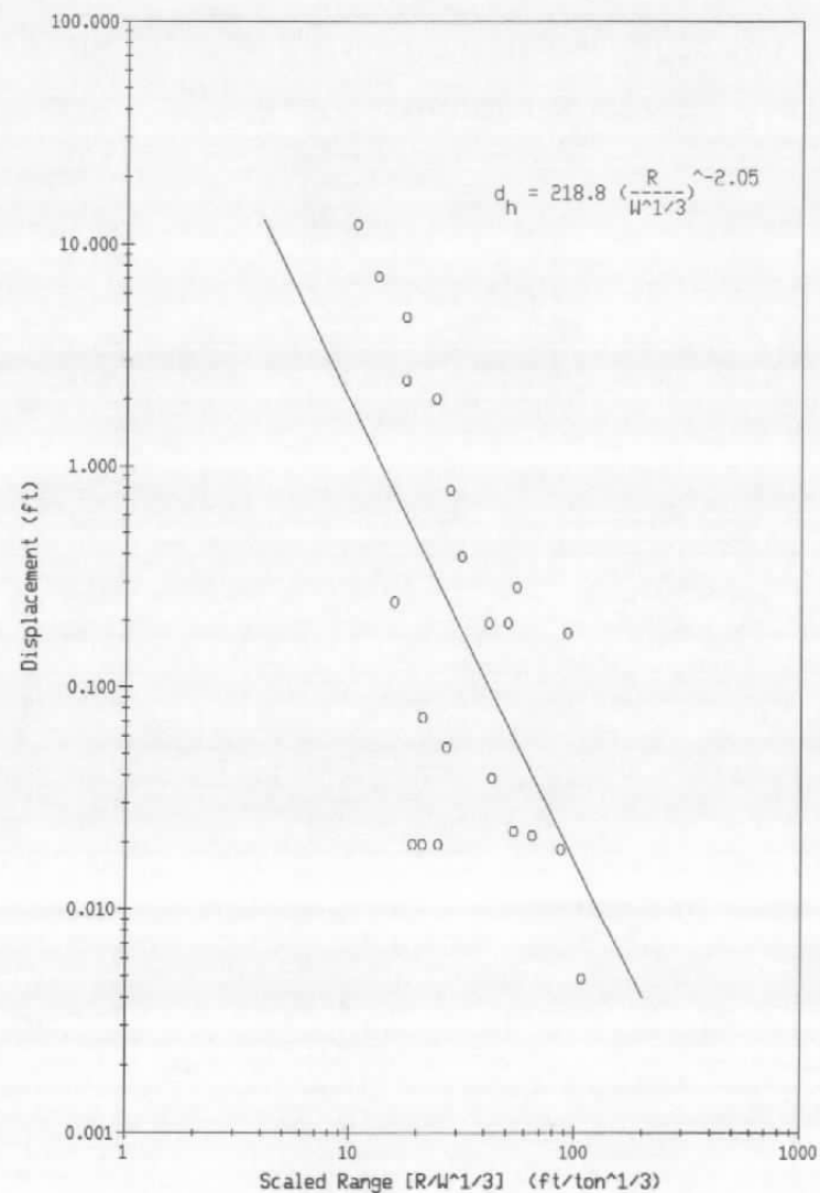
Figure 20. Peak Horizontal Displacement at 18 foot depth, from surface detonation.
