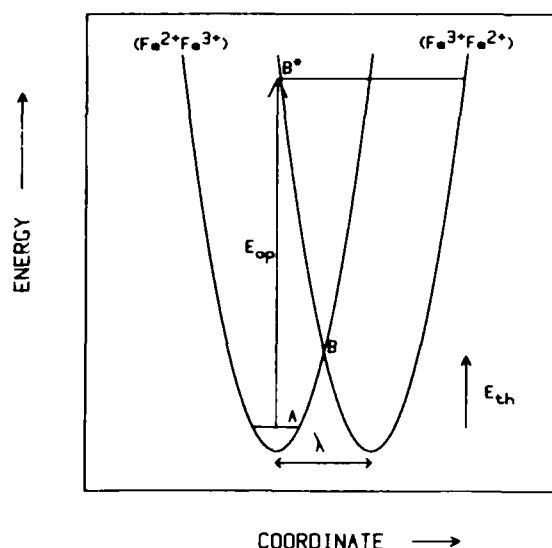
Figure 1. Vibrational potential energy vs. configurational coordinate for electron transfer via vibronic coupling between two symmetrical states of a single oscillator. A, initial state; B, vibrationally excited state; B, thermally excited state; \lambda , vibronic coupling parameter; E_{op} , optical transition energy; E_{th} , thermal transition energy. Energy of initial state (left-hand well) is same as final (right-hand well) state (from Hush, 1967).
