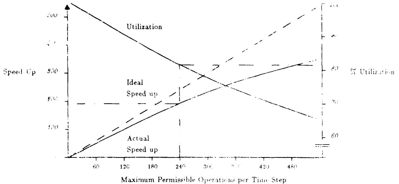
Figure 3: Speed Up and Utilization for 20 x 20 SIMPLE
