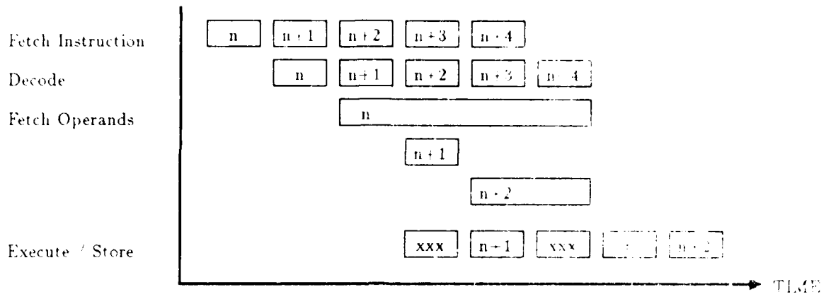
Figure 7: Variable Operand Fetch Time
