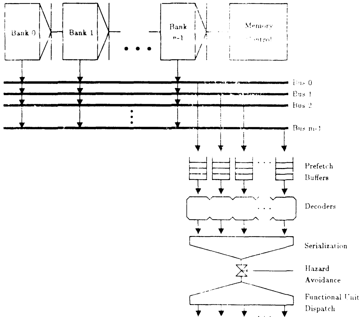
Figure 8: Hazard Avoidance at the Instruction Decode Stage
