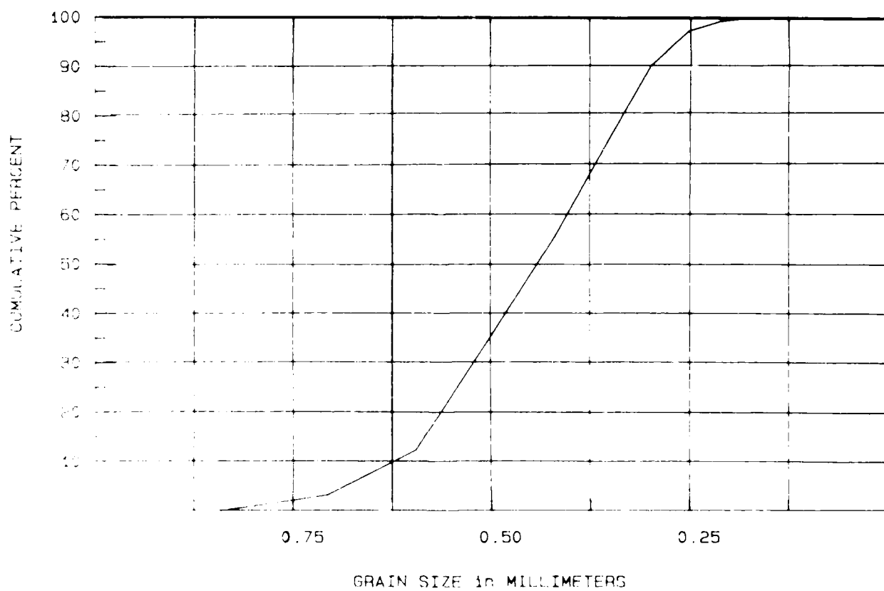
Figure 2. Grain size distribution of the sediment used in the experiments.
