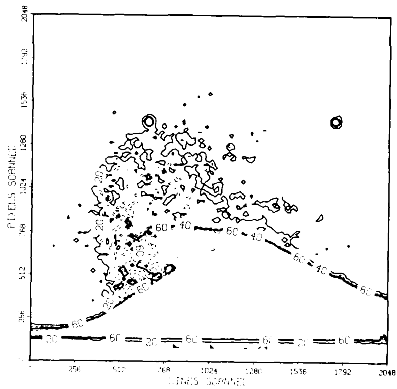
Figure 8. Light intensity contour plot from image SED8.LAN.
