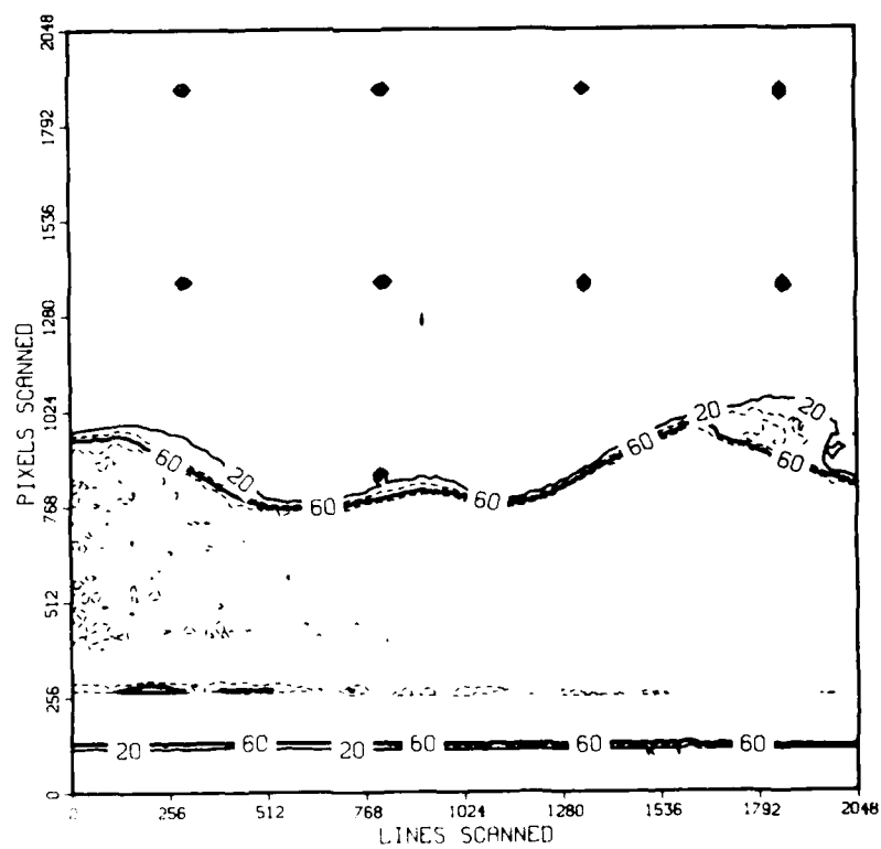
Figure 9. Light intensity contour plot from image SED6.LAN.
