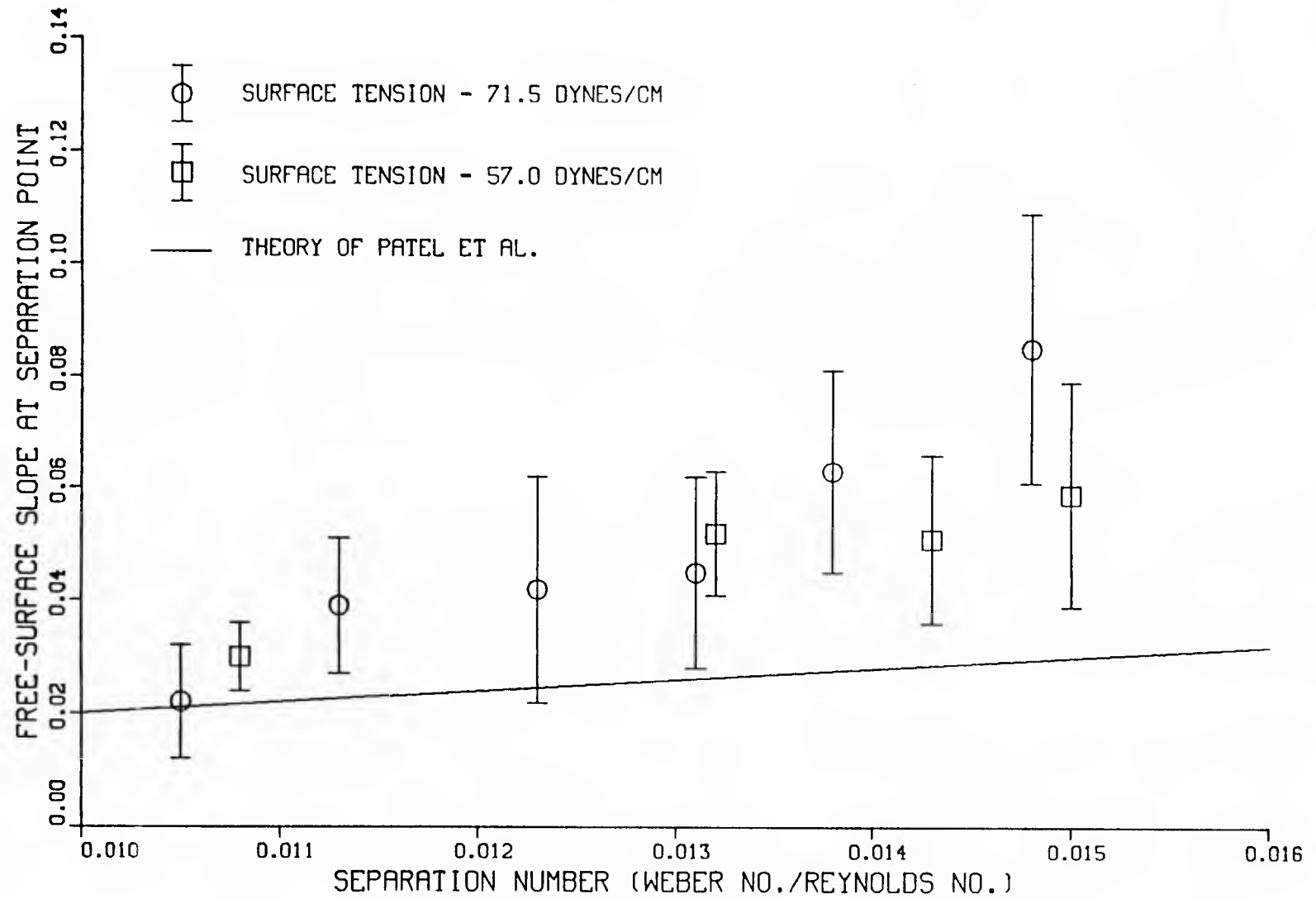
FIGURE 5: Free surface slope versus the separation number.
