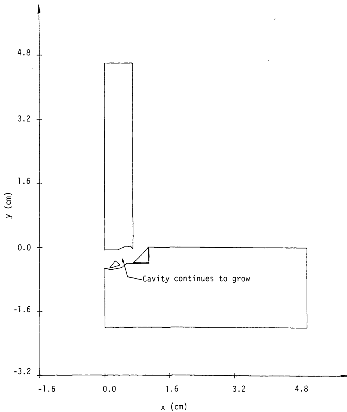
Figure 54. Fragmentation pattern after 0.869 \mu\text{sec} .
