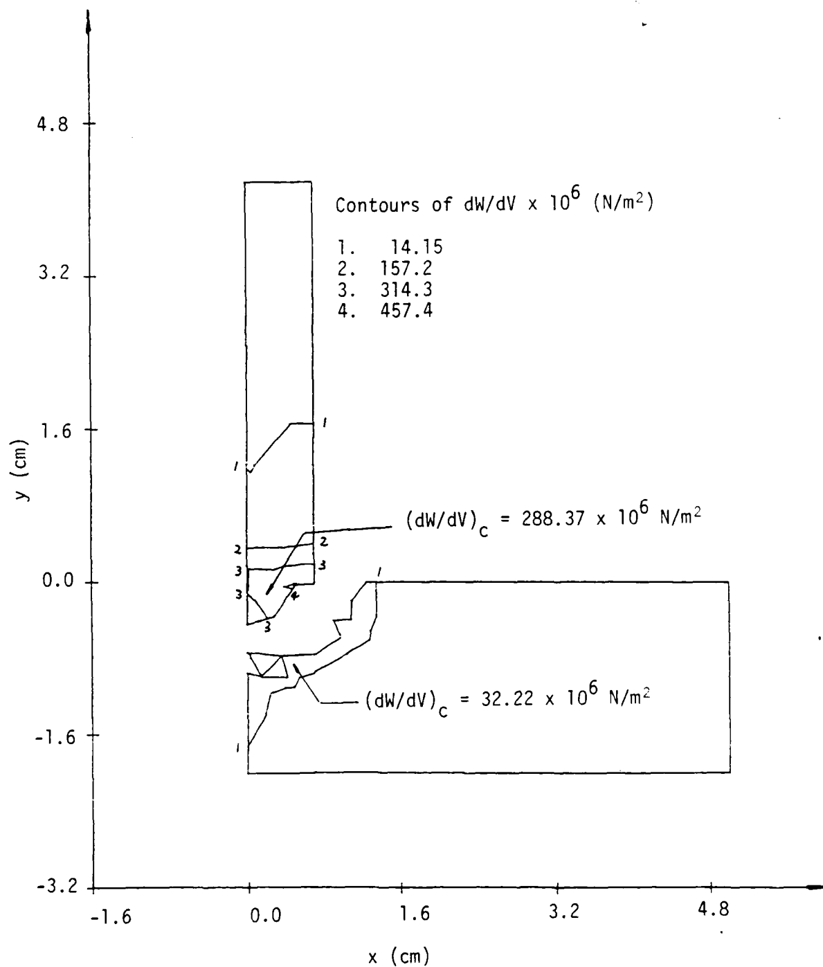
Figure 69. Contours of constant dW/dV at t = 1.259 \mu sec.
