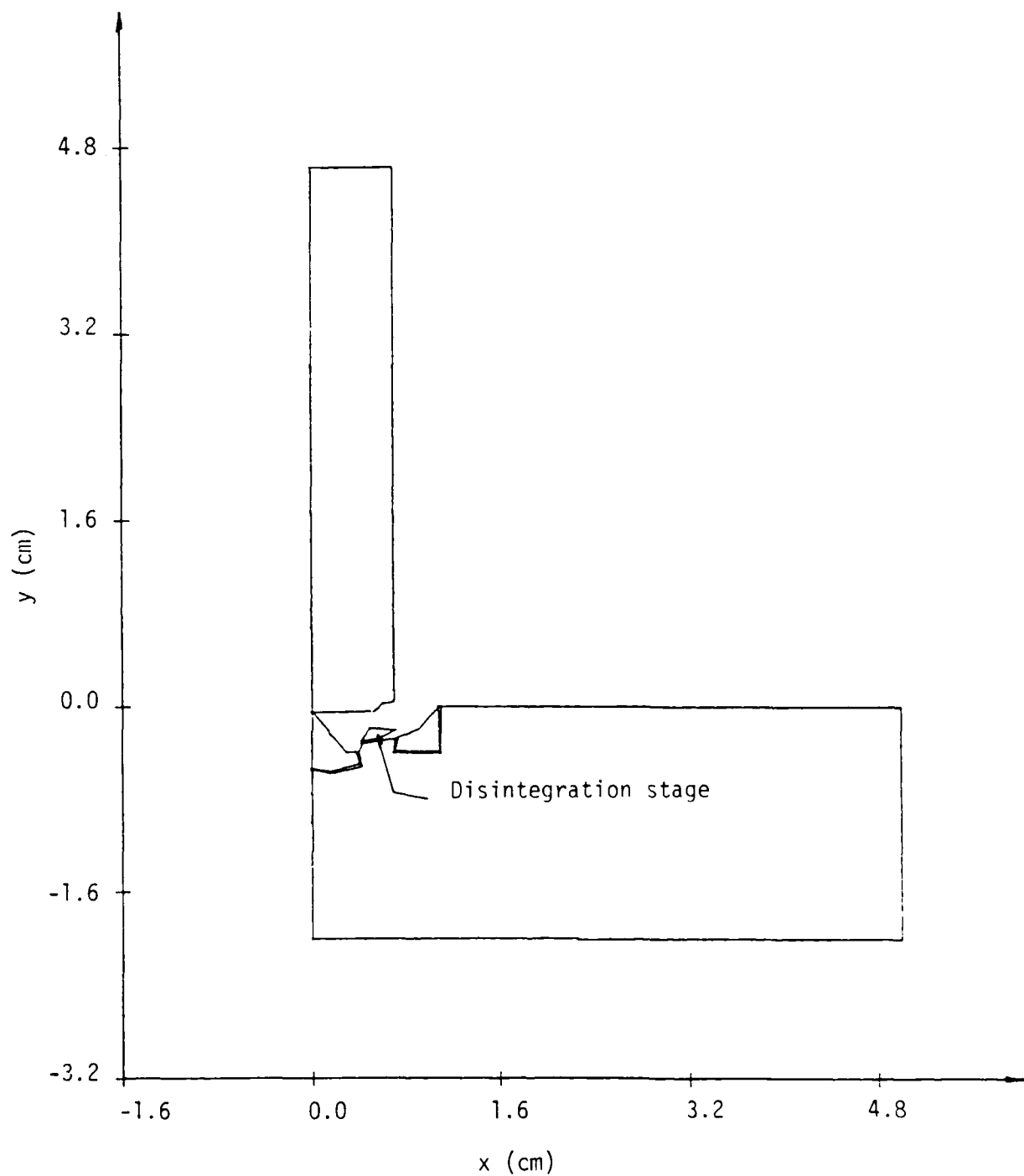
Figure 42. Damage of projectile/target after 0.562 \mu sec.
