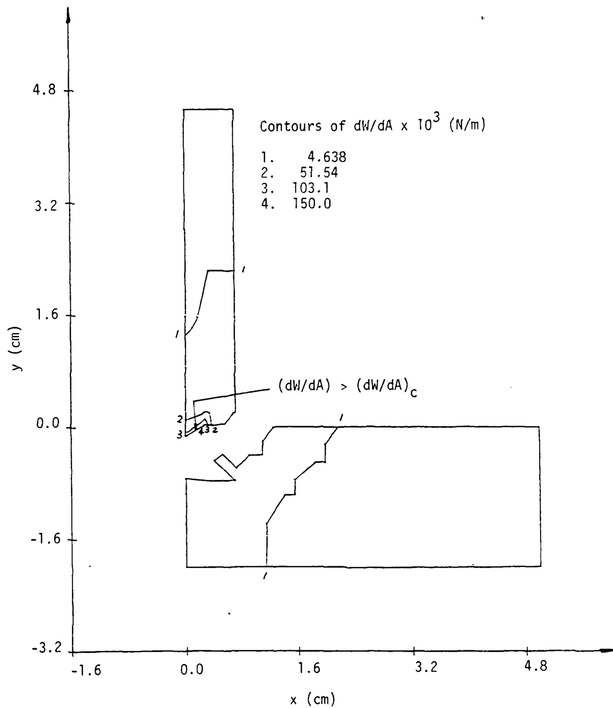
Figure 64. Contours of constant dW/dA at t = 1.224 \mu\text{sec} .
