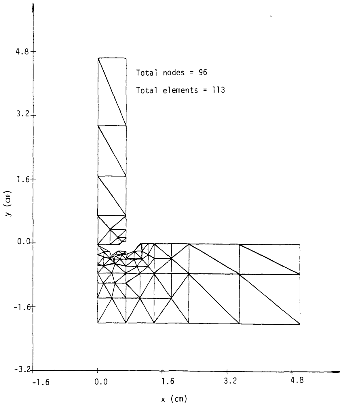
Figure 39. Grid pattern of projectile/target system after 0.501 \mu sec.
