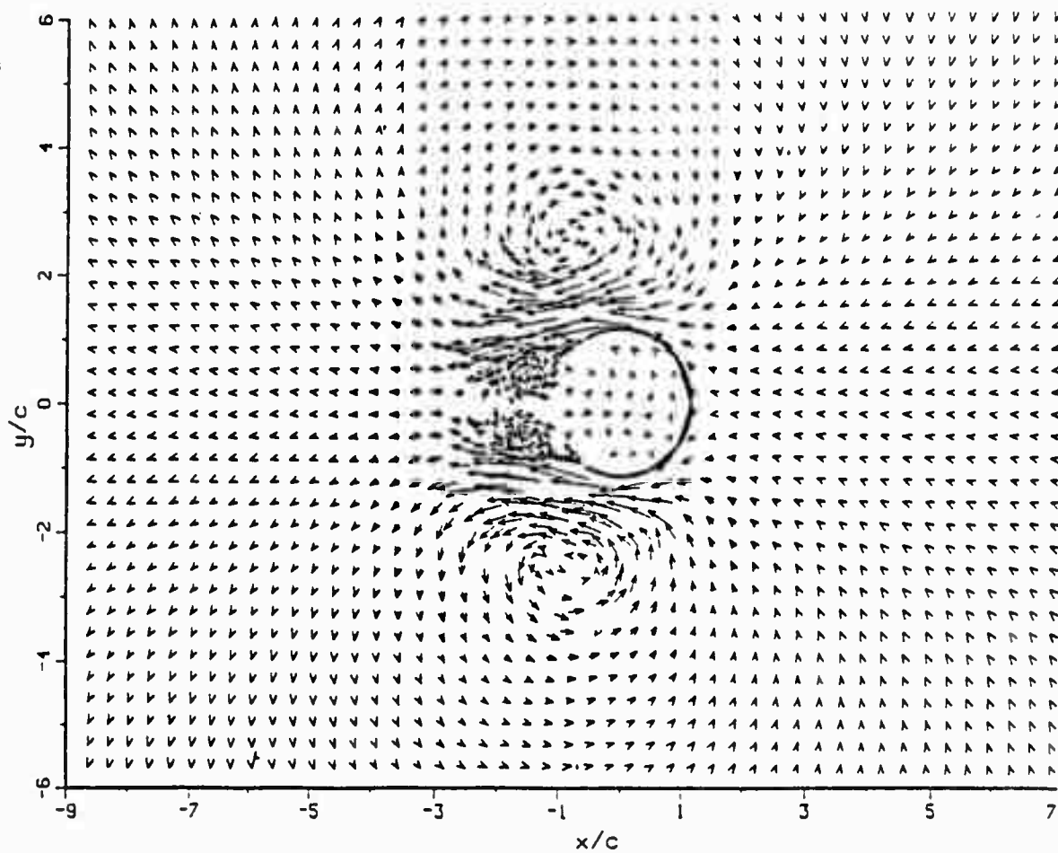
Fig. 71 Velocity Field at T^* = 20 (Model C)
