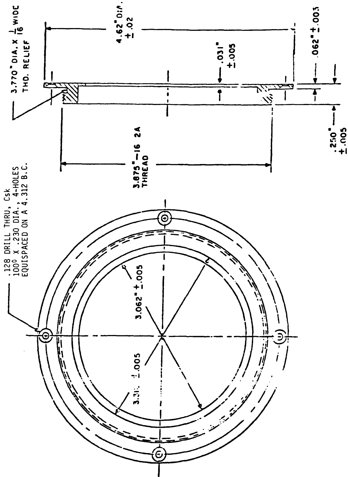
Figure 2. Camera Adapter Ring (Scale: None, Material: ALUM)
