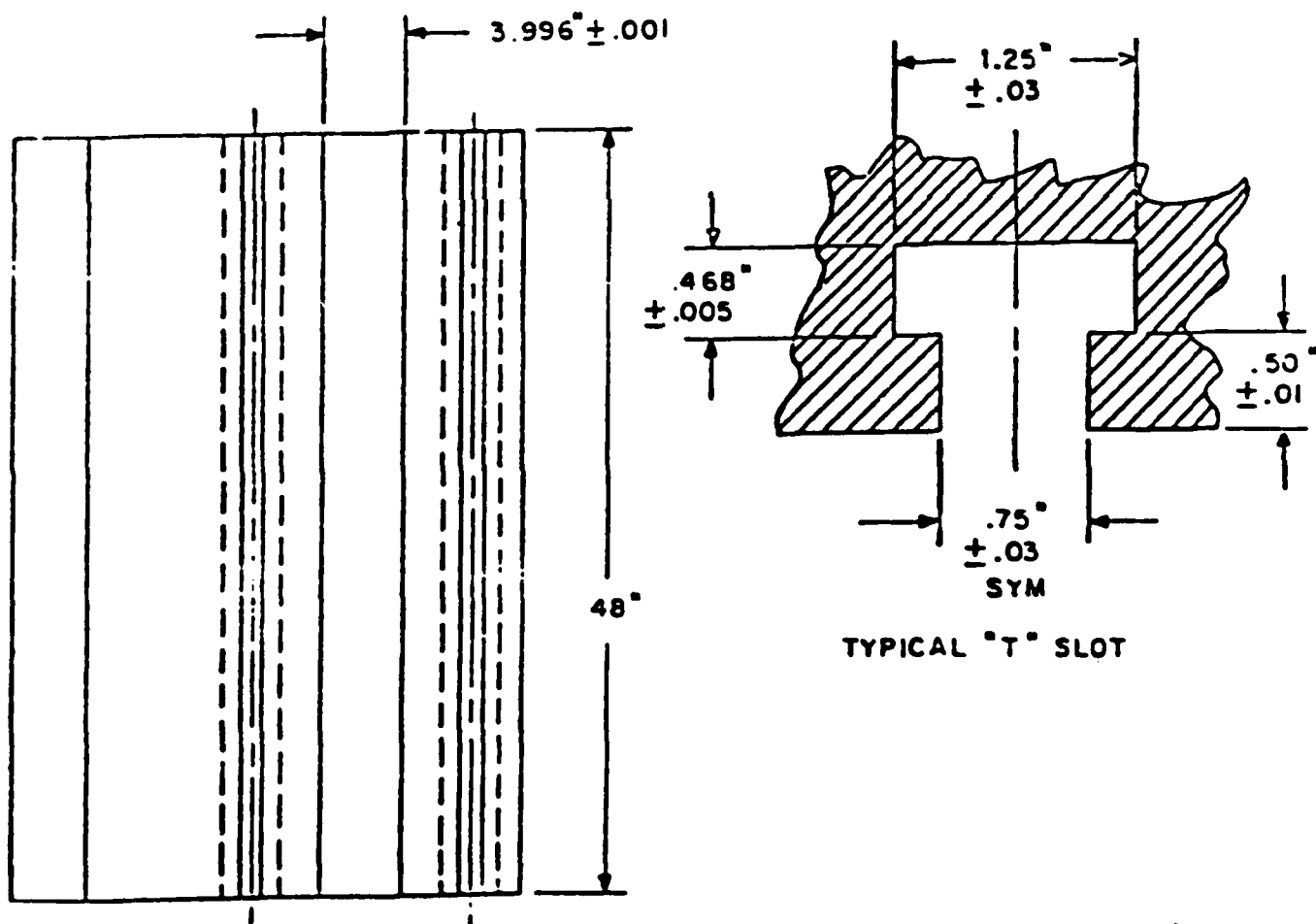
Figure 1. Instrument Mounting Platform (Scale: None)
