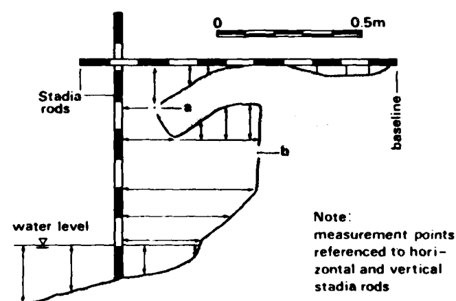
Figure 5. Profiling a bank using stadia rods (Hudson 1982).
