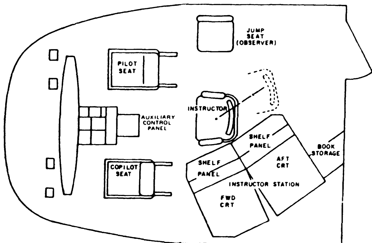
Figure 2. CH-47 flight compartment layout of CH-47 flight simulator.
