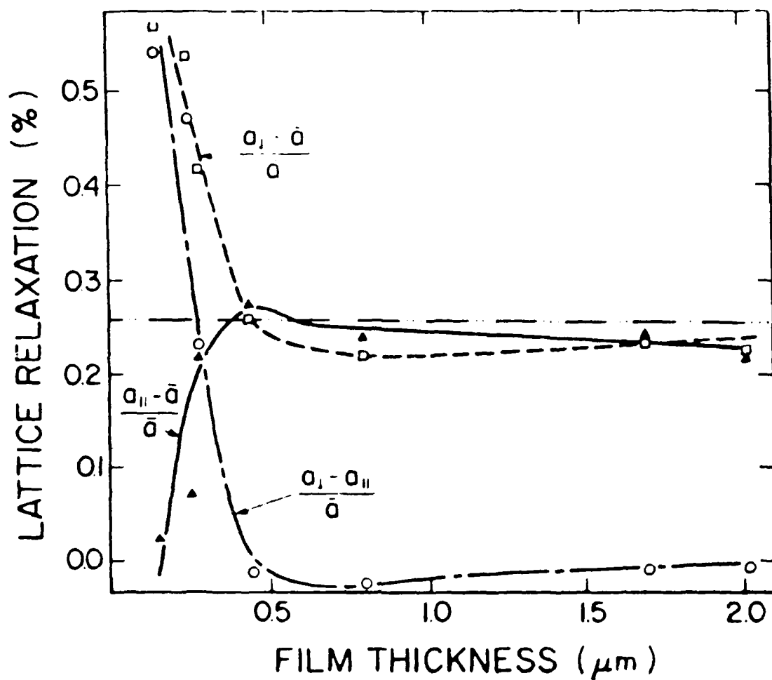
Figure 3-3. ZnSe lattice relaxation as a function of layer thickness. The lattice parameter a_I is the ZnSe lattice parameter normal to the heterointerface while a_{II} and \bar{a} are the ZnSe and GaAs lattice parameters parallel to the interface, respectively.
