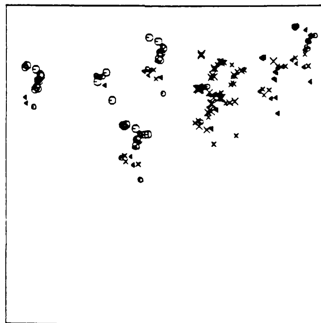
Figure 16. Projections of the m_b residuals for nine events at depths of 25 km and 50 km.
