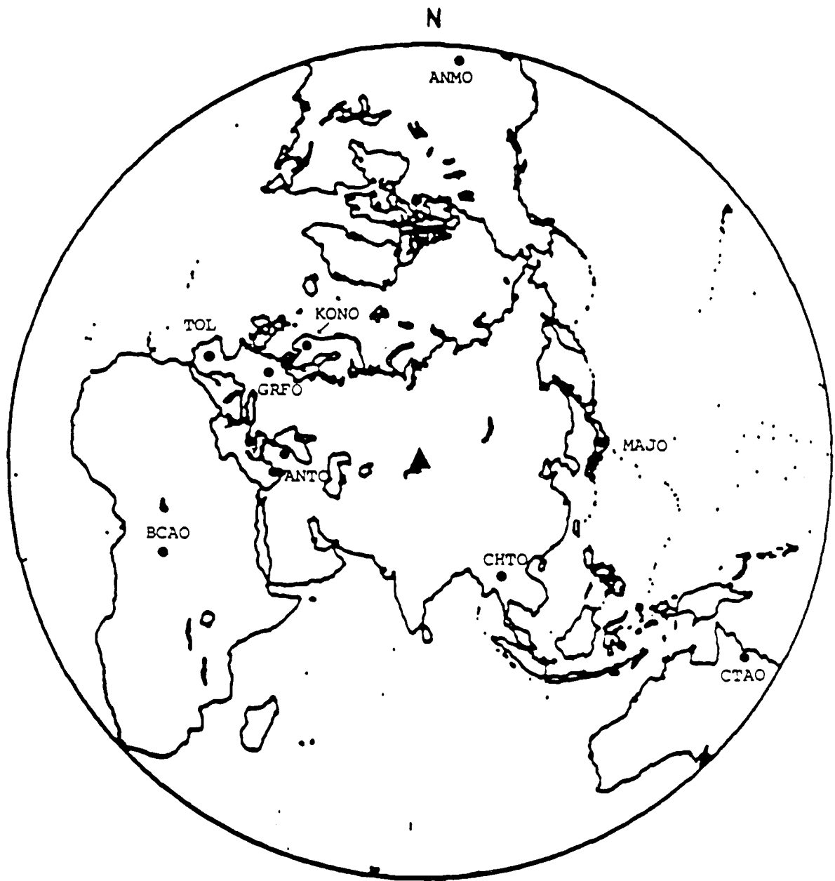
Figure 23. Map locations of selected GDSN stations shown on an azimuthally equidistant projection centered on the Shagan River test site.
