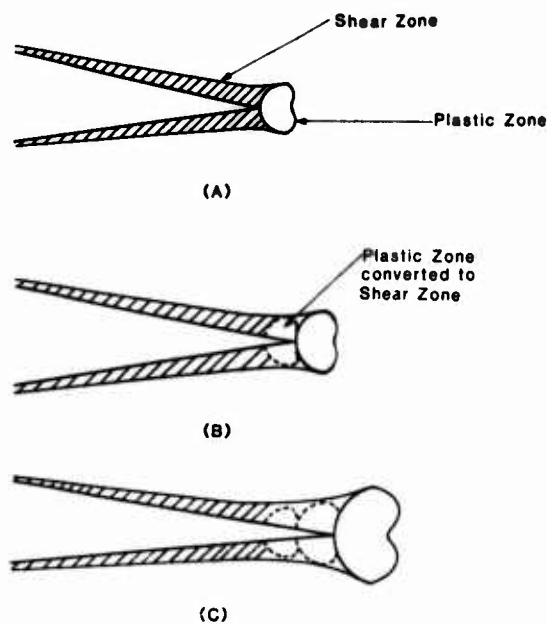
Fig. 4. Zone of plastic deformation in the vicinity of the fatigue crack[31].
