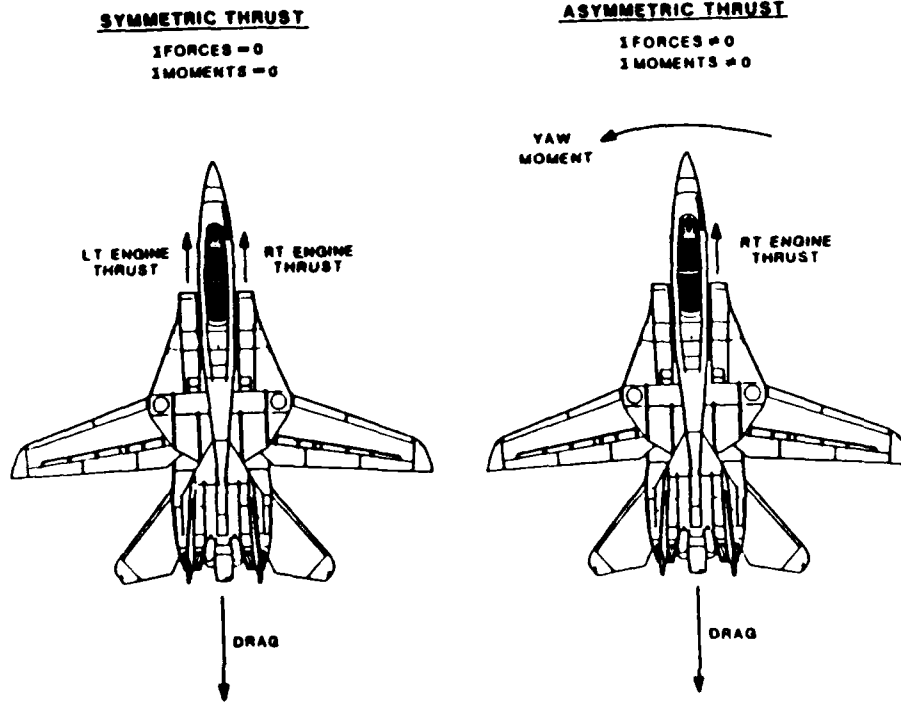
Figure 8: F-14A Aircraft
