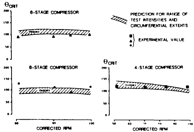
Fig. 6 Predicted and experimental critical sector angles [14]
