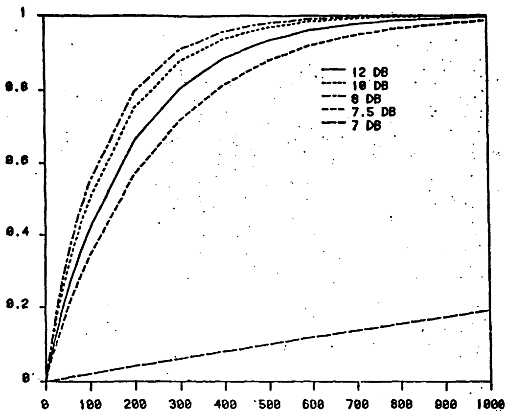
FIGURE 2 OBSERVATION TIME T_D
