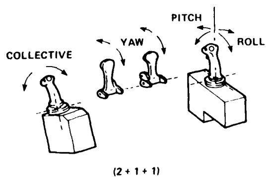
Fig. 5 Control configuration.
