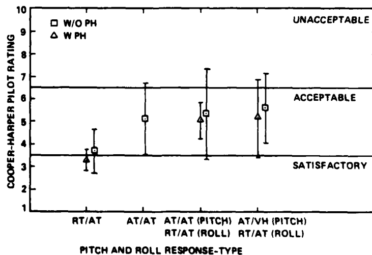
Fig. 16 SPACES II--Air-to-air attack.
