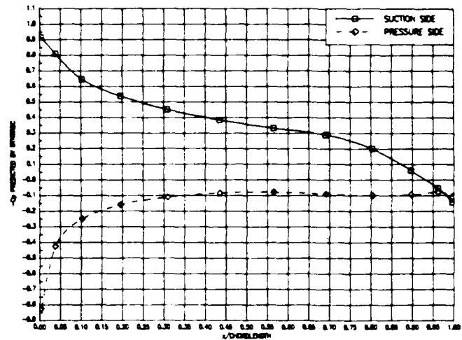
Fig. 5a. At the 40 percent radius.
