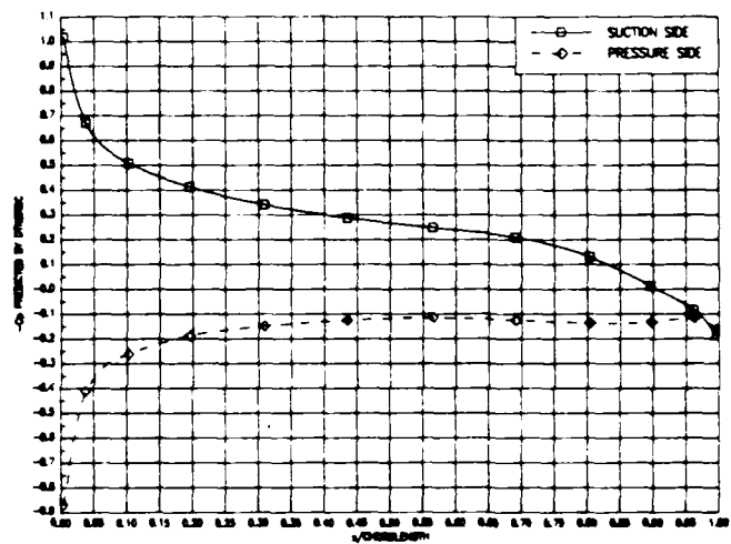
Fig. 5b. At the 50 percent radius.
