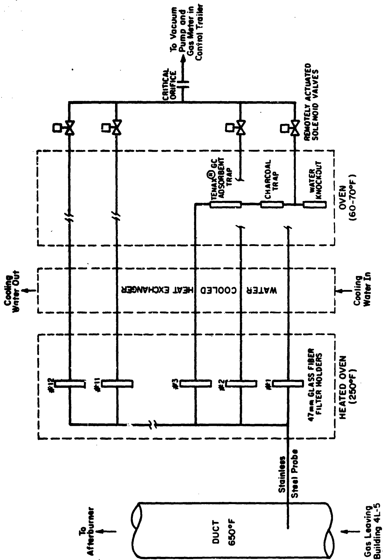
FIGURE 7-1 MODIFIED VOLATILE ORGANIC SAMPLING TRAIN (VOST)
