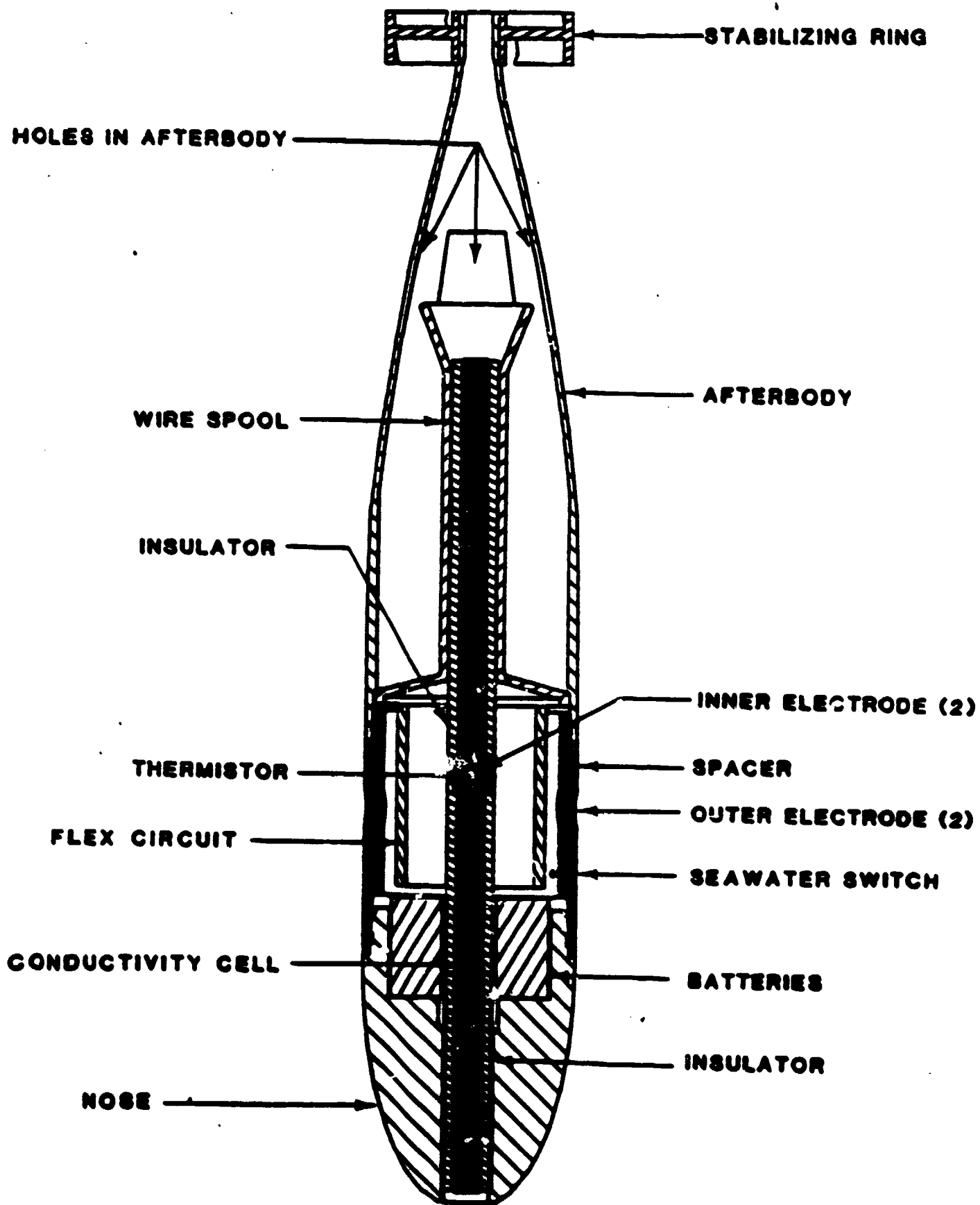
FIGURE 2-1: XCTD PROBE
