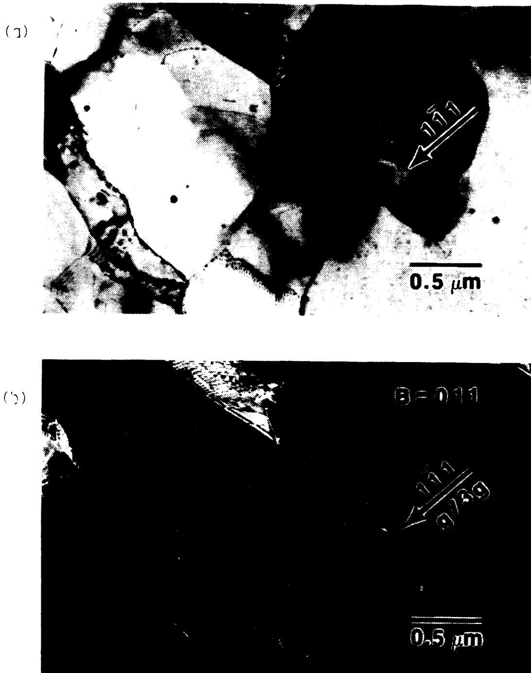
Figure 4.18 6-1 bright field dark field prior to deformation
