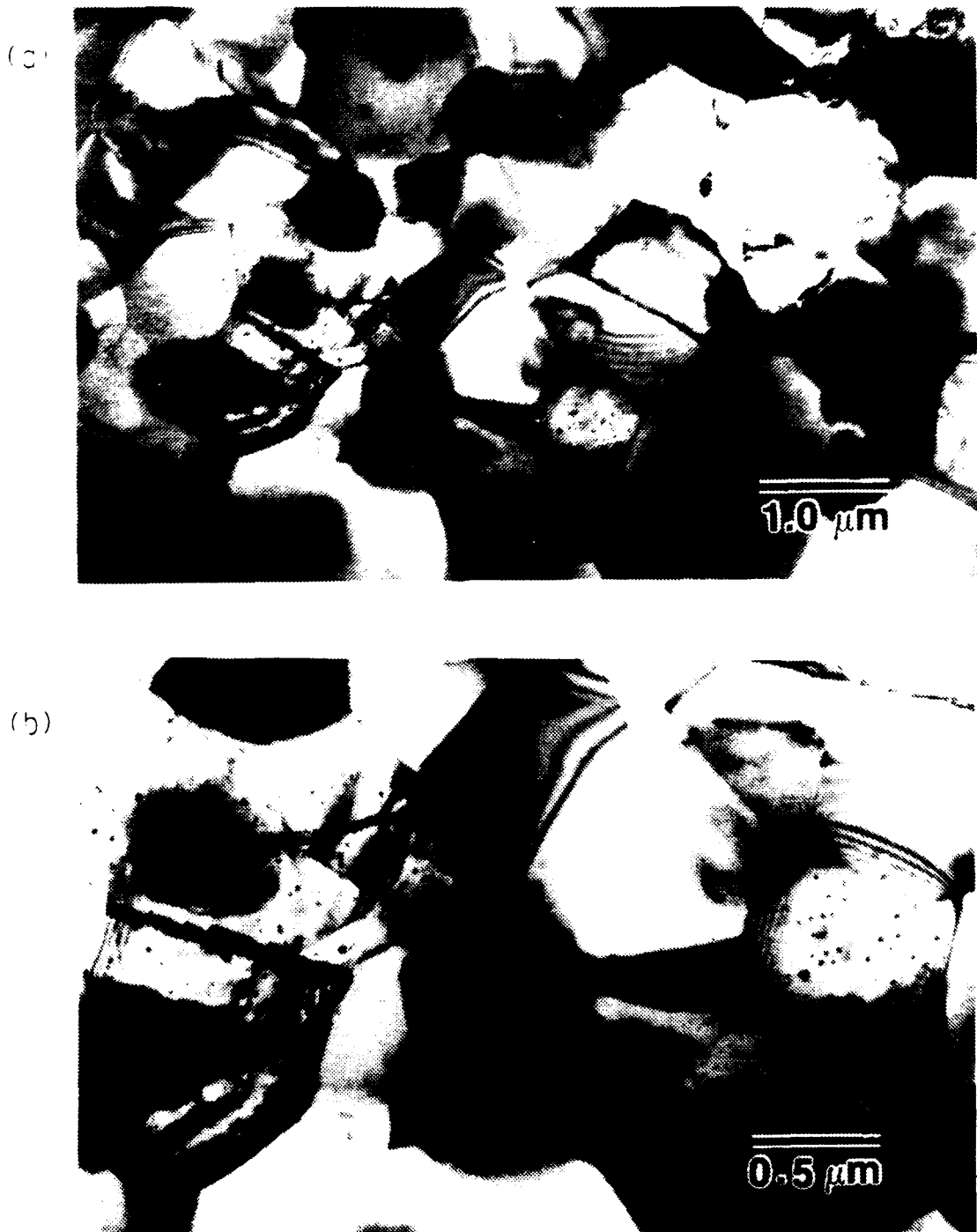
Figure 4.14 S-1 prior to deformation
