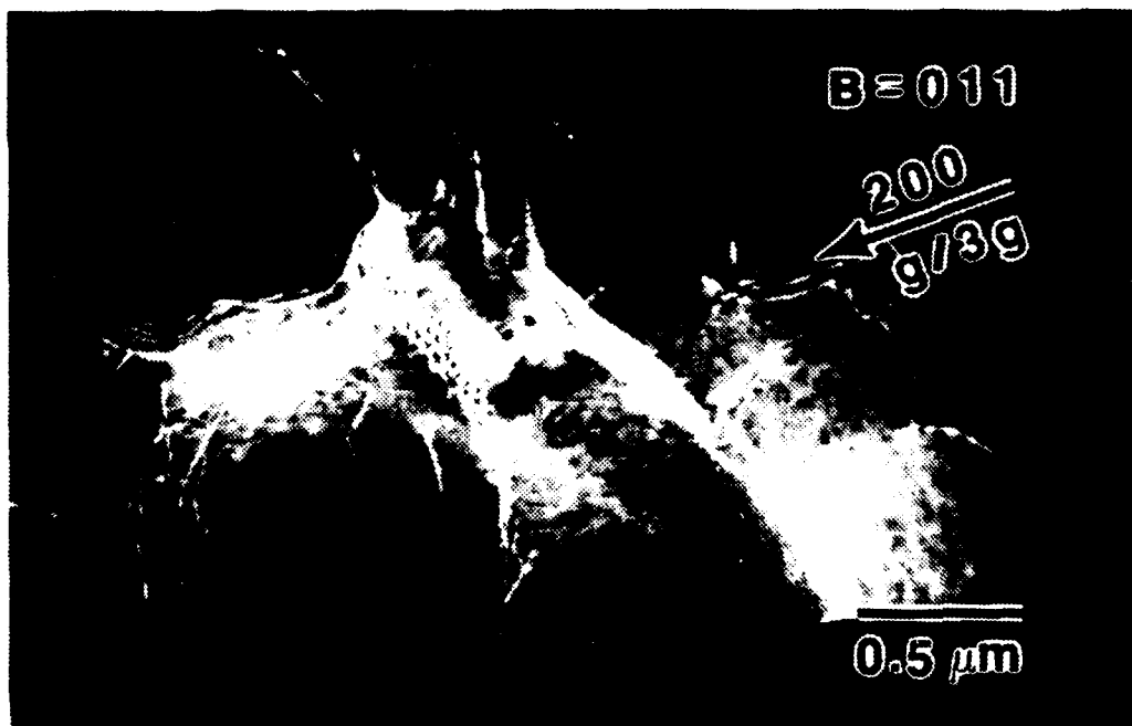
Figure 4.16 S-I bright field dark field following deformation at 1.7 \times 10^{-2} \text{ sec}^{-1}
