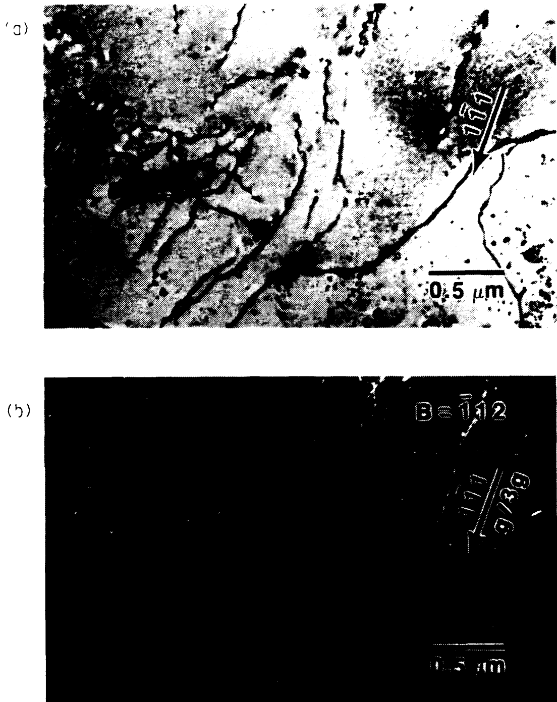
Figure 4.22 6-I bright field dark field following deformation at 6.7 \times 10^{-3} \text{ sec}^{-1}
