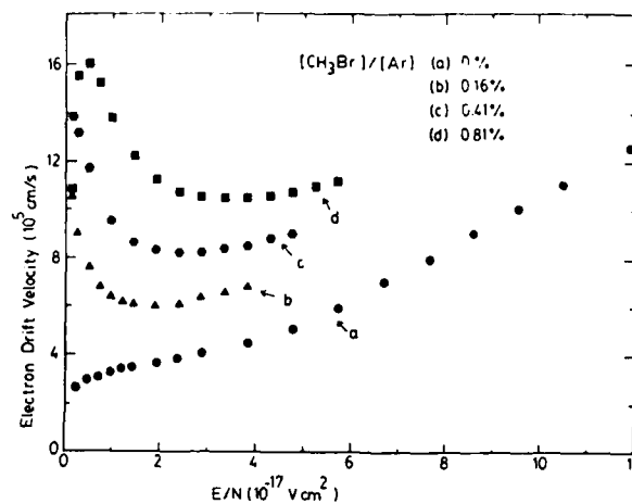
Fig. 3 Drift velocities of electrons in the gas mixture of CH 3 Br in Ar as a function of the CH 3 Br concentration
