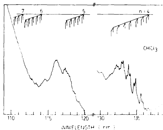
Fig. 4. Photoabsorption spectrum of \text{CHCl}_3 measured with a monochromator resolution of 0.04 nm. The wavelength positions for the vibrational progressions of tentatively assigned Rydberg series are indicated.
