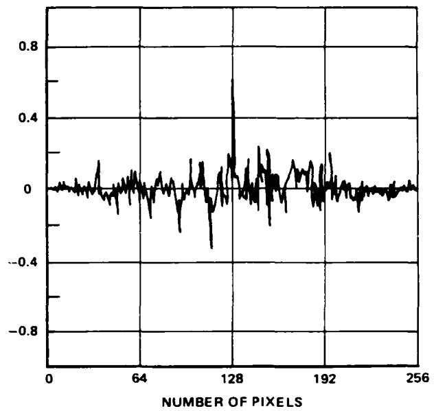
(b) CORRELATION WITH BIPOLEAR FILTER ( M = 2 )
