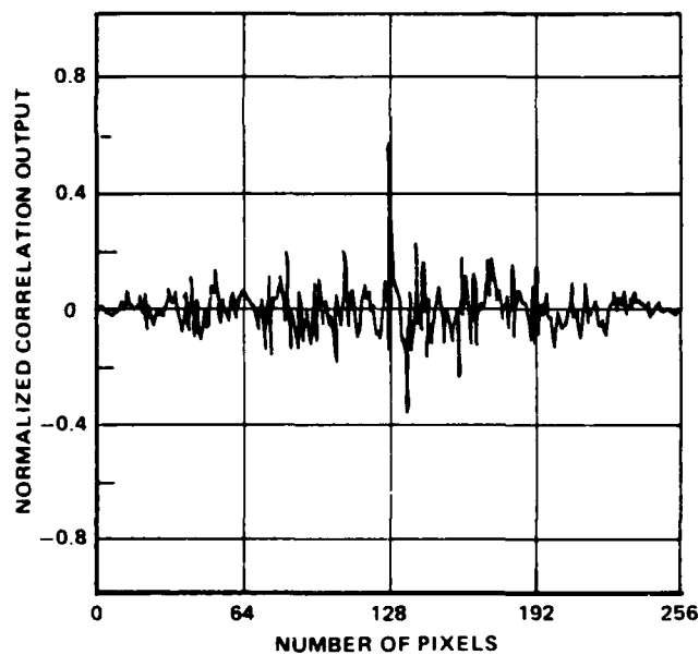
(c) CORRELATION WITH BIPOLEAR FILTER ( M = 3 )
