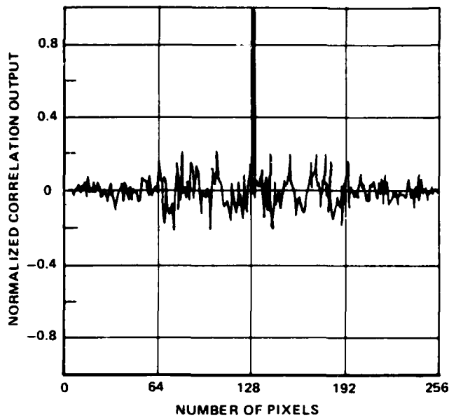
(a) CORRELATION WITH BIPOLEAR FILTER ( M = 1 )
