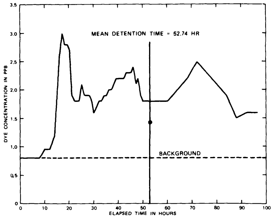
Figure 10. Dye dispersion curve, Savannah Harbor field evaluation
