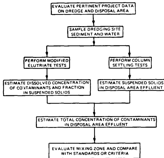
Figure 3. Steps for predicting effluent water quality
