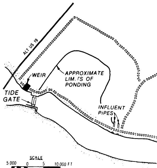
Figure 9. Plan of Disposal Area 12, Savannah Harbor
