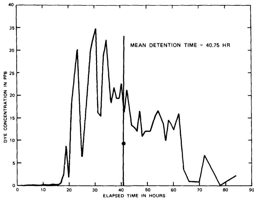
Figure 16. Dye dispersion curve, Norfolk Harbor field evaluation
