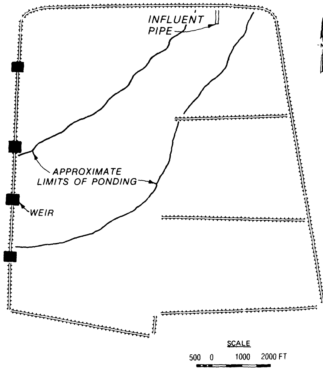
Figure 15. Plan of Craney Island disposal area, Norfolk Harbor field evaluation
