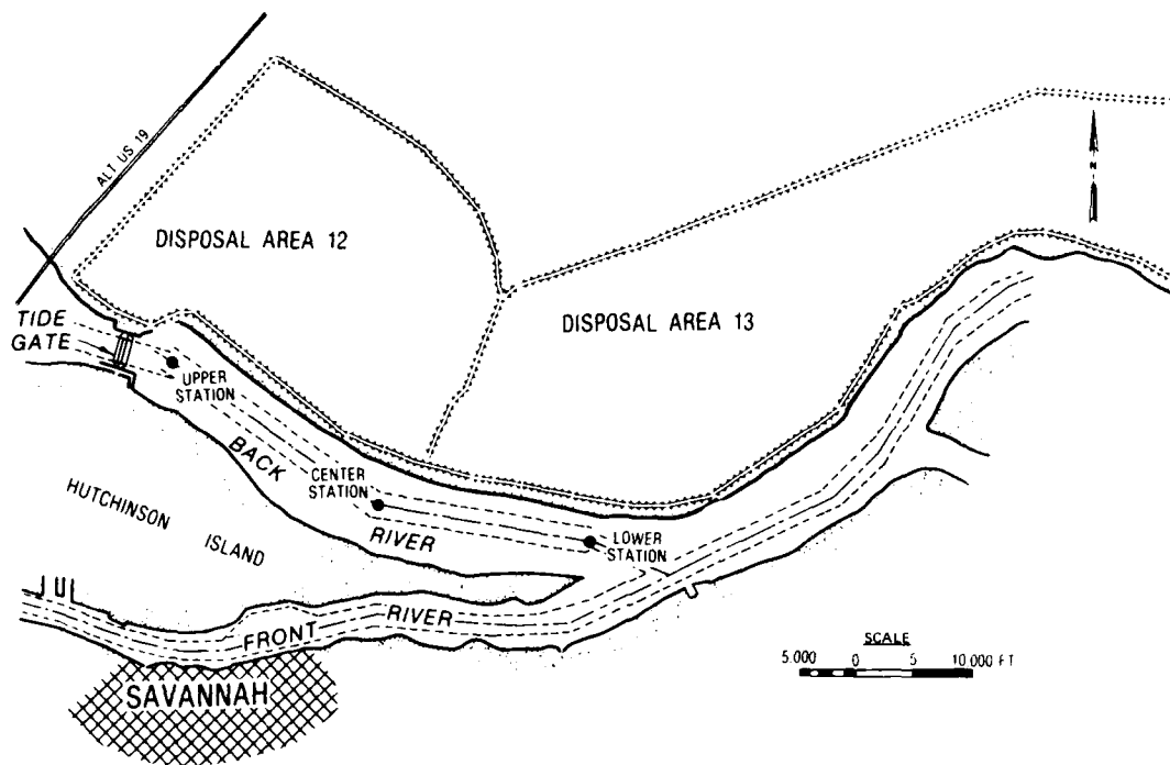
Figure 8. Savannah Harbor, Georgia, showing channels, sediment basin, and Disposal Area 12
