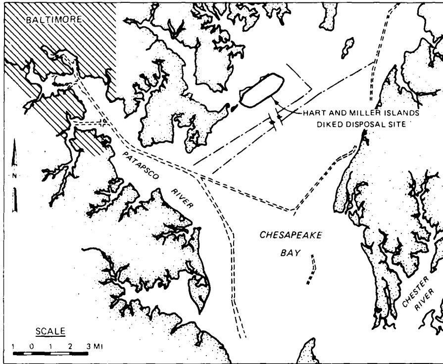
Figure 29. Hart Miller Island study area
