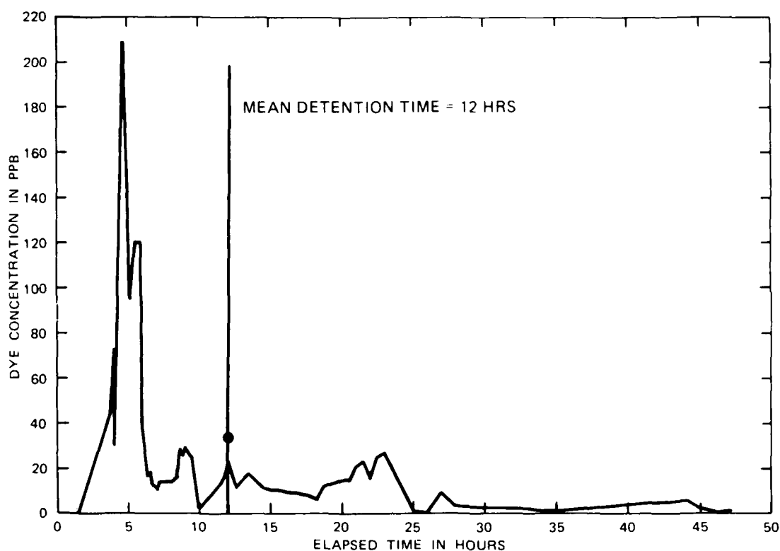
Figure 4. Dye dispersion curve, Mobile Harbor field evaluation
