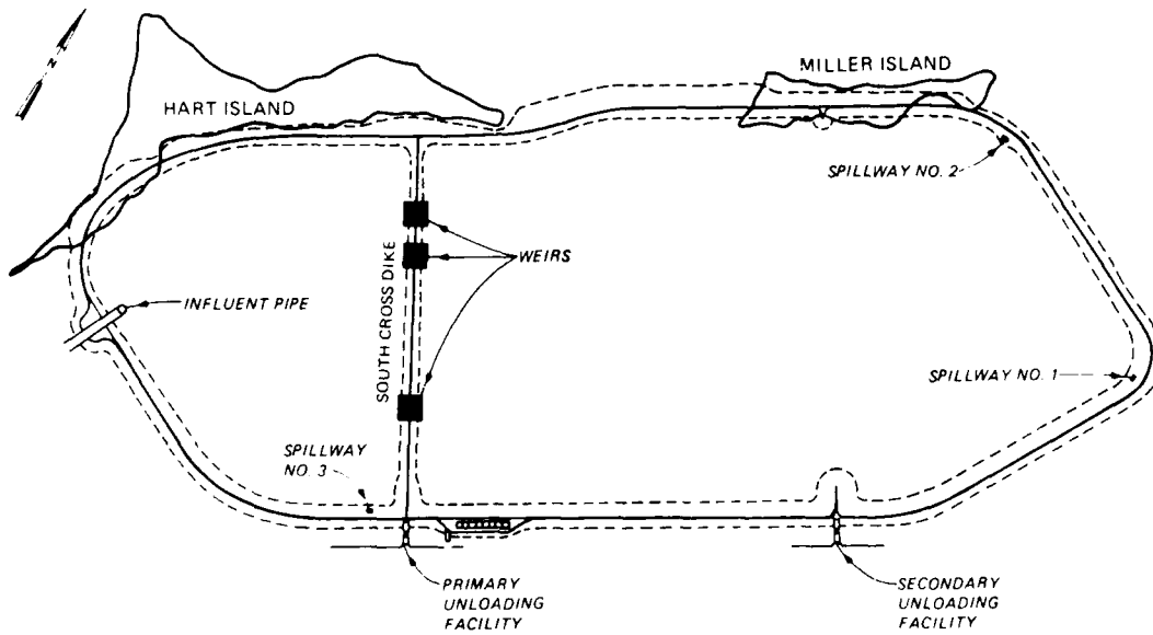
Figure 30. Hart Miller Island containment area
