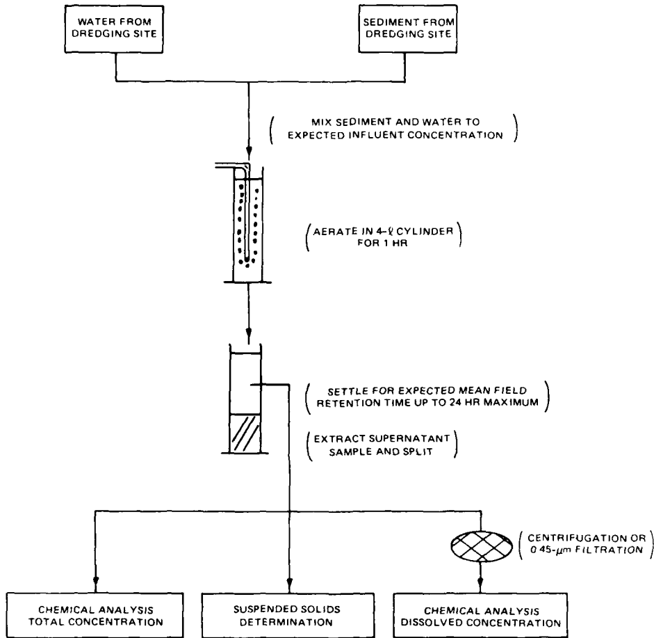
Figure 1. Modified elutriate test procedure
