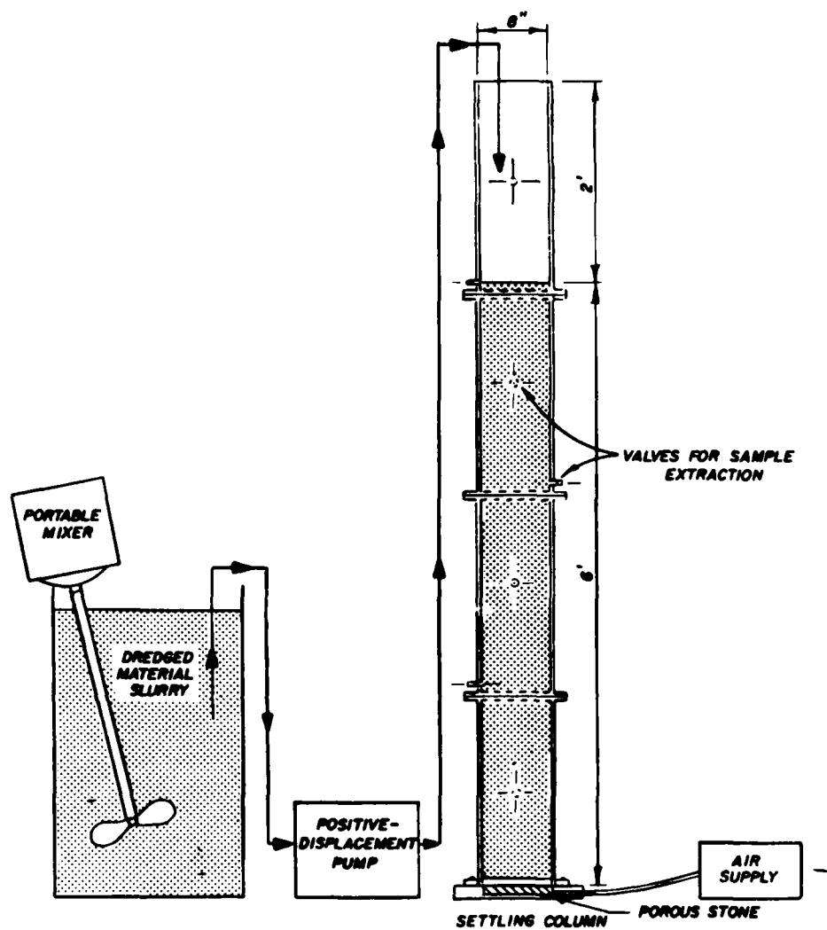
Figure 2. Schematic of apparatus for column settling tests (Montgomery 1978)
