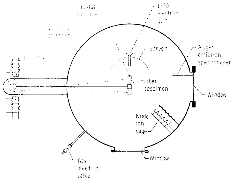
FIGURE 6-3 LEED adhesion apparatus (Buckley, 1970).
