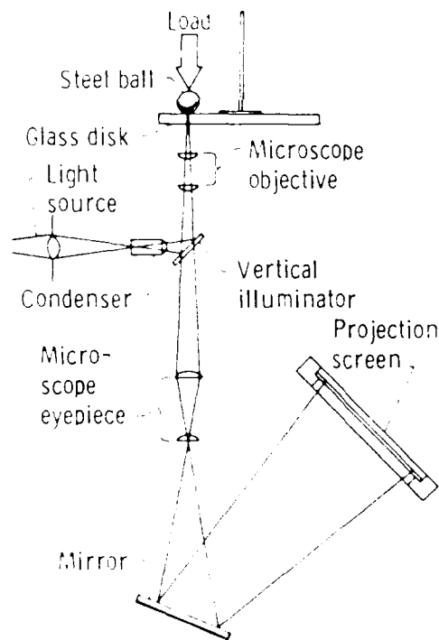
FIGURE 1 Schematic diagram of optical system (Sliney, 1978).
