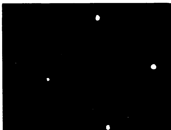
(a) clean iron (001) surface
