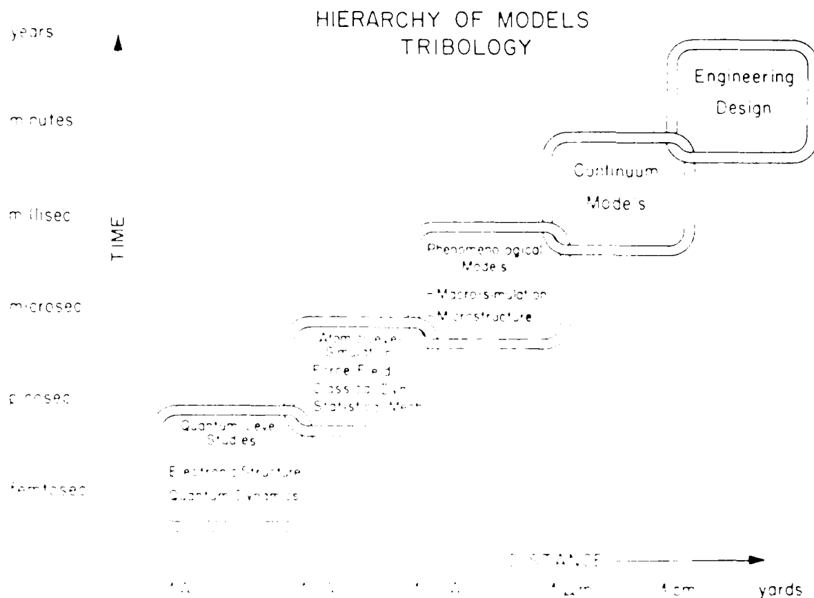
FIGURE 8-1. Relationships and connections between atomic-level descriptions of materials, and the microscopic, macroscopic, and engineering models used in rationalizing experiments and designing new materials.
