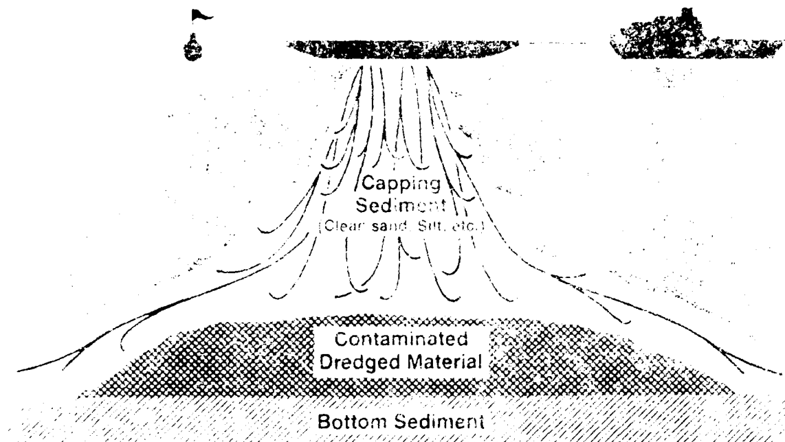
Figure 2. Schematic of typical capping operation
