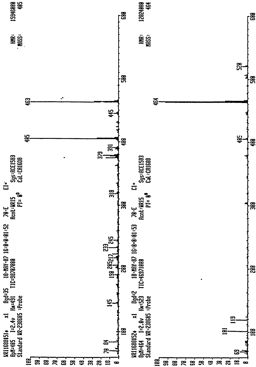
FIGURE 40 Electron Impact (upper) and Chemical Ionisation (lower) mass spectra for WR 238605
