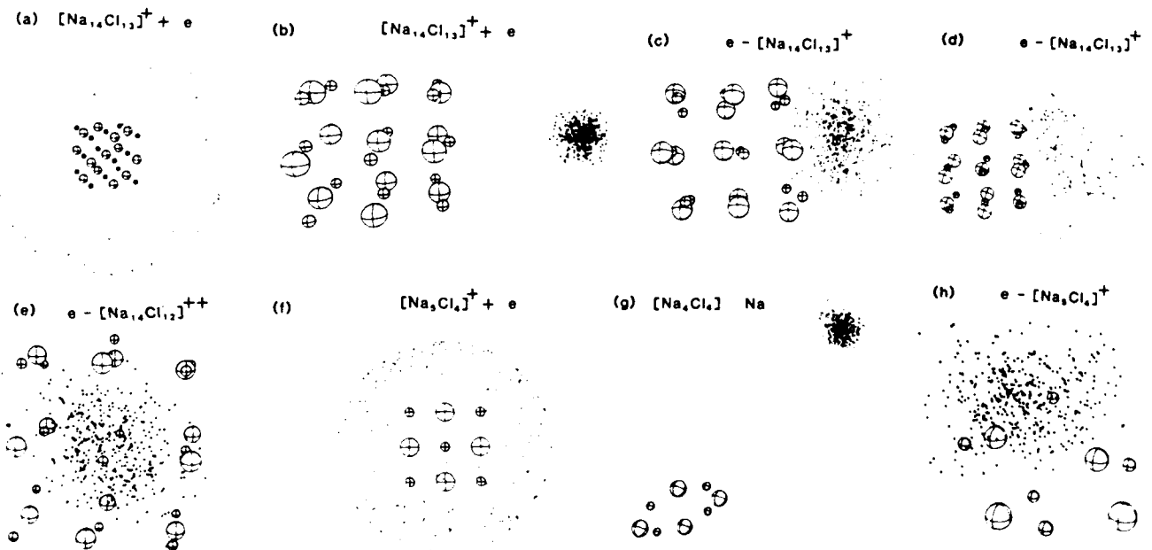
FIG. 1. Ion configurations and "electron necklace" distributions for an excess electron interacting with sodium-chloride clusters. Small and large spheres correspond to \text{Na}^+ and \text{Cl}^- ions, respectively. Dots represent 2D projections of the "electron beads." (a),(b) Alternate initial configurations of [\text{Na}_{14}\text{Cl}_{13}]^+ + e [in (b) the e bead is localized to the right of the cluster] which achieve the equilibrium configurations corresponding to surface states given in (c), R_c = 3.22a_0 , and (d) R_c = 5.29a_0 . (e) Equilibrium configuration of e - [\text{Na}_{14}\text{Cl}_{12}]^{++} , R_c = 3.22a_0 , exhibiting an internal F center. (f) Initial state of e - [\text{Na}_5\text{Cl}_4]^+ . (g) Equilibrium configuration of e - [\text{Na}_5\text{Cl}_4]^+ with R_c = 3.22a_0 resulting in dissociation of \text{Na} . (h) Equilibrium configuration of e - [\text{Na}_5\text{Cl}_4]^+ with R_c = 4.36a_0 which corresponds to structural isomerization.
