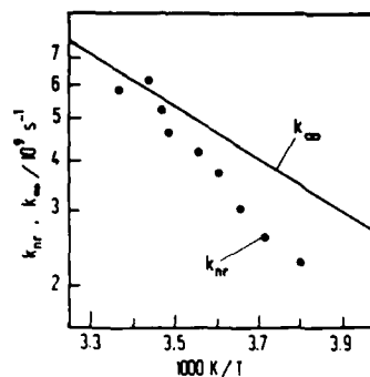
Fig. 2. Comparison of "high-pressure rate constant" k_\infty (this work) with measurements of thermalized photoisomerization rate constants k_{nr} for diphenylbutadiene in liquid ethane (experimental points \bullet from ref. [11]).
