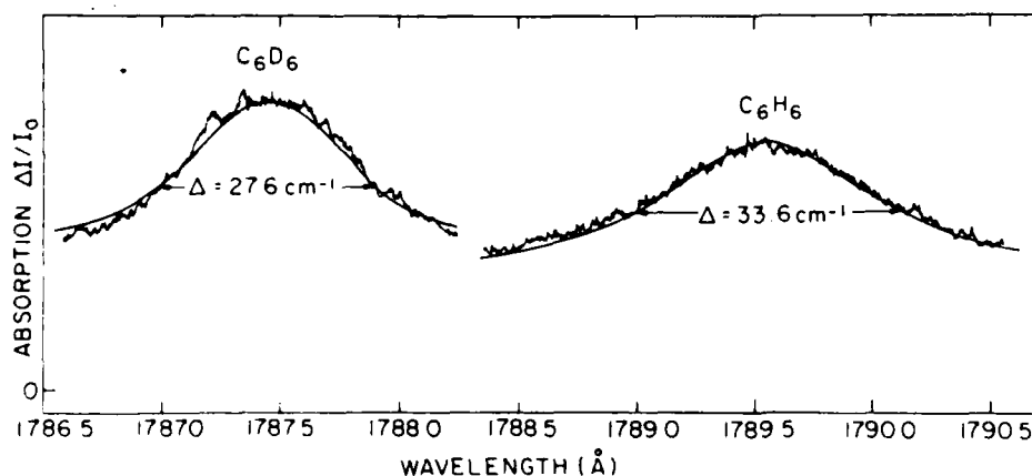
FIG. 1. Absorption spectra of the ^1A_{1g} \rightarrow 3P_{x,y}(A_{2u}) electronic origin of benzene and benzene-D 6 in pulsed planar supersonic expansions of Ar at p = 105 Torr. The spectral resolution is 0.45 Å. The base line is marked as zero on the intensity scale. The solid curves represent fits of the line shape L(\lambda) to a Lorentzian superimposed on a constant background L(\lambda) = A + C/[(\lambda - \lambda_0)^2 + (\Delta/2)^2] . For C 6 H 6 : A = 5.7 , C = 17.2 (in arbitrary units), \lambda_0 = 1789.65 Å and \Delta = 1.08 Å (33.7 cm -1 ) while for C 6 D 6 : A = 6.5 , C = 12.6 (in arbitrary units), \lambda_0 = 1787.45 Å and \Delta = 0.88 Å (27.5 cm -1 ).
