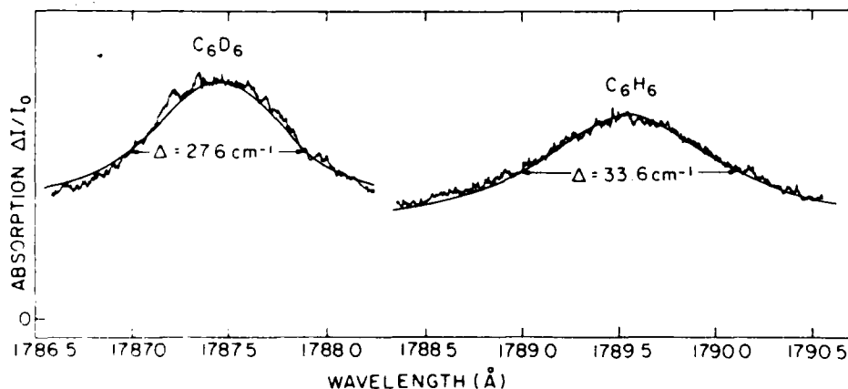
FIG. 1. Absorption spectra of the ^1A_{1g} \rightarrow 3P_{x,y}(A_{2u}) electronic origin of benzene and benzene-D 6 in pulsed planar supersonic expansions of Ar at p = 105 Torr. The spectral resolution is 0.45 Å. The base line is marked as zero on the intensity scale. The solid curves represent fits of the line shape L(\lambda) to a Lorentzian superimposed on a constant background L(\lambda) = A + C/[(\lambda - \lambda_0)^2 + (\Delta/2)^2] . For C 6 H 6 , A = 5.7 , C = 17.2 (in arbitrary units), \lambda_0 = 1789.65 Å and \Delta = 1.08 Å (33.7 cm -1 ) while for C 6 D 6 , A = 6.5 , C = 12.6 (in arbitrary units), \lambda_0 = 1787.45 Å and \Delta = 0.88 Å (27.5 cm -1 ).
