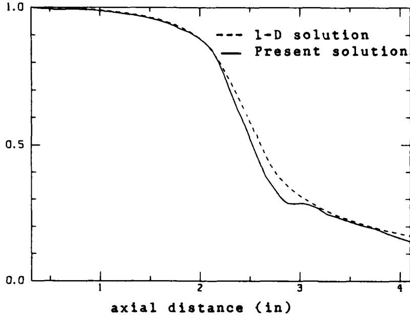
Figure 5: Axis pressure ratio
