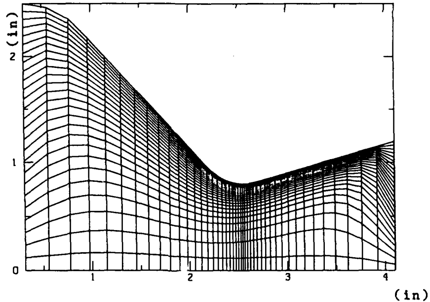
Figure 3: Grid lines (\xi, \eta) in the physical domain ( for the Poisson equation ).
