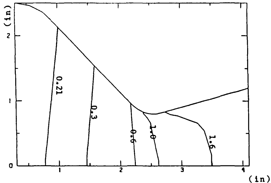
Figure 4: Contour plot of Mach number
