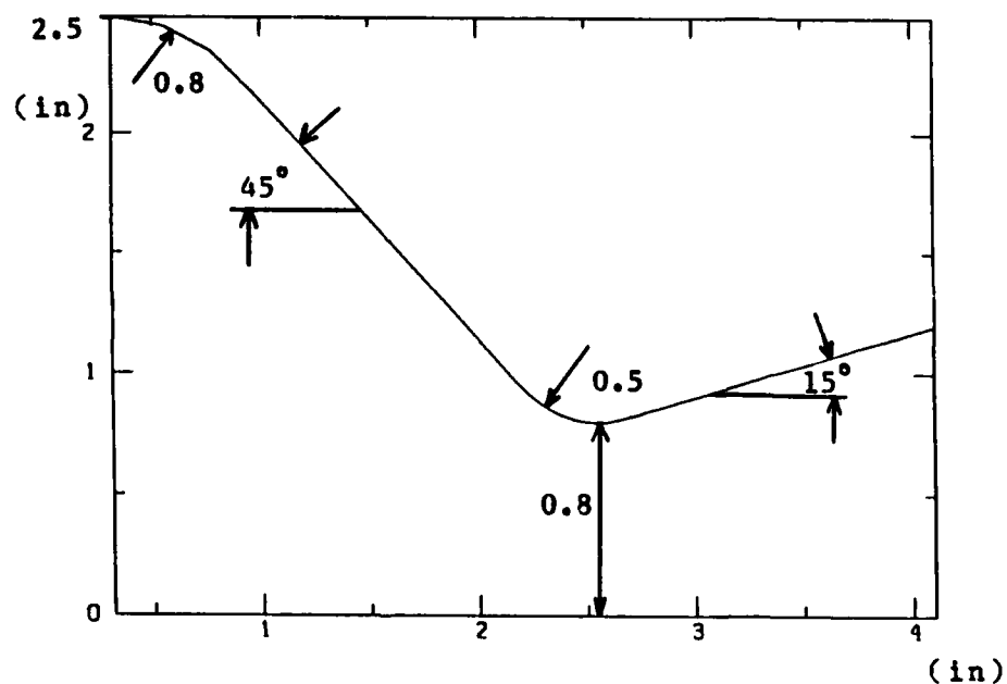
Figure 1: 45° - 15° Convergent-Divergent Nozzle
