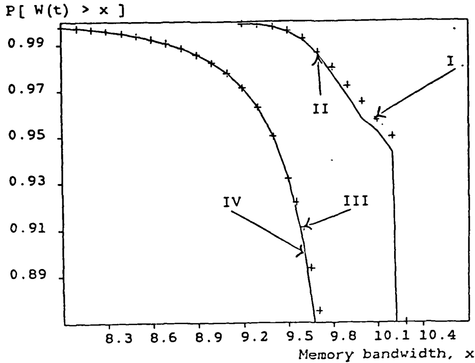
Figure 9: Complementary Distribution of Time-Averaged Accumulated Bandwidth W^c(x, t) for Different Networks and Different Repair Policies.
