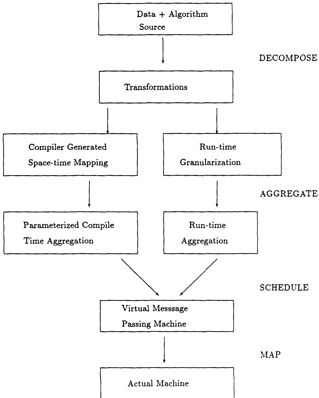
Figure 4. Data and Control Flow in Crystal Runtime System.
