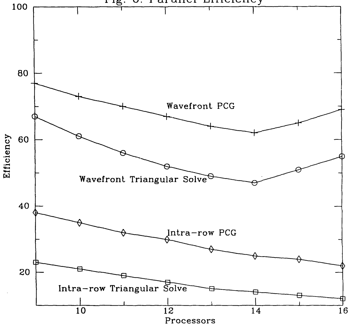
Fig. 6: Parallel Efficiency
