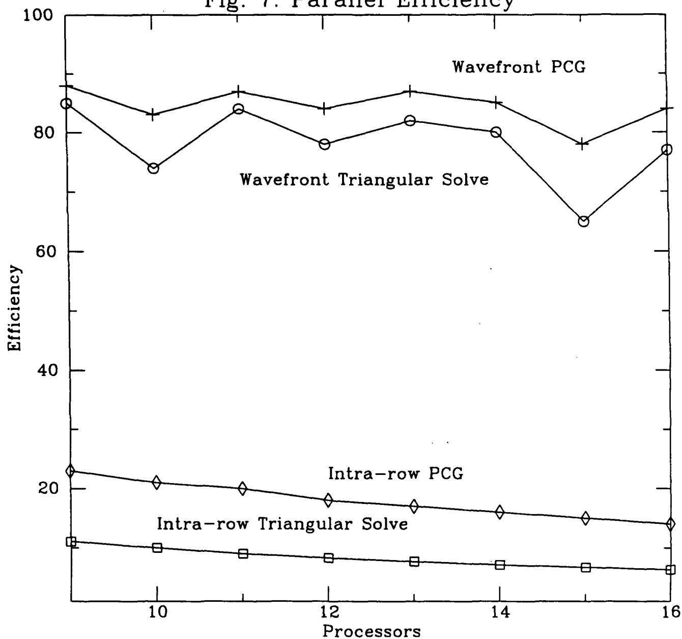
Fig. 7: Parallel Efficiency
