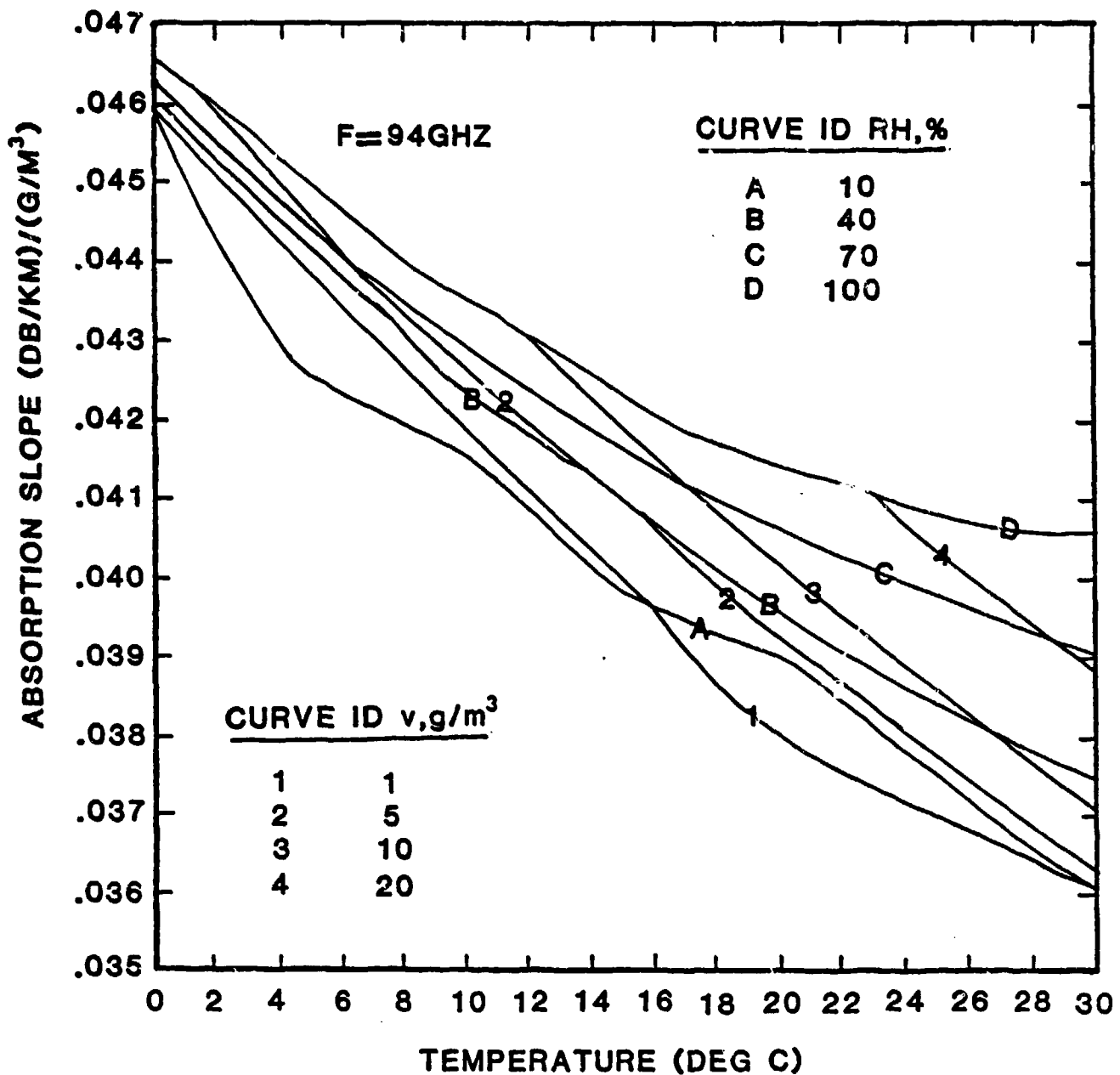
Figure 2-6. Water Vapor Absorption Slope Predicted by the EOSAEL Model at F=94 GHz, T=[0,30]^{\circ}\text{C} , for Selected Absolute and Relative Humidities.
