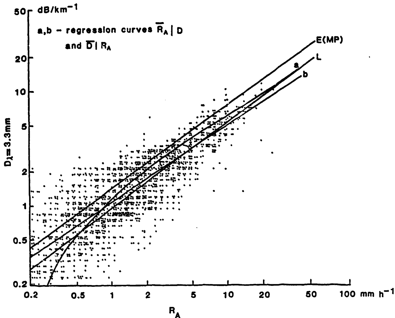
Figure 3-18. Measured Attenuation Coefficients Versus Rainfall Rate at \lambda = 3.3 \text{ mm} (90.8 GHz) (after Sander, 1975). Added Lines Indicate LIEBE and EOSAEL Model Predictions. A Rain Temperature of 10°C is Used for the EOSAEL Model Prediction.
