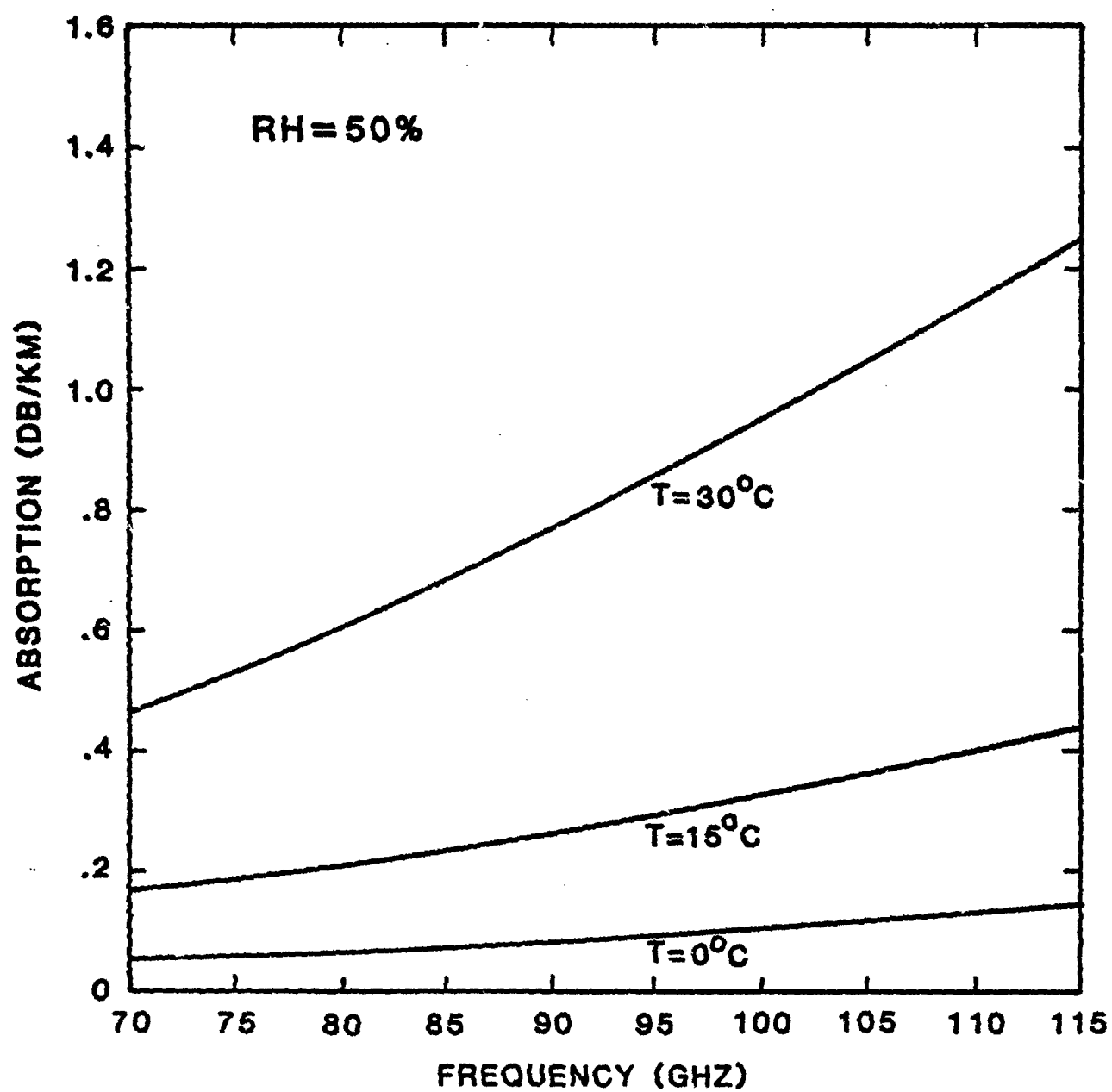
Figure 2-4. LIEBE Model Water Vapor Continuum Absorption Predictions at T=0,15,30^{\circ}\text{C} , F=[70,115] GHz, for a Relative Humidity of 50%.
