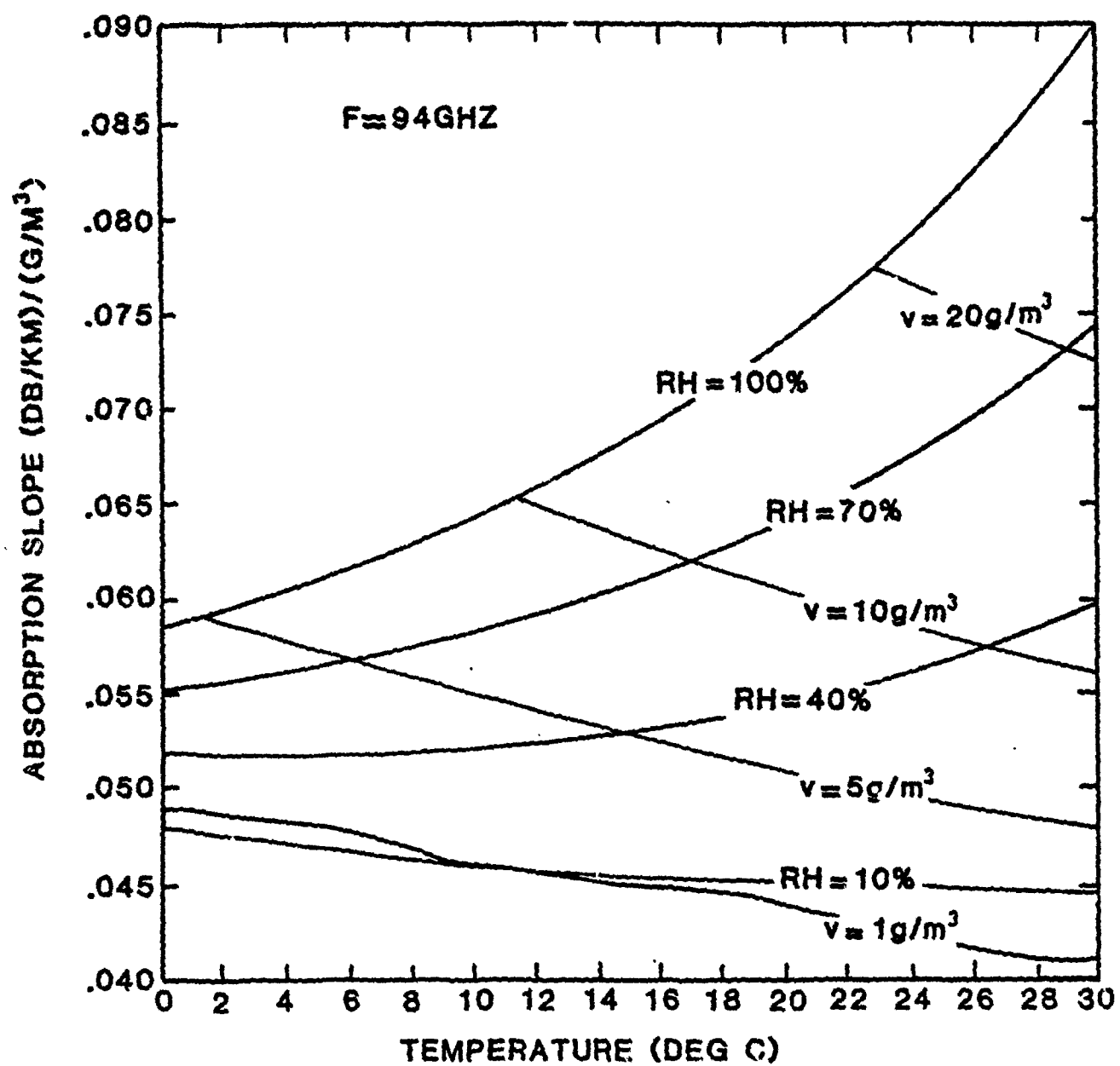
Figure 2-7. Water Vapor Absorption Slope Predicted by the LIEBE Model at F=94 GHz, T=[0,30]^{\circ}\text{C} , for Selected Absolute and Relative Humidities.
