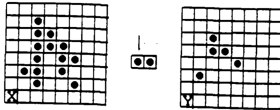
FIGURE 4b. EROSION
