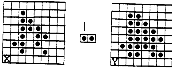
FIGURE 4a. DILATION
