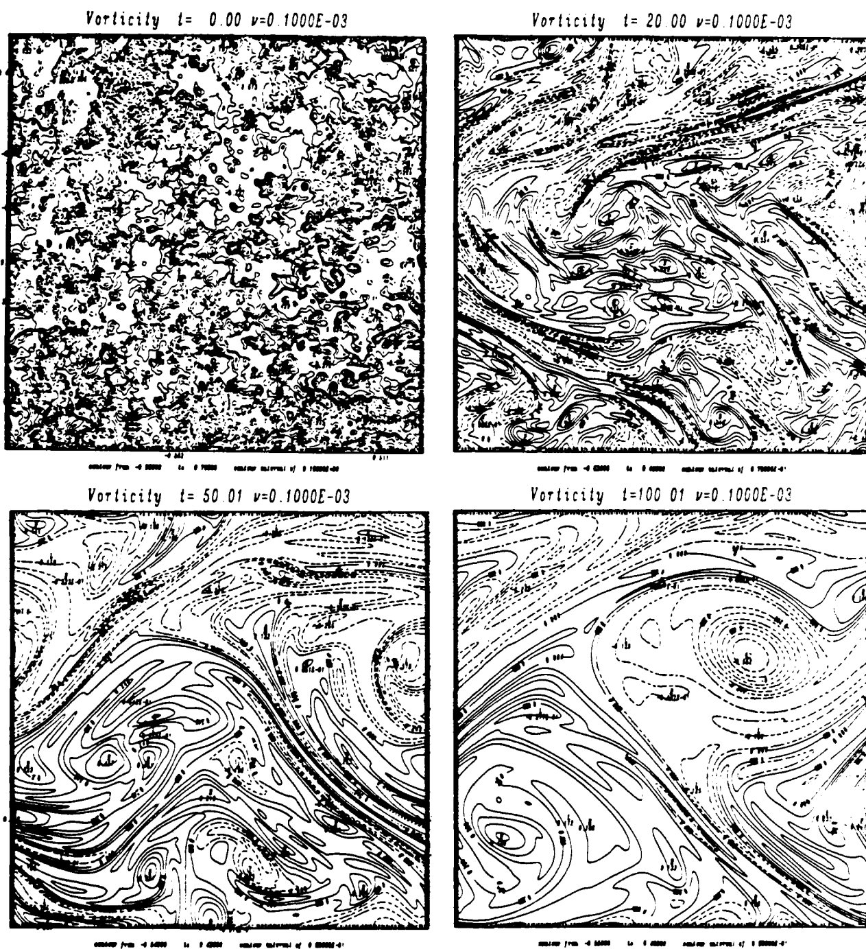
Figure 2 Contour plots of the vorticity for random initial data, \nu = 10^{-4} , N = 256 .
