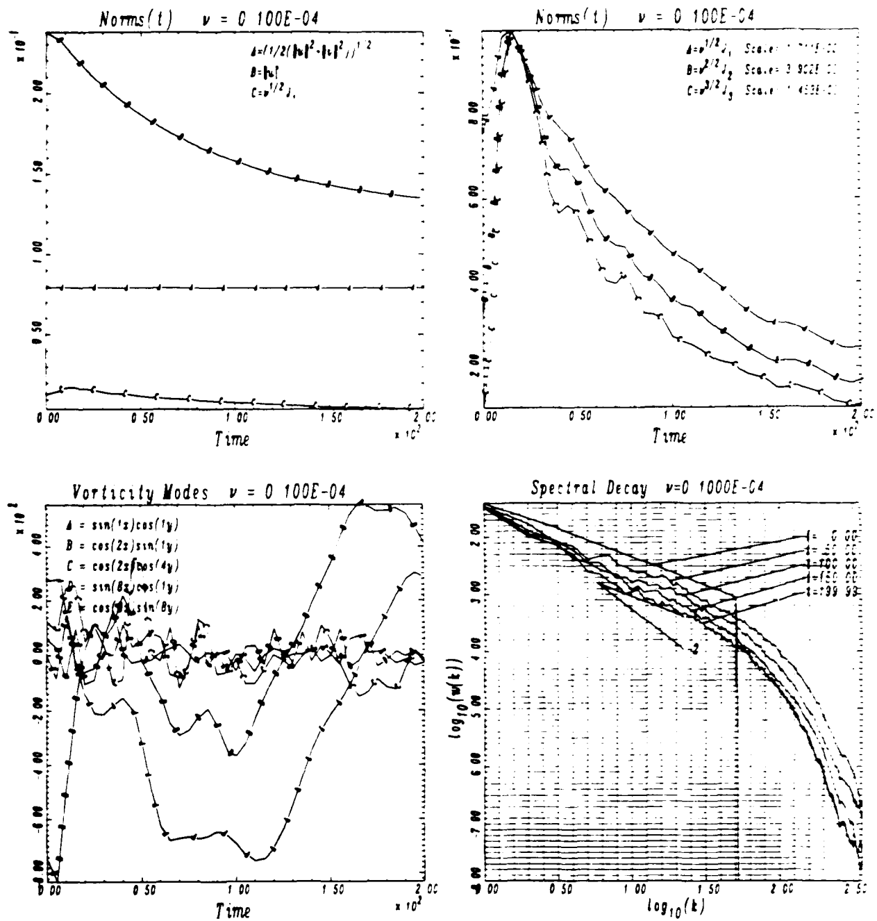
Figure 8 Results for random initial data, \nu = 10^{-5} , N = 512 .
