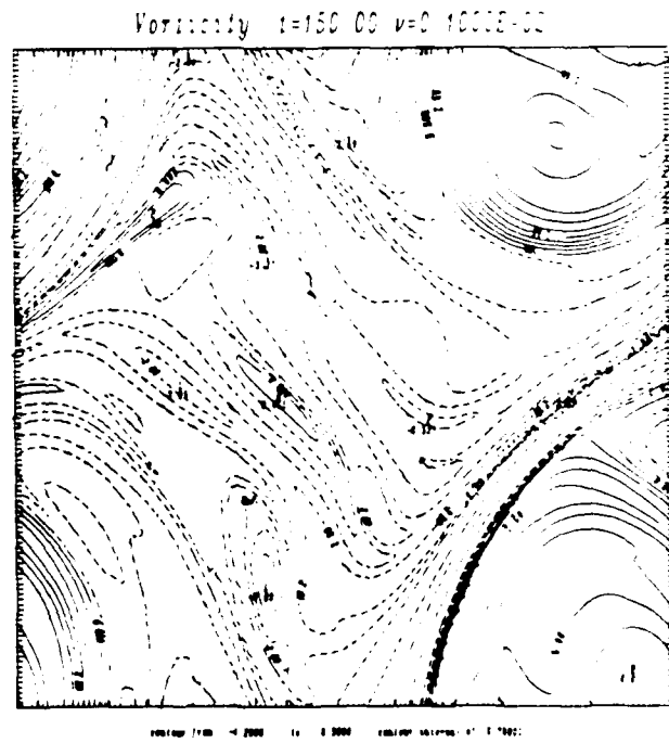
Figure 11 Random Forcing, |f|_\infty = 1 , \nu = 10^{-3} , N = 128 .
