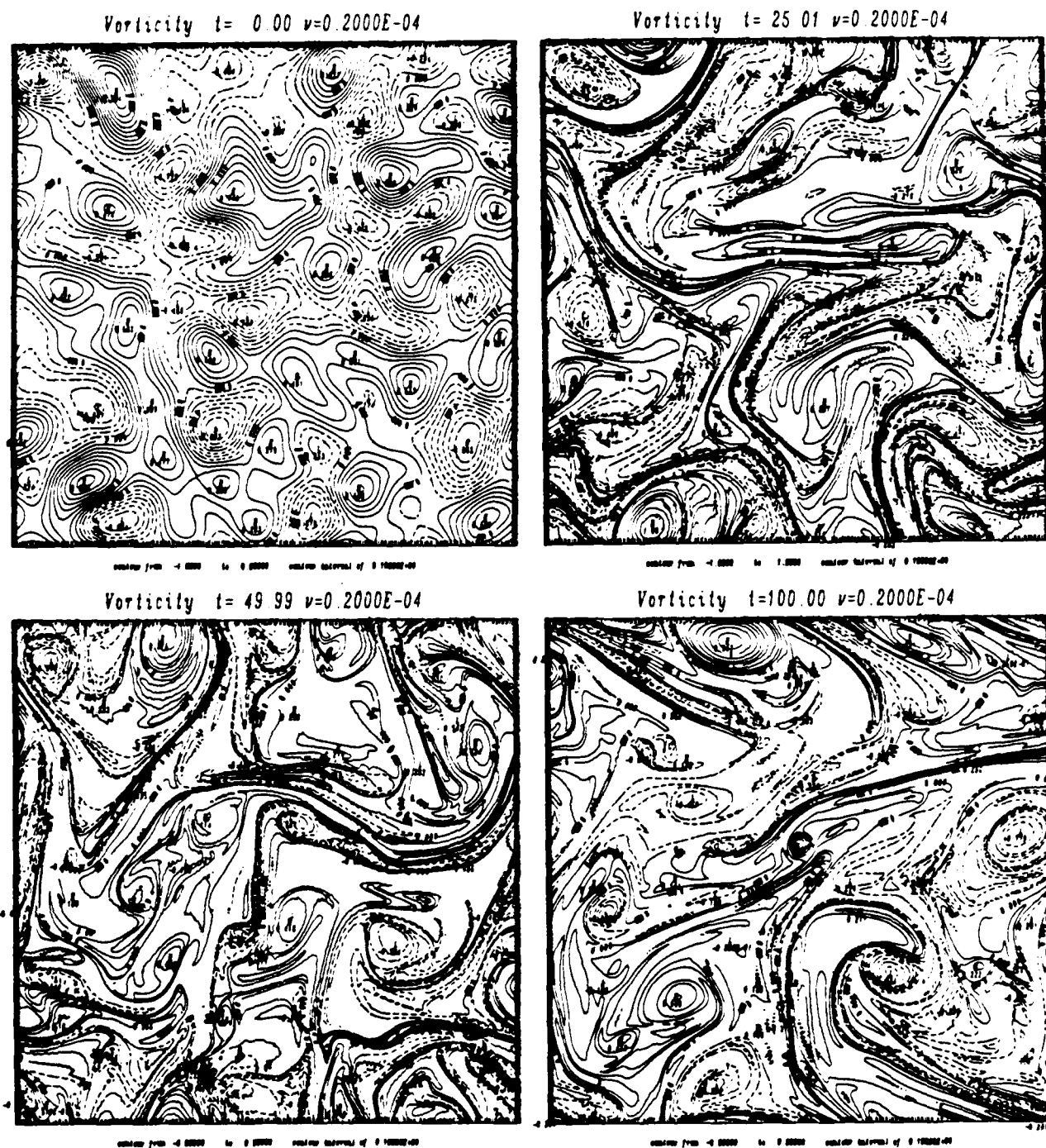
Figure 9 Contour plots of the vorticity for smooth random initial data, \nu = 2 \times 10^{-5} , N = 256 .
