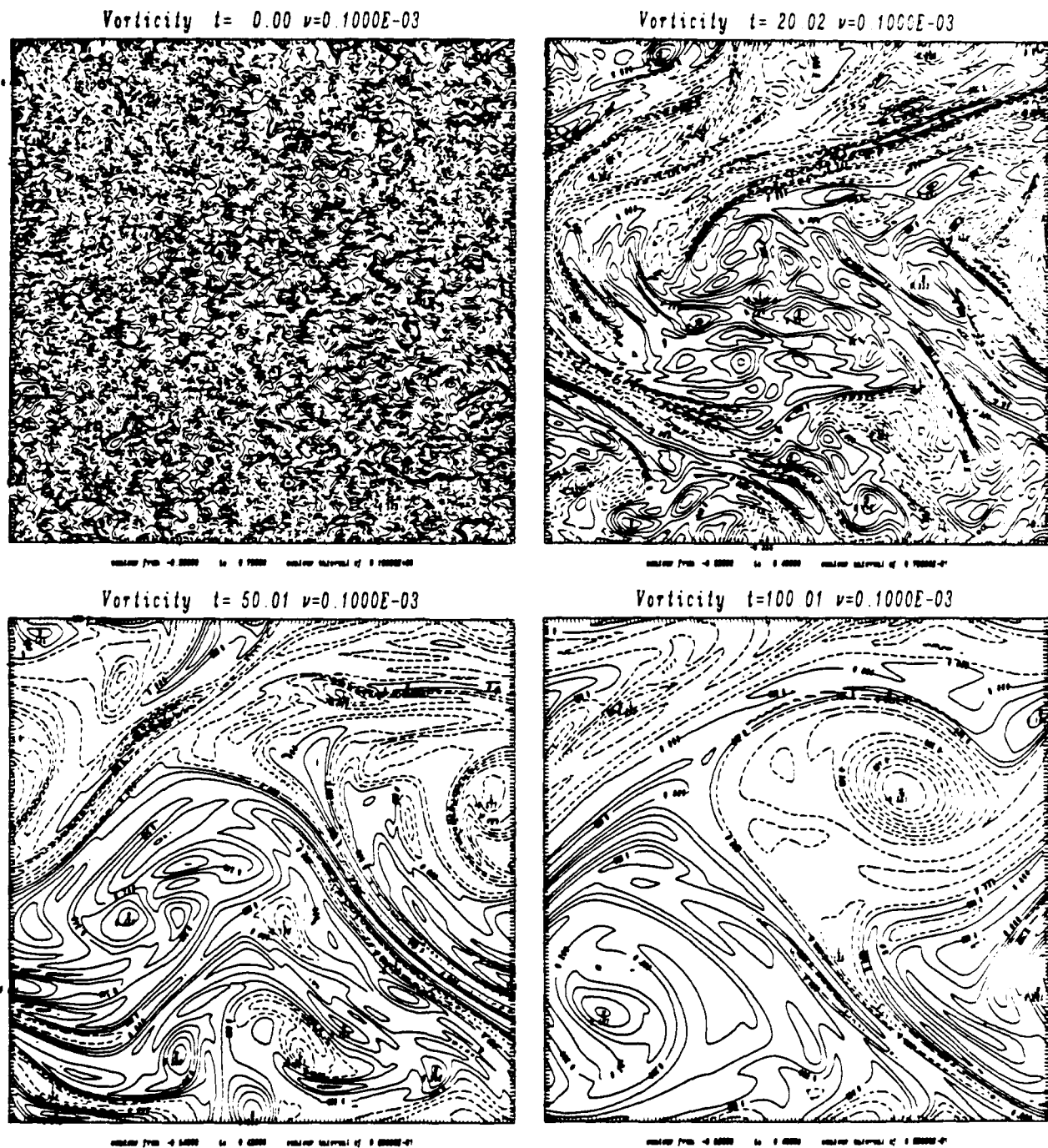
Figure 5 Contour plots of the vorticity for random initial data, \nu = 10^{-4} , N = 128 .
