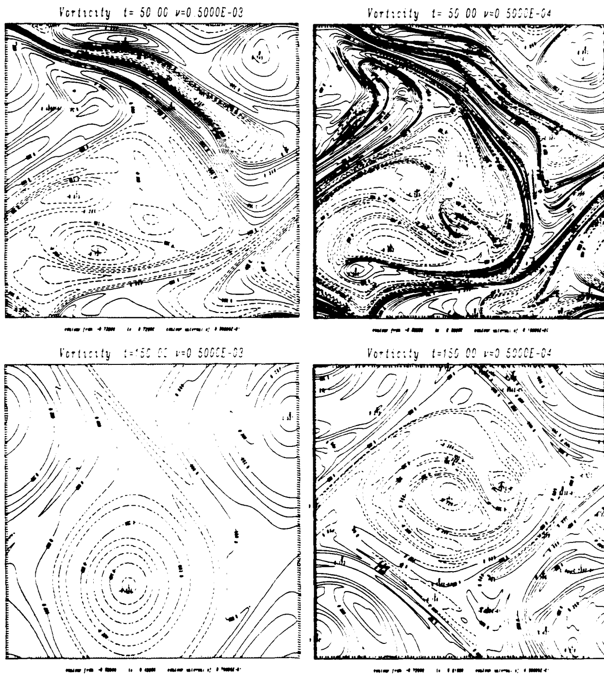
Figure 13 Contour plots of vorticity spectrum for random forcing. |f|_{\infty} = O(\nu) .
