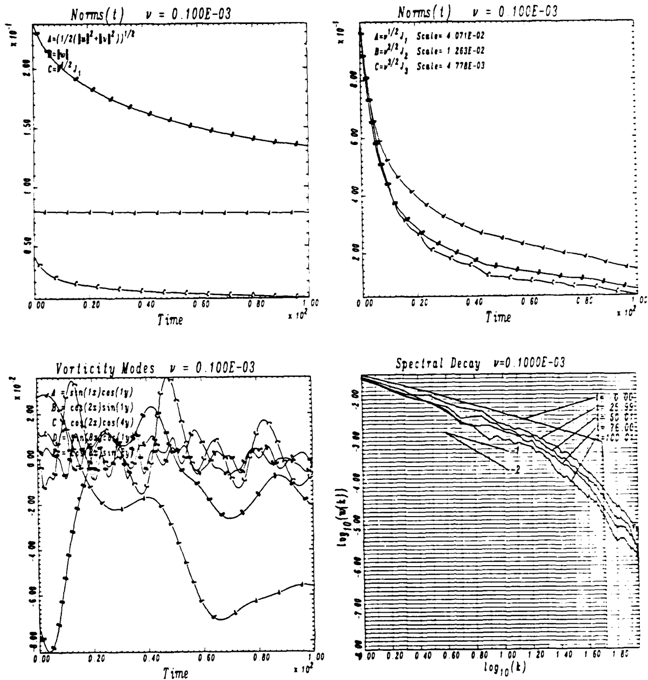
Figure 6 Results for random initial data, \nu = 10^{-4} , N = 128 .
