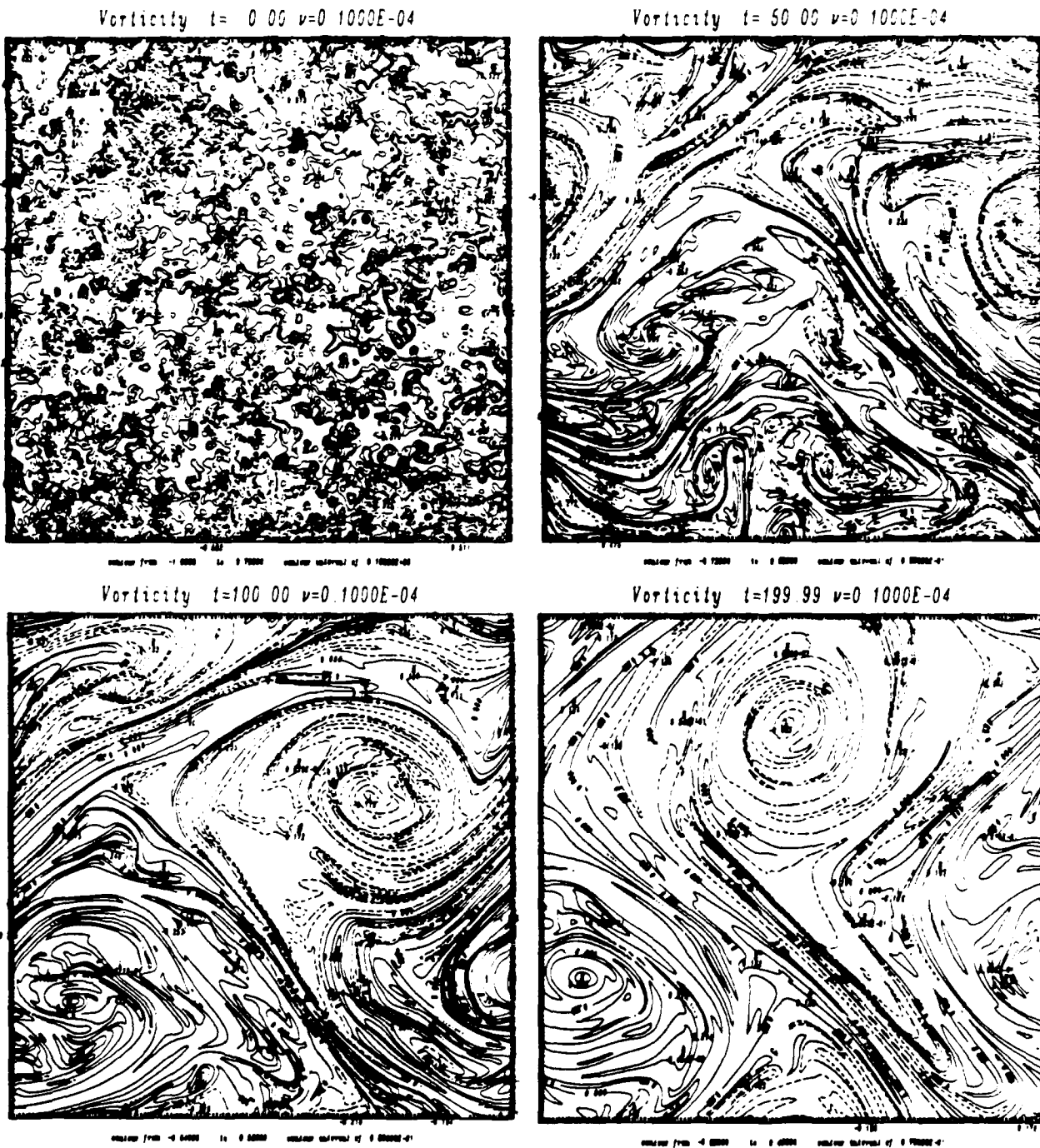
Figure 7 Contour plots of the vorticity for random initial data, \nu = 10^{-5} , N = 512 .
