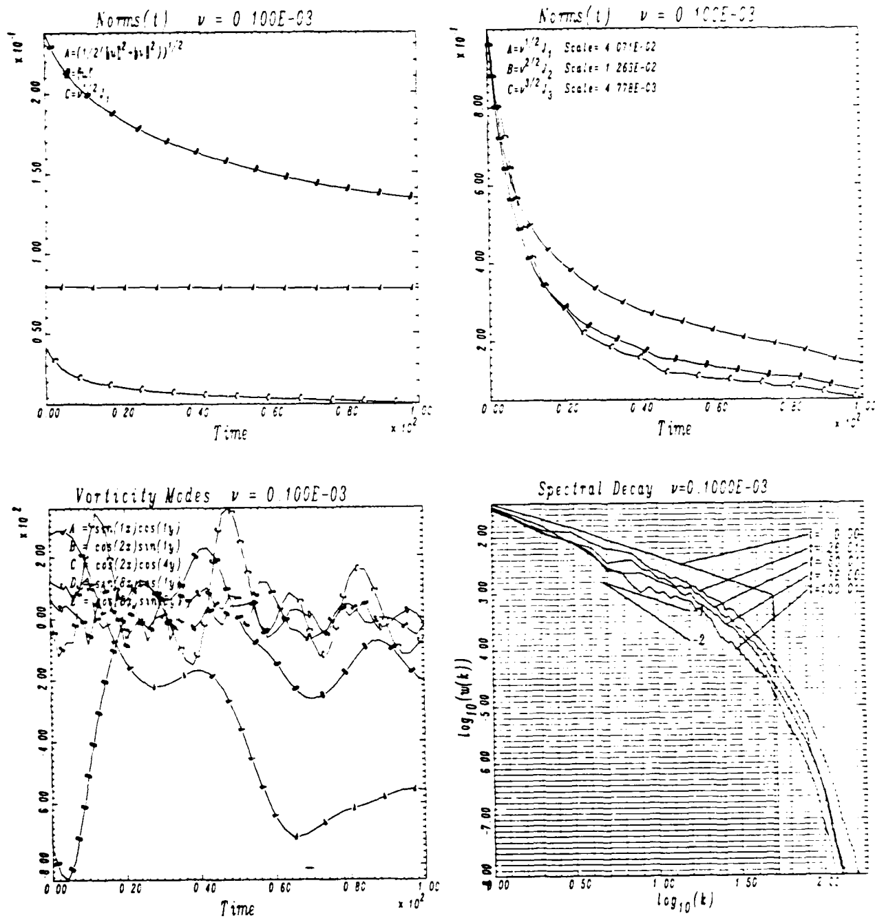
Figure 4 Results for random initial data. \nu = 10^{-4} . N = 256 .
