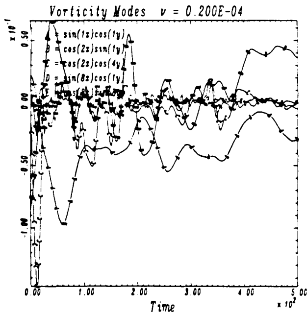
Figure 10 Results for smooth random initial data, \nu = 2 \times 10^{-5} , N = 256 .
