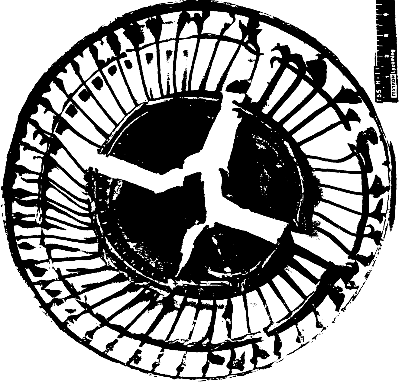
Figure 48 Exit Stator Ring, Front
