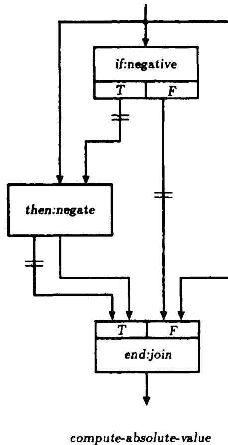
Figure 17. A plan diagram illustrating control flow and data flow. Compute-Absolute-Value computes the absolute value of a number.
