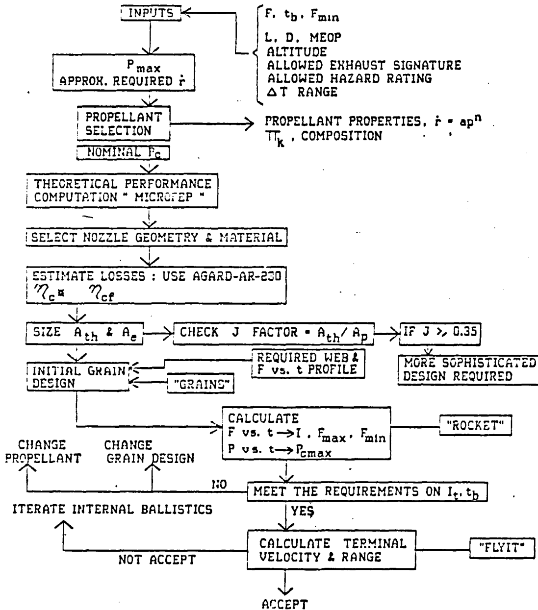
FIGURE 1. DESIGN PROCESS
