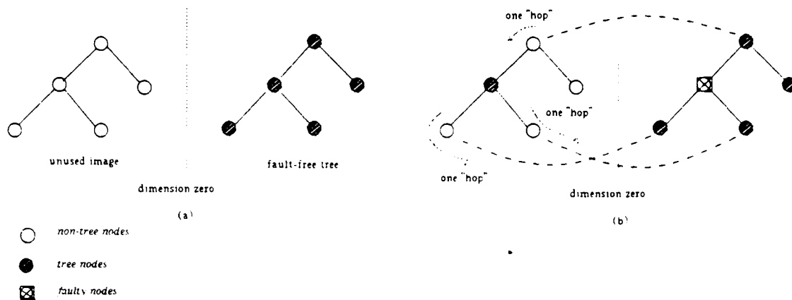
Figure 1 (a) a fault-free tree and its image (b) local remapping for a single fault
